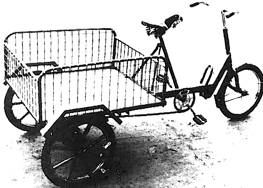
The design of the Oxtrike can be adapted to suit locally-available materials and manufacturing resources. Contrast the design of this vehicle, made in Kenya, with the U.K. version above.
