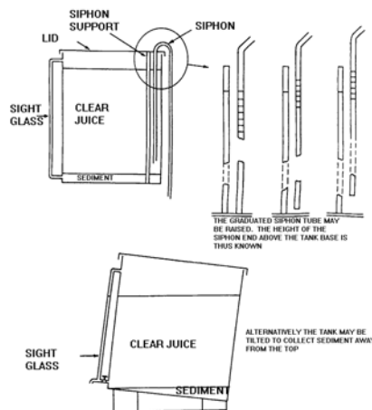
Figure 2: Florentine Flask
