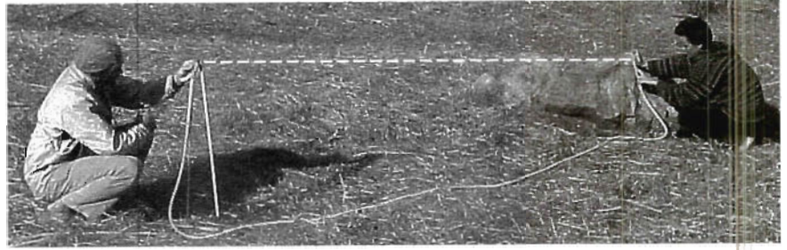
Checking levels with a water level. Person at right adjusts tube until water level is at her reference mark. Person at left measures from water level in tube to ground.
