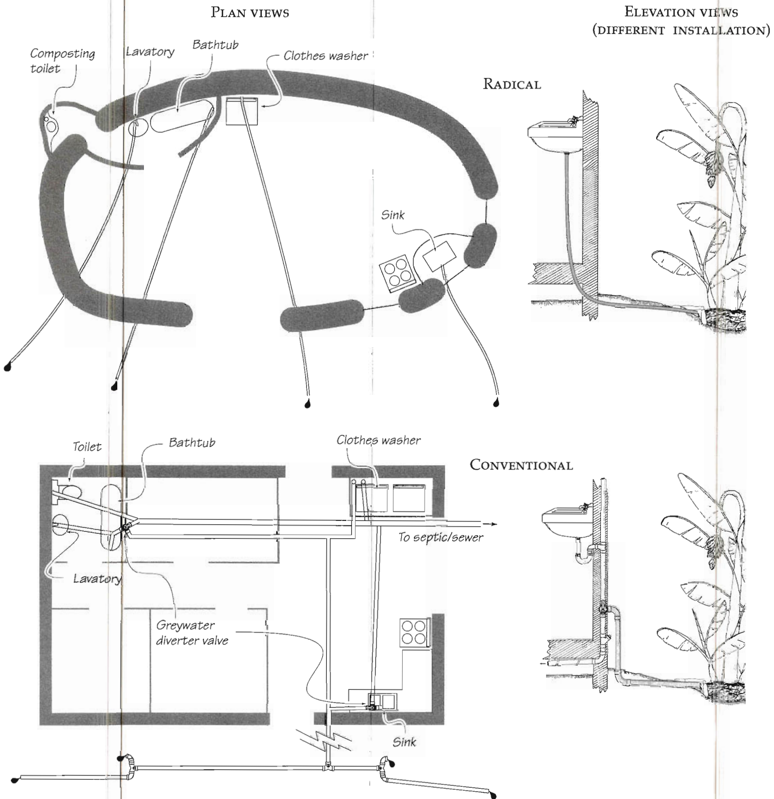
FIGURE 4.8: RADICAL VS. CONVENTIONAL PLUMBING
