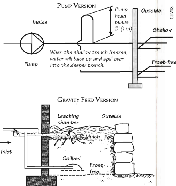
FIGURE C.1: AUTOMATIC SWITCHES FROM SHALLOW TO FROST-FREE ZONES/LEVELS
