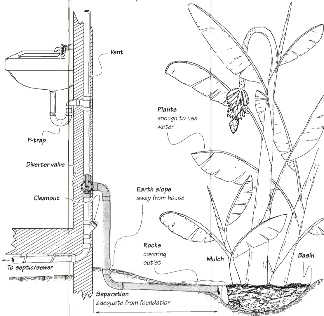
FIGURE 7.2: DRAIN TO MULCH BASIN
