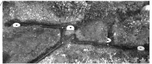
Four outlets with 1/8 each of bath/shower flow. These subsoil outlet chambers are way undersized. The owner plans to replace them with a continuous row of infiltrators 30' (10 m) long and 14" (35 cm) wide.
