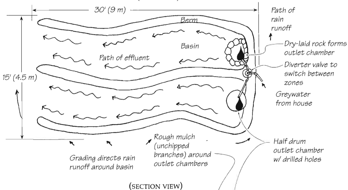
FIGURE 12.4: EVAPOTRANSPIRATION/INFILTRATION MULCH BASIN IN OREGON (PLAN VIEW)
