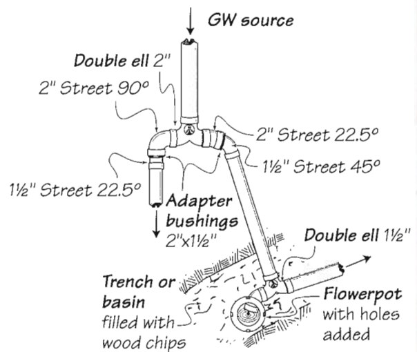
FIGURE 9.3: FLOWS SPLIT BY BRANCHED DRAIN NETWORKS (PLAN VIEW)
