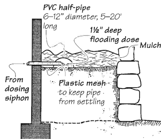
FIGURE 8.5: HALF-PIPE LEACHING CHAMBER
