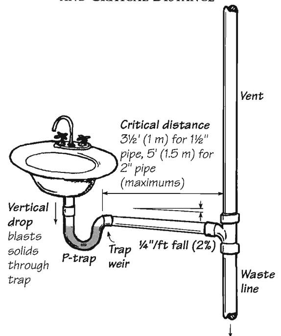
FIGURE 4.1: P-TRAP AND CRITICAL DISTANCE
