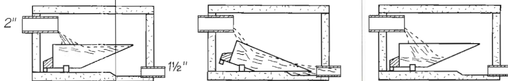
FIGURE 9.5: DIPPER DISTRIBUTION BOX DIPPING CYCLE
