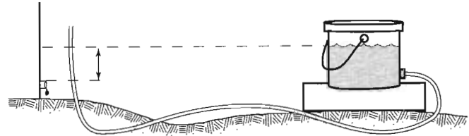
Reservoir water level. Can be used by one person—water level in bucket barely changes as tube moves up and down. You have to start over if you spill any water, though.
