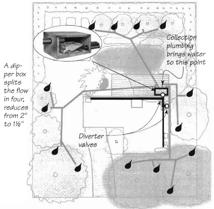
B: COMBINED FLOW SPLIT INITIALLY BY A DIPPER BOX, THEN BY FLOW SPLITTERS
