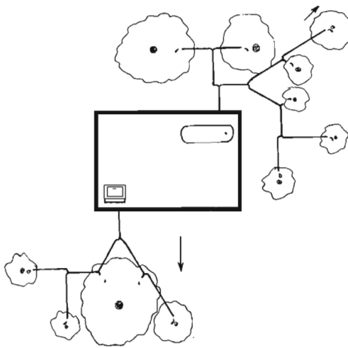
FIGURE 7.4: BRANCHED DRAIN NETWORKS (PLAN VIEW)
