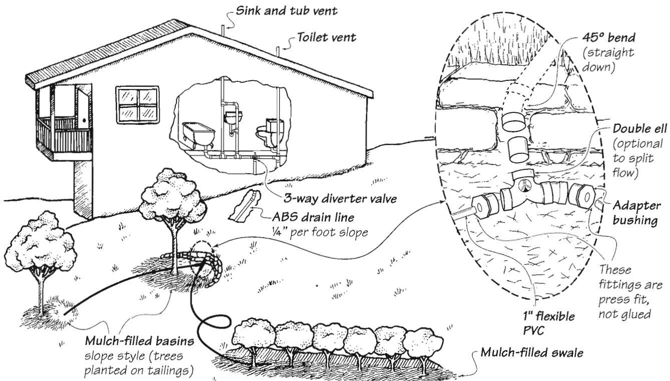
FIGURE 7.3: MOVABLE DRAIN
