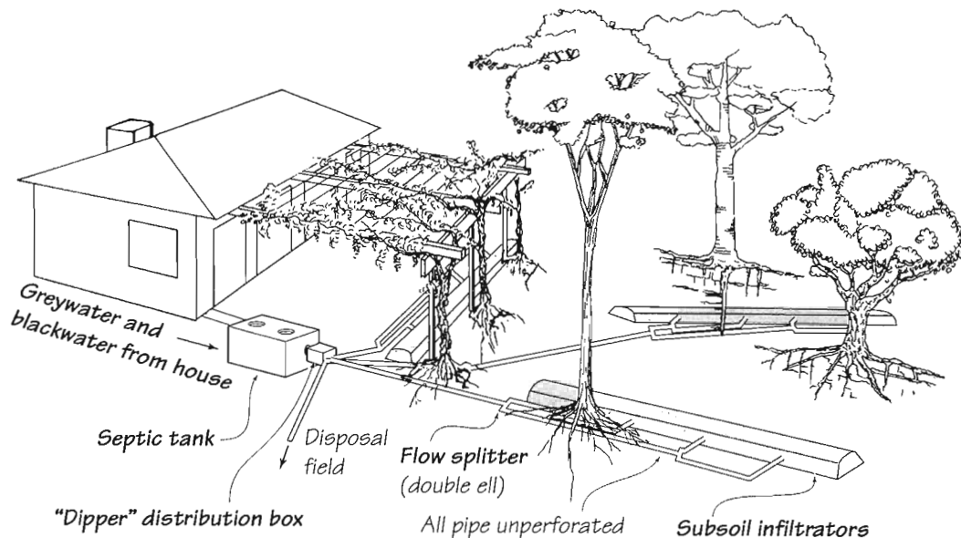
FIGURE 8.7: GREEN SEPTIC: TANK, FLOW SPLITTERS, AND INFILTRATORS (NUTRIENT AND WATER REUSE FROM A NEARLY CONVENTIONAL SEPTIC SYSTEM)
