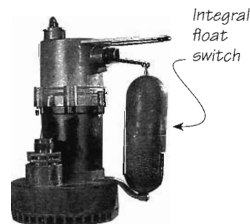
One of the better throw-away pumps that require a filter (a $200 Little Giant Model 5.5-ASP pictured).
