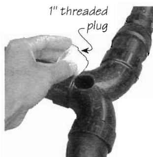
A double ell retrofitted with inspection access. The access is sealed with a threaded plug. 59
