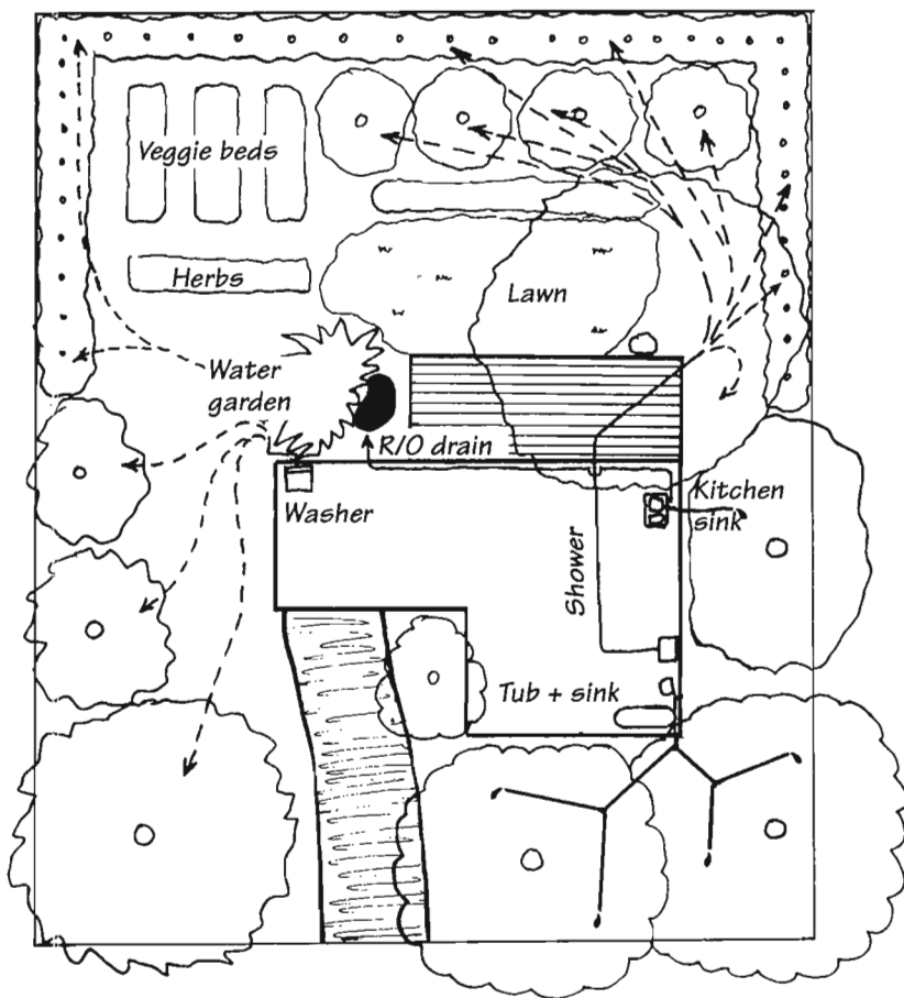
FIGURE 5.1: MATCHING GREYwater SOURCES TO IRRIGATION NEEDS
