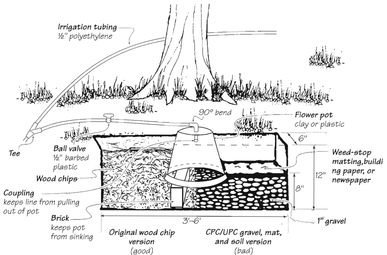
FIGURE 8.3: MINI-LEACHFIELD
