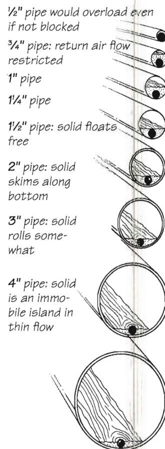
FIGURE 4.7: EFFECTS OF PIPE SIZE ON FLOW
