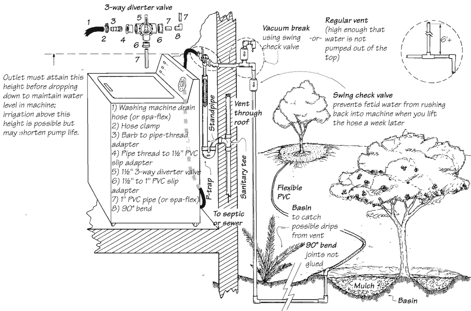
FIGURE 7.6: DRUMLESS LAUNDRY
