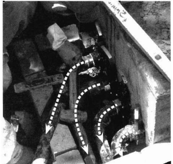
Dipper distribution box with a brick enclosure around individually valved outlets.
