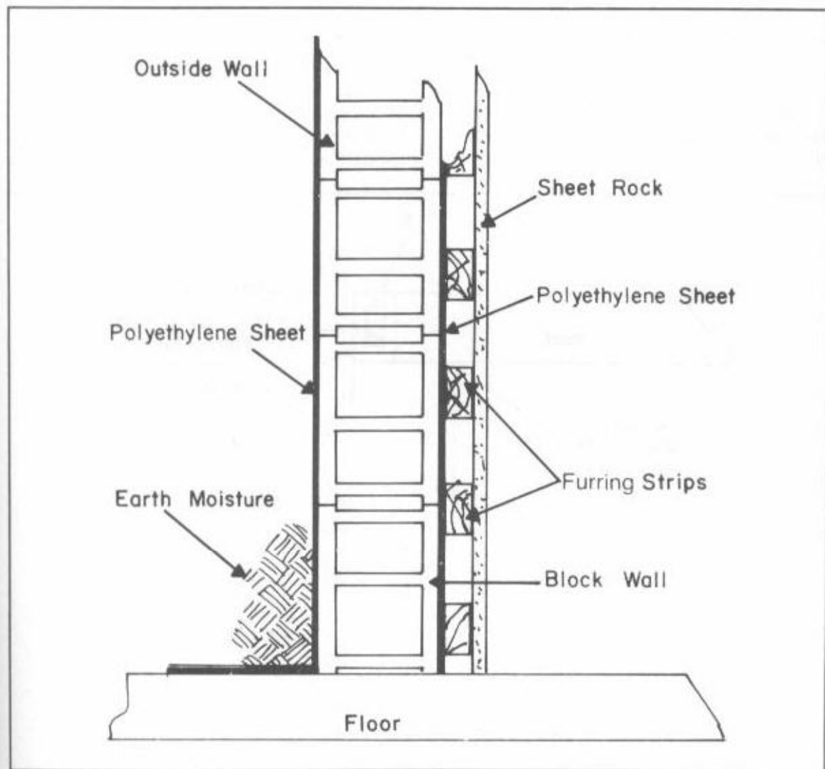
Fig. 12-7. Typical section of exterior wall.
