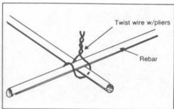
Fig. 9-19. Tie rebar together with stove pipe wire.
