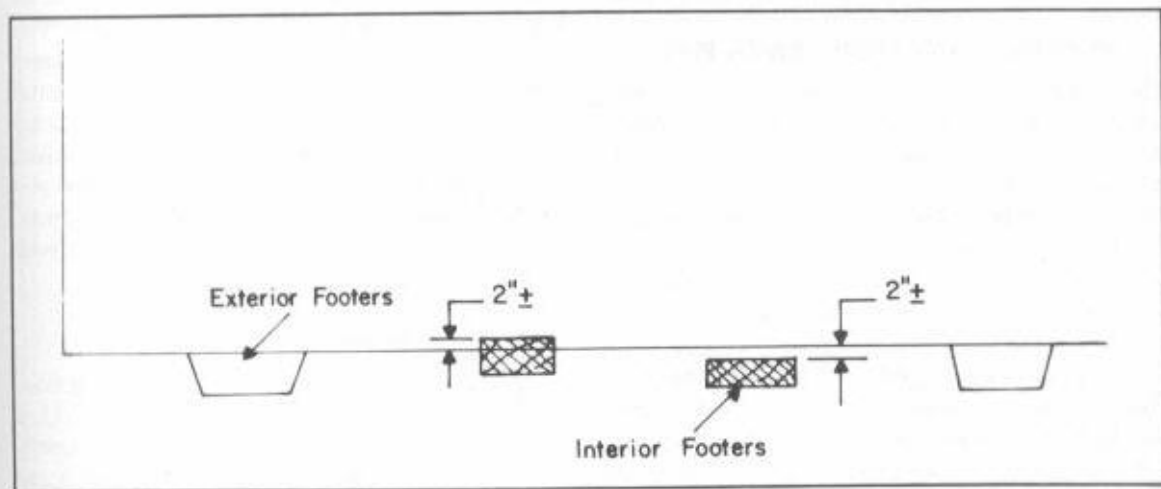
Fig. 7-7. Interior and exterior footers need not be exactly level with each other.
