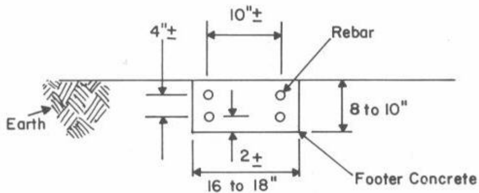
Fig. 7-1. Typical placement of rebar in normal footers.
