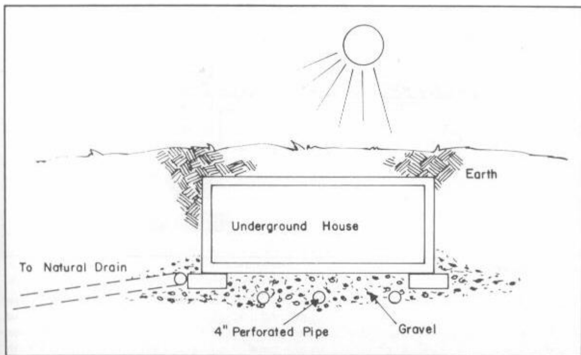
Fig. 11-4. Drain field under floor.
