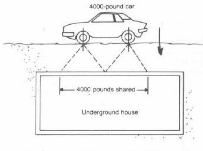
Fig. 13-12. The weight of a vehicle will displace the earth as the wheel presses downward.
