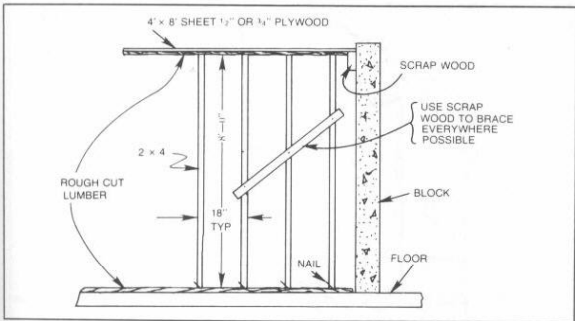
Fig. 9-3. A typical arrangement for storing materials.
