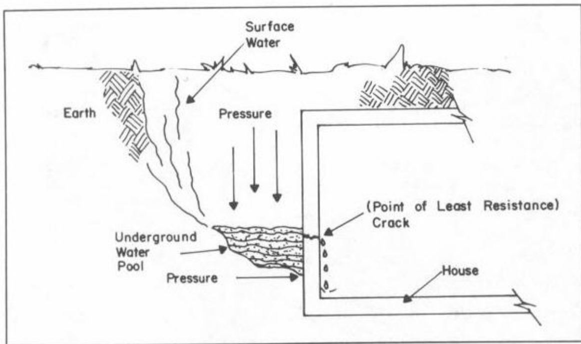
Fig. 2-2. Pockets of water cause pressure below.
