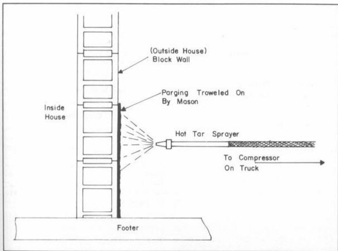
Fig. 11-2. Hot tar is sprayed.
