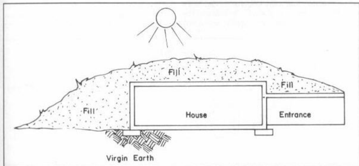
Fig. 2-5. Backfilling and extra earth get to be cost prohibitive when building underground above natural grade.
