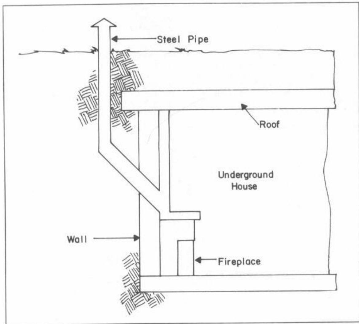
Fig. 9-26. Preferred way to place chimney.
