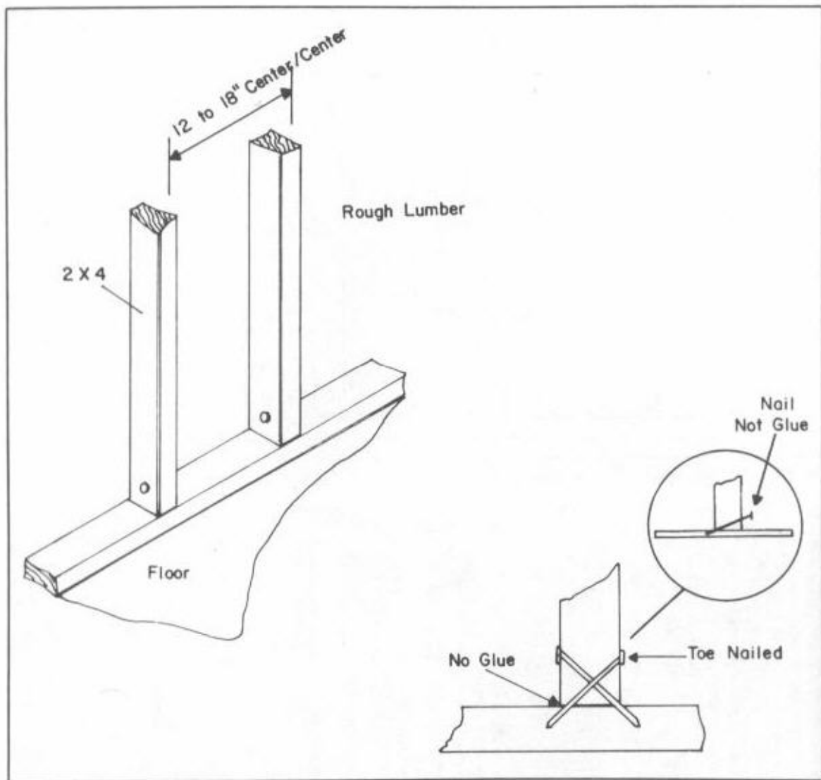
Fig. 9-5. Don't glue wood together onto concrete floor.
