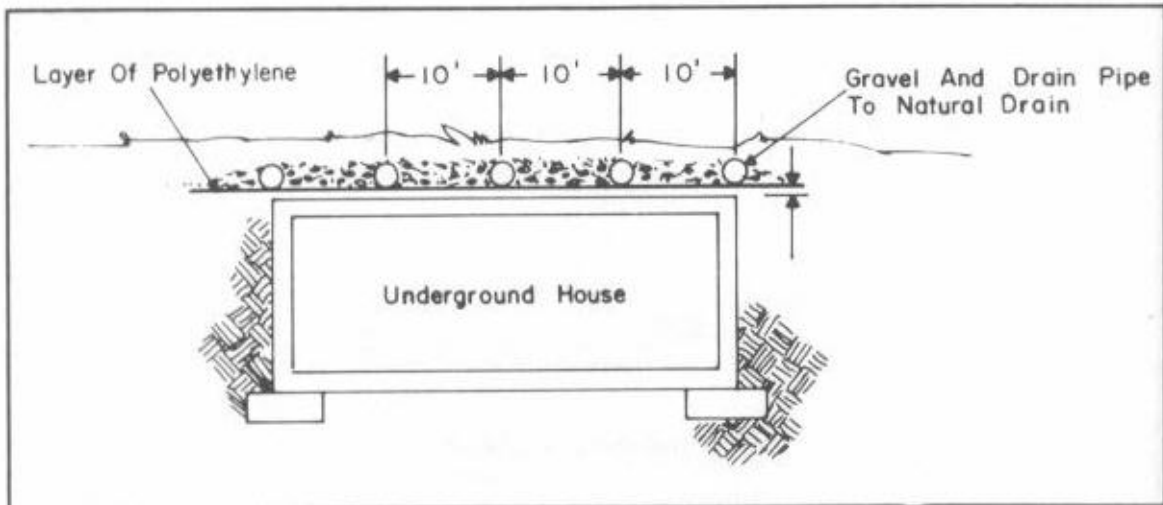
Fig. 11-5. Drain field over roof.
