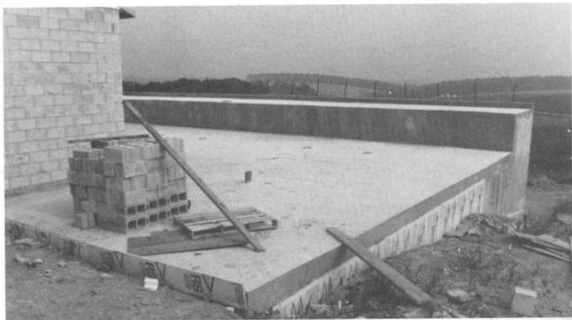
Fig. 10-11. Two-story underground garage.
