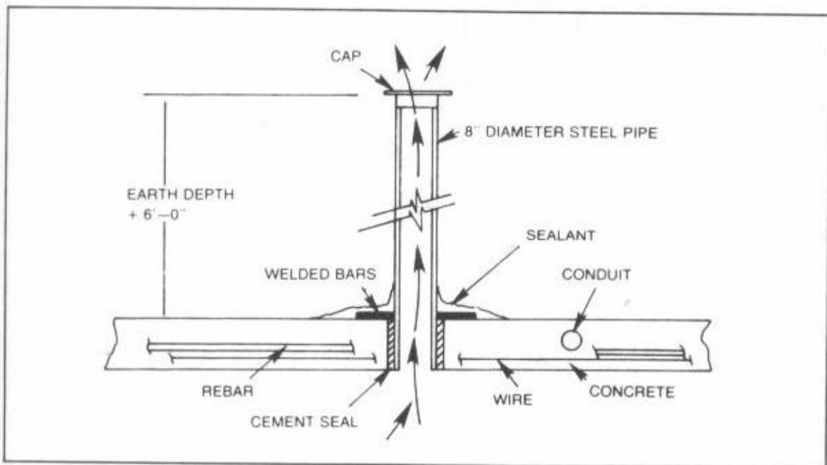
Fig. 9-25. Notice the electrical conduit in place in the concrete.
