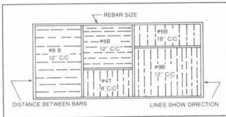
Fig. 9-16. Size and location of rebar.
