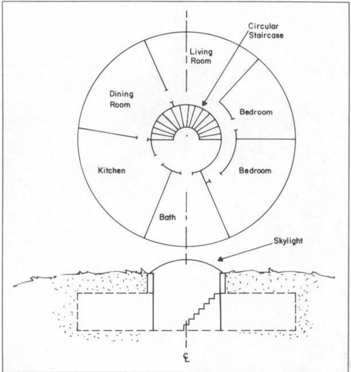
Fig. 1-6. Sketch of the circular design.
