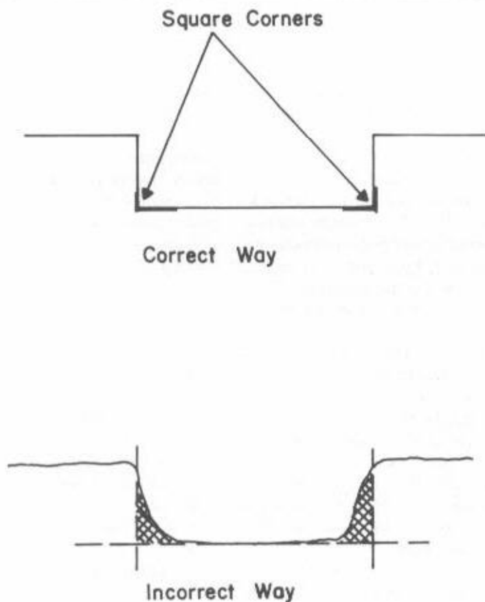
Fig. 7-2. Always keep corners of footers square and clean.
