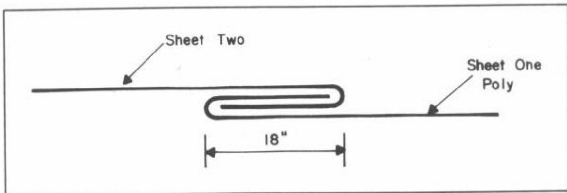
Fig. 12-8. Lopping method of plastic sheets; no glue is necessary.
