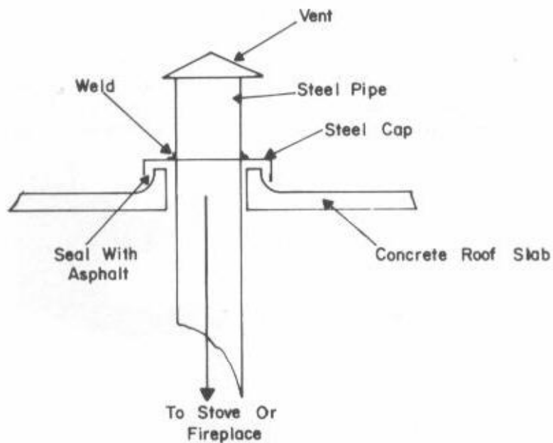
Fig. 9-27. Build a column of concrete as the roof is being poured at least 6 inches high.
