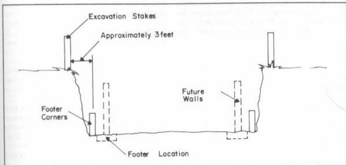
Fig. 6-12. Don't confuse the difficult points of measurement.
