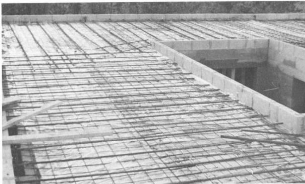
Fig. 9-17. Wire mesh gives real strength to the roof structure.
