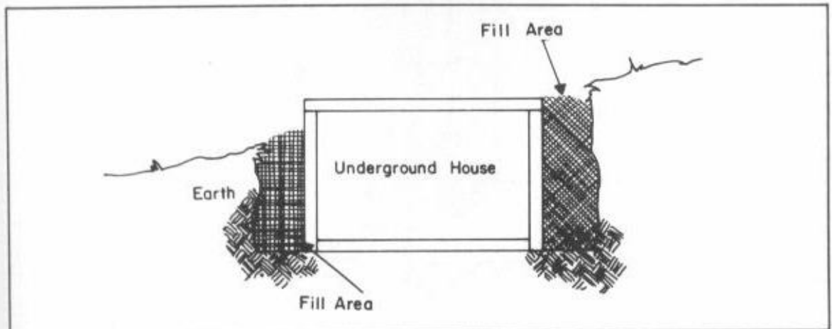
Fig. 13-5. Backfill areas before the roof scaffolding is placed. You need to walk on this space.
