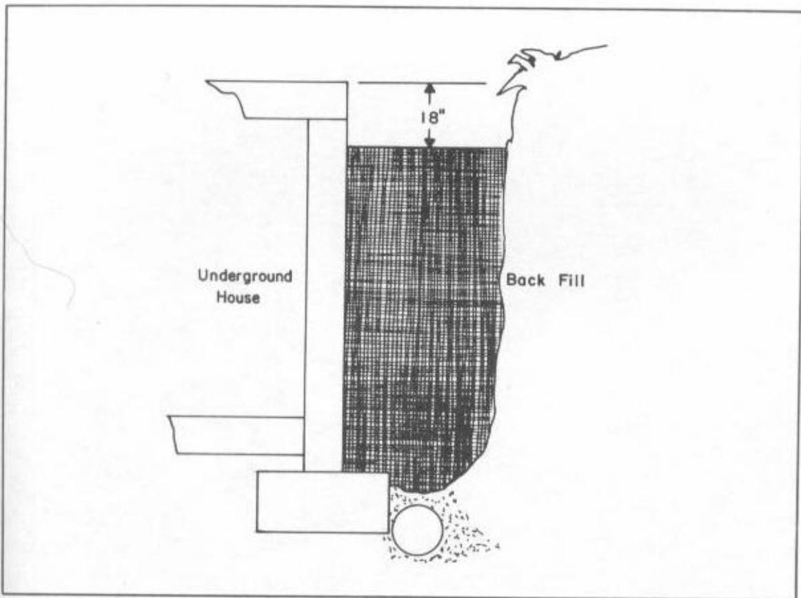
Fig. 13-8. The 18 inches of space will give you room to seal the roof plastic to the side plastic.
