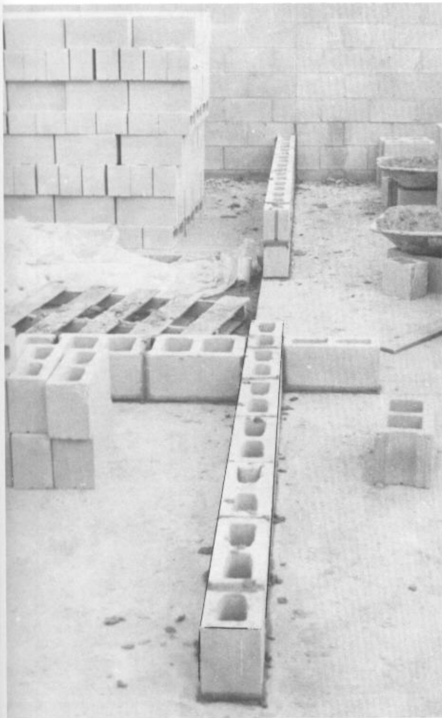
Fig. 8-3. First stages of interior walls.
