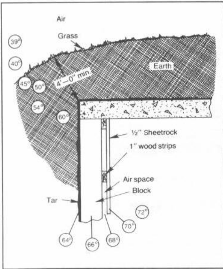
Fig. 12-3. Notice the gradual penetration of temperatures.
