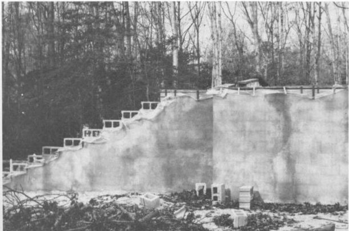
Fig. 10-3. Another view of the same structure.
