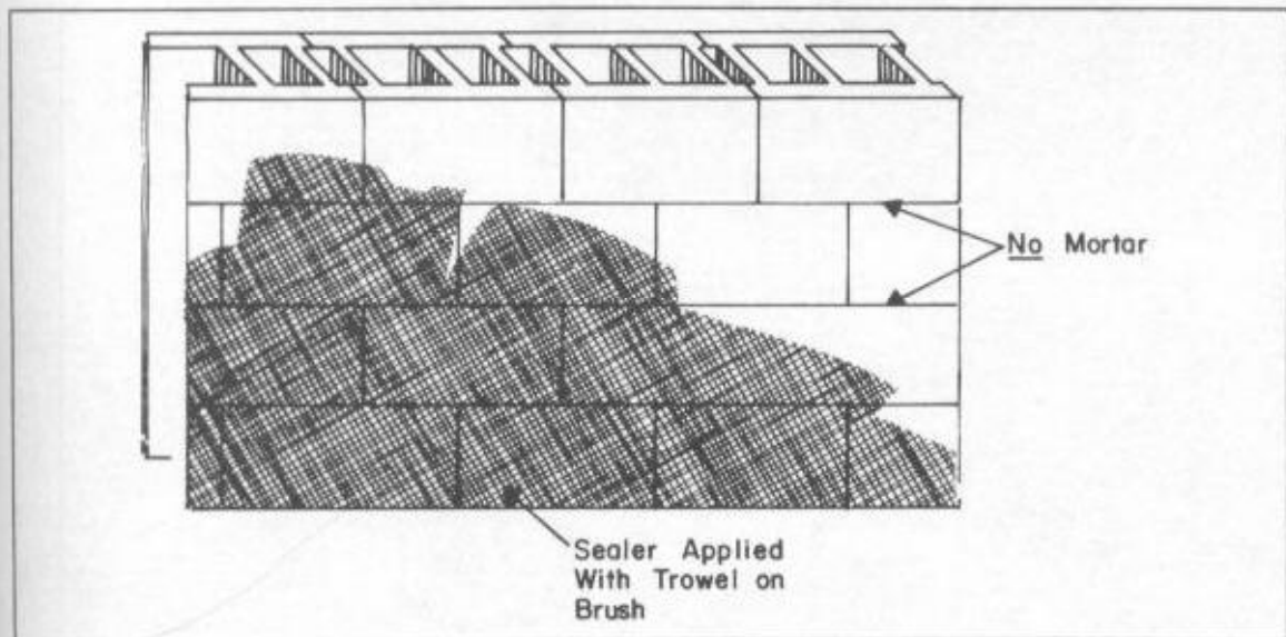
Fig. 10-4. Sealer-adhesive holds block together without mortar.
