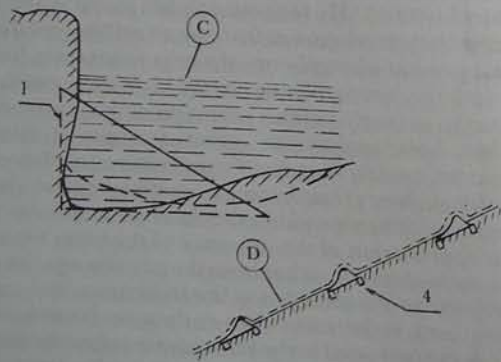
(C) shows details of braking element. (D) shows another type of braking element (4) for mountain streams, to slow down the speed of flow, thereby reducing the amount of material carried away from the bed and banks. (Taken from Austrian patent 11 34 87.)
