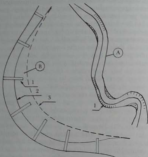
A scheme for flood control. (A) shows a watercourse to be regulated. A breaking barrier has been built into the river bed at (1). (B) shows how the axis of flow will be moved from (2) to (3) after the barrier has been working for some time.
