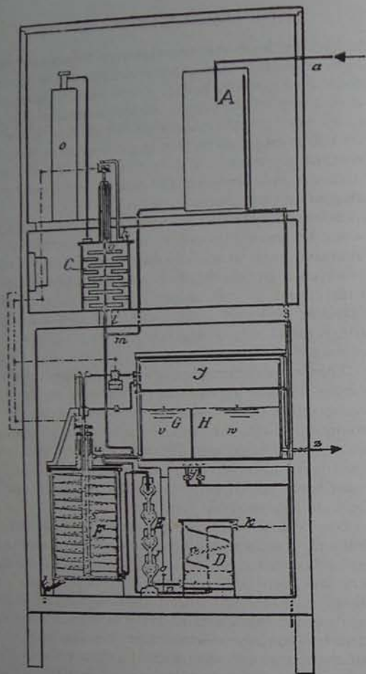
An earlier type of apparatus for the production of 'living water'. Sterilized water from container (A) is mixed drop by drop with the salt solution from (C). The mixture then passes to (D) where it sprays out from the perforated pipe 'n', while carbon dioxide is being introduced via pipe 'k'. Water falls in droplets to the bottom of (D) while absorbing carbon dioxide, and is led to (E) where it is forced into a meandering motion onto (F) where it passes over gold and silver filaments, to finally gather and cool in the silver lined container (H), until it slowly reaches +4°C.
