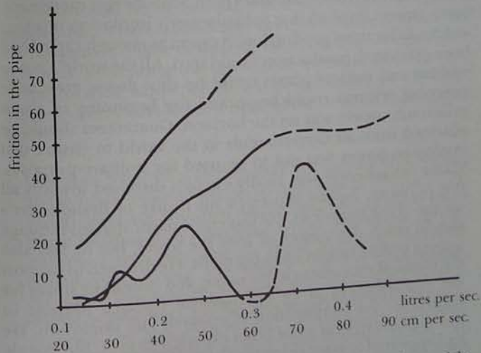
Graph of the tests in Stuttgart. The upper curve shows friction in a straight glass pipe; the middle curve, in a straight copper pipe; and the bottom curve, the spiral-wound copper pipe. The solid lines show measured values, and the broken lines the estimated values.
