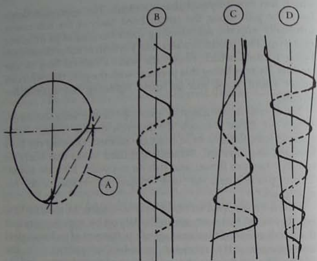
Pipes for liquids and gas. This pipe was also to be used in the 'Trout turbine'. Its cross section is shown in (A). (B), (C) and (D) are different designs of spiral pipe systems, showing the pipe to be wound around cylindrical and conical objects. (From Austrian patent no. 19 66 80).
