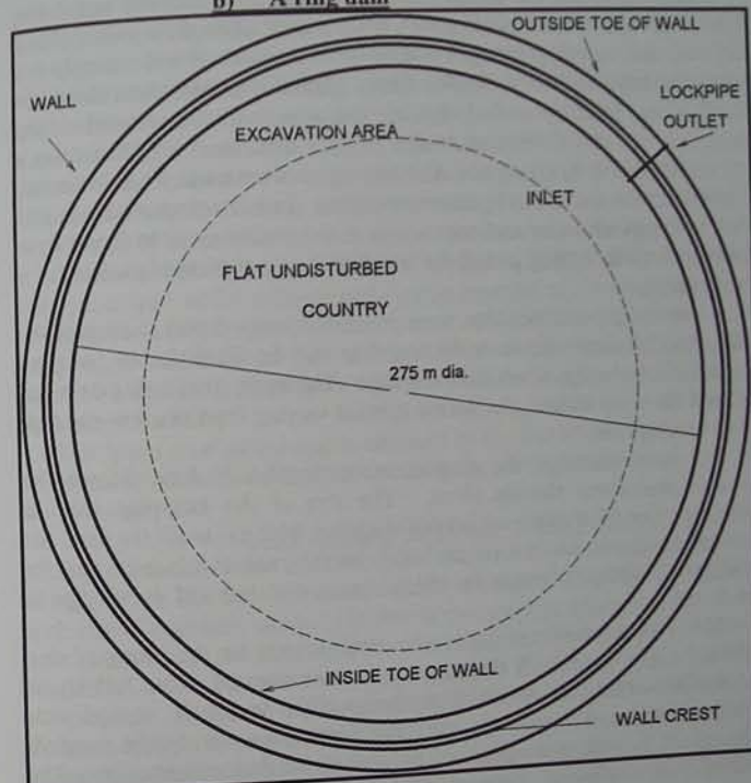
Figure 17. Plan of ring dam.
