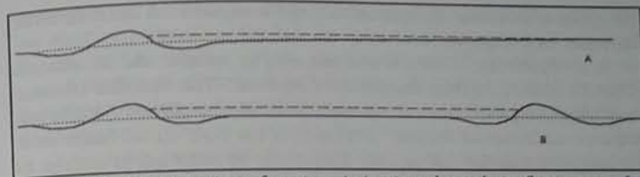
Figure 37 Cross section of contour irrigation channels in flat country for Flood-flo irrigation.
