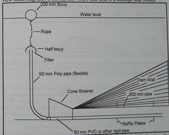
Figure 28. A cross section of the inside toe of the wall showing the Flota-filta components.
