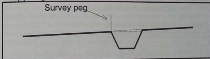
Figure 34. Preferred channel cross section for hillside (Keyline Pattern) irrigation. Grade is 1 in 300; with a range between 1 in 250 and 1 in 500. Note the channel is dug beside the surveyed peg on the uphill side.
