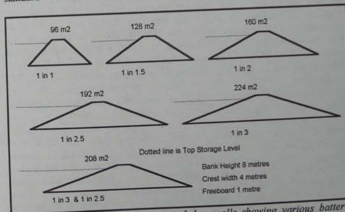
Figure 22. Cross sectional areas of dam walls showing various batter slopes.
