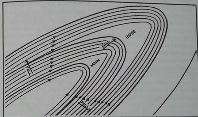
Figure 10. Showing the automatic development of a pattern that will drift the water toward the centre of the ridge. Ridge cultivation is parallel upwards from any guide line. The small arrows show the direction of slope of the furrows.
