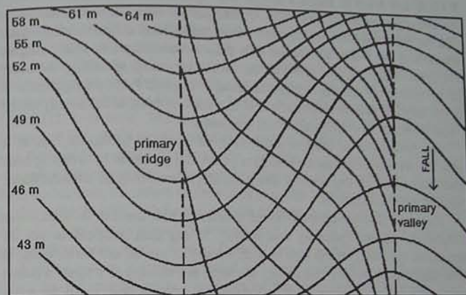
Figure 7. The flow paths of run off water from the ridges to the valleys are flat S curves.
