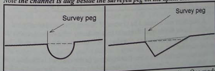
Figure 35. Alternative cross sections with similar flow capacity. One made with a rotary channel digger, the other with angled blade, which forms a flat V channel. Both are excavated 600 mm (2 feet deep). The channel width at the water line of semicircular section is 1.2 m (4 feet) whereas the V channel is 2 m (6 feet 8 inches). The wider channel is impractical to straddle.
