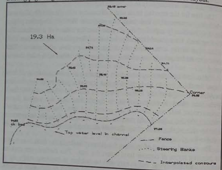
Figure 39. A steering bank layout designed from several contours surveyed through the area. Steering banks cross contours at right angles, which is the maximum slope. Consequently there is very little "cross fall" (sideways slope) in the bays. Land planing, such as laser levelling, is not normally required.
