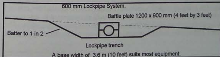
Figure 24. Showing side battering of lockpipe trench.
