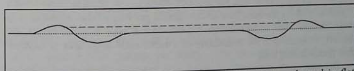
Figure 36. Cross section of a contour (no fall) irrigation channel in flat country for Flood-flo irrigation.
