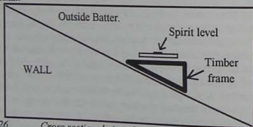
Figure 26. Cross sectional view showing the use of a large, right-angle triangle frame and spirit level to check the outside batter of the wall.
