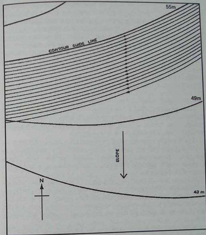
Figure 14. The contour diagram shows the selection of the contour guide line - the 55m contour - for a pattern of cultivation which will drift water toward the steeper western side of this area. As the contours in this diagram indicate a ridge shape it is normally better not to drift the water to the steeper side of the area as this will be toward the sides of the adjacent valley.
