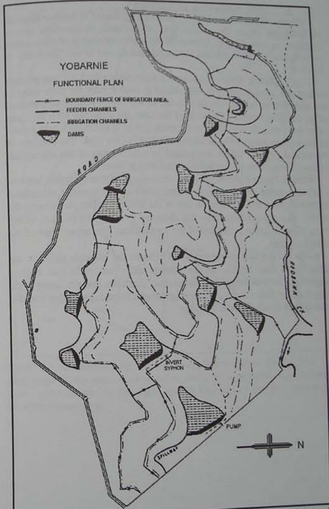
Figure 4. The flow through the spillway of the creek dam fills six other dams below the creek diversion channel. Pumping is only from the lowest dam on the bottom boundary.
