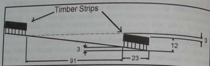
Figure 30. Cross section of timber strip spacing used in the text. Ground slope is 1 in 7.5.
