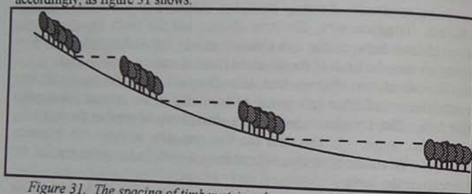
Figure 31. The spacing of timber strips changes as the slope varies.
