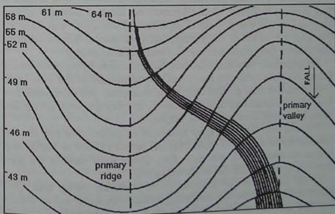
Figure 8. Depicting one flow path to illustrate the increasing volume of flow from the ridge to the valley.
