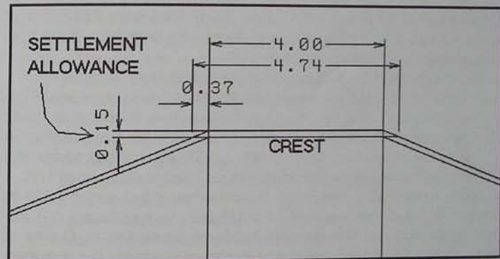
Figure 23. Upper section of an 8 metre wall showing the settlement allowance dimensions.
