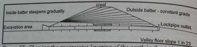
Figure 27. Showing the progressive layering of the earth in the wall.
