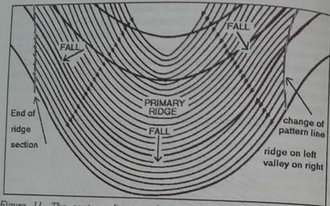
Figure 11. The contour diagram show a primary ridge with Keyline cultivation designed to drift the first flow of run off towards the centre of the ridge. Note the end of the ridge pattern cultivation.
