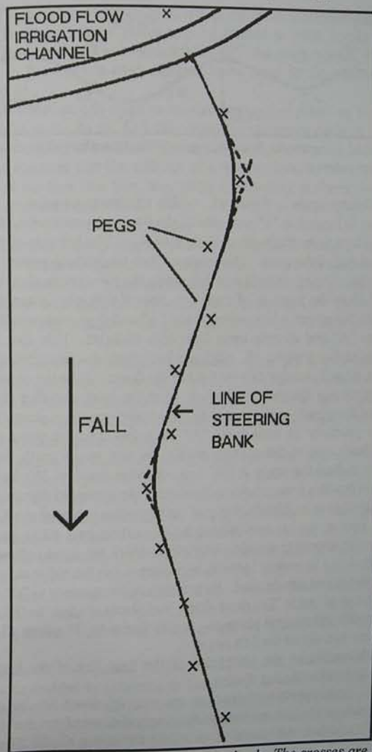
Figure 40. Pegging the line for a steering bank. The crosses are the points of maximum fall located by the level. The curved line represents the steering bank. The three straights show the formalised line of the steering bank if a fence is to be located along it.
