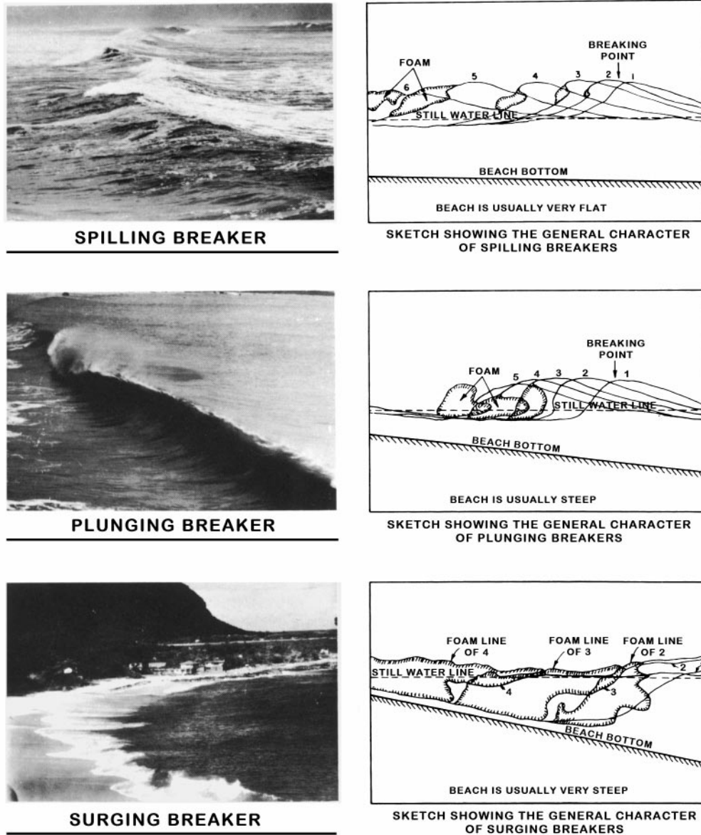
Figure 3317. The three types of breakers. Courtesy of Robert L. Wiegell, Council on Wave Research, University of California.
