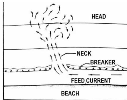
IDEALIZED RIP CURRENT
