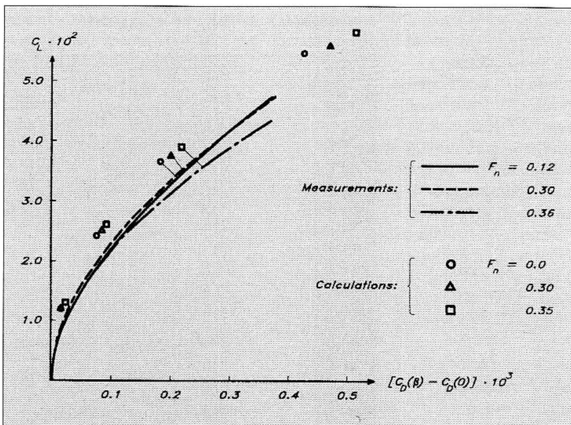
Fig 16.7 Calculated and measured lift-drag polars on Antiope
