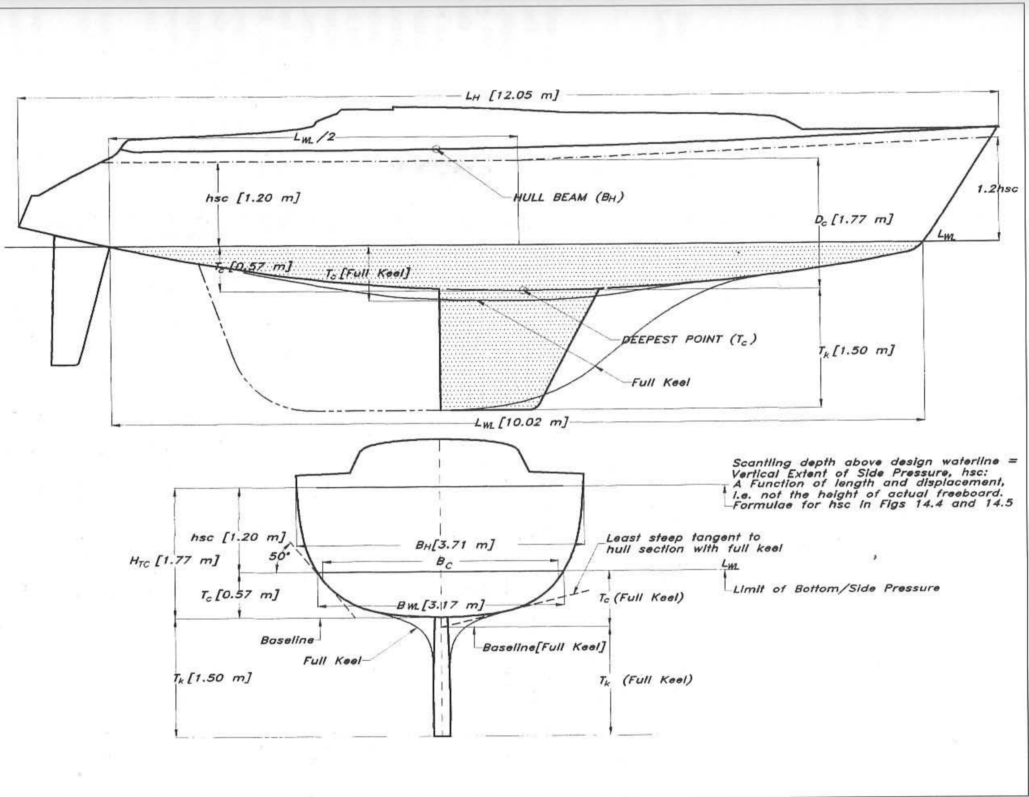
Fig 14.3 ISO hull definitions
