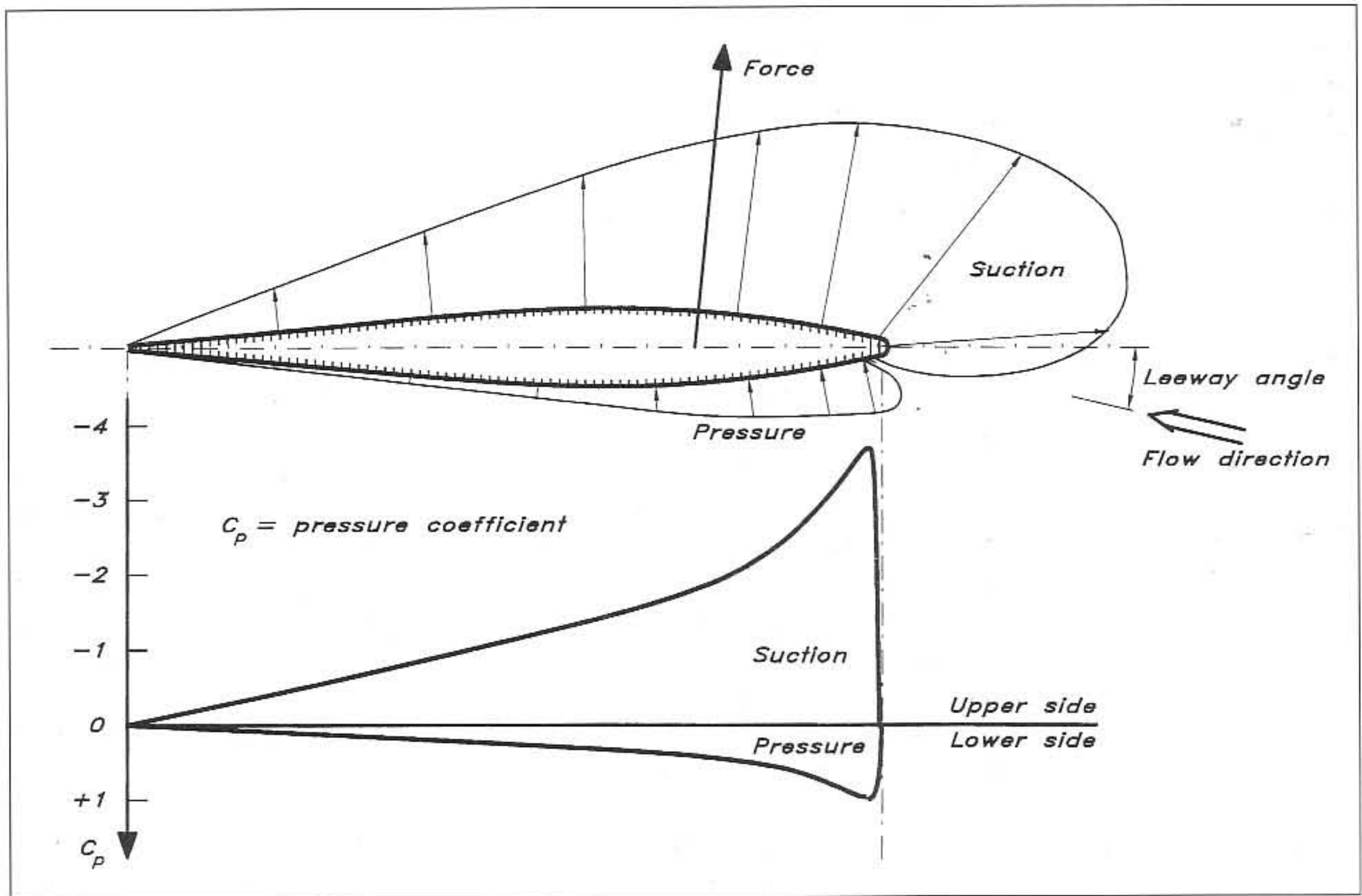
Fig 6.2 Pressure distribution around a wing section
