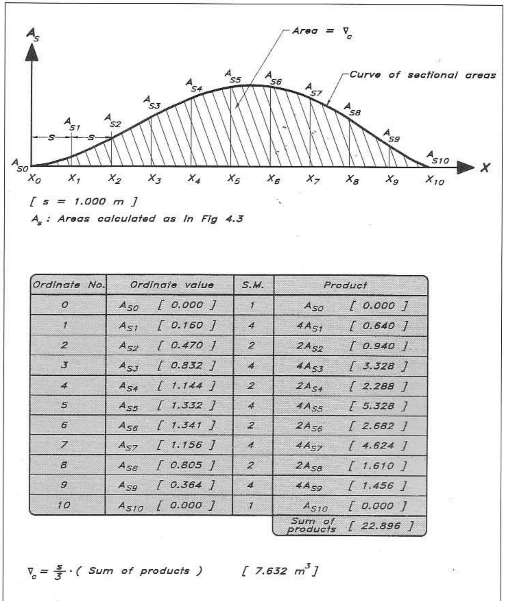
Fig 4.4 Calculation of the volume displacement
