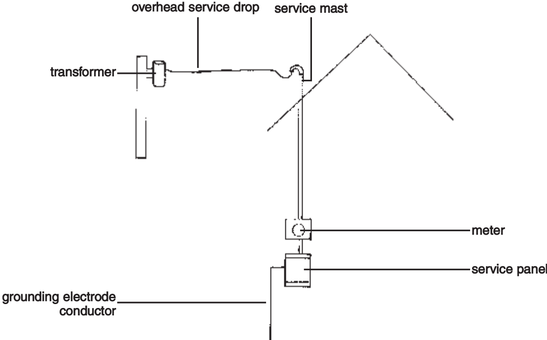
Overhead drop service.
