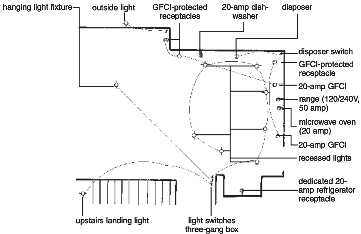
Typical kitchen wiring diagram.
