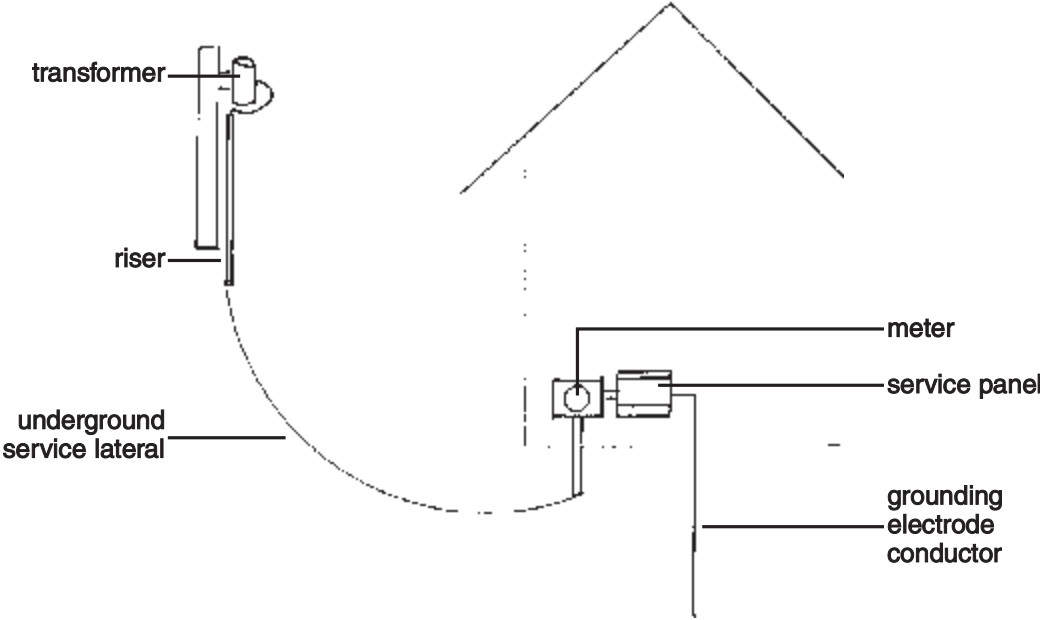
Underground service lateral.
