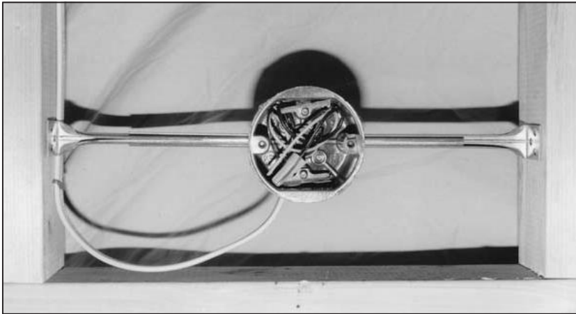
A round box with extendible bars.
