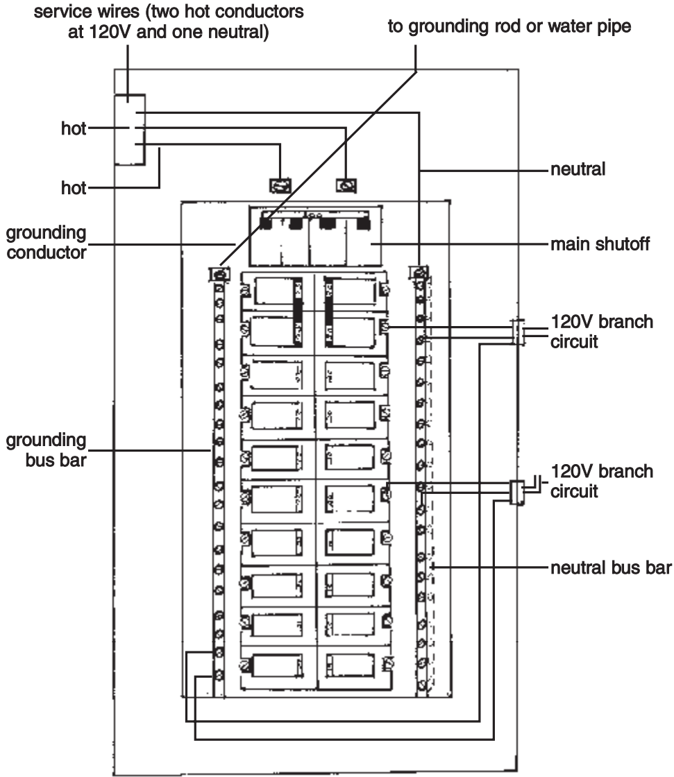
Inside of service panel.
