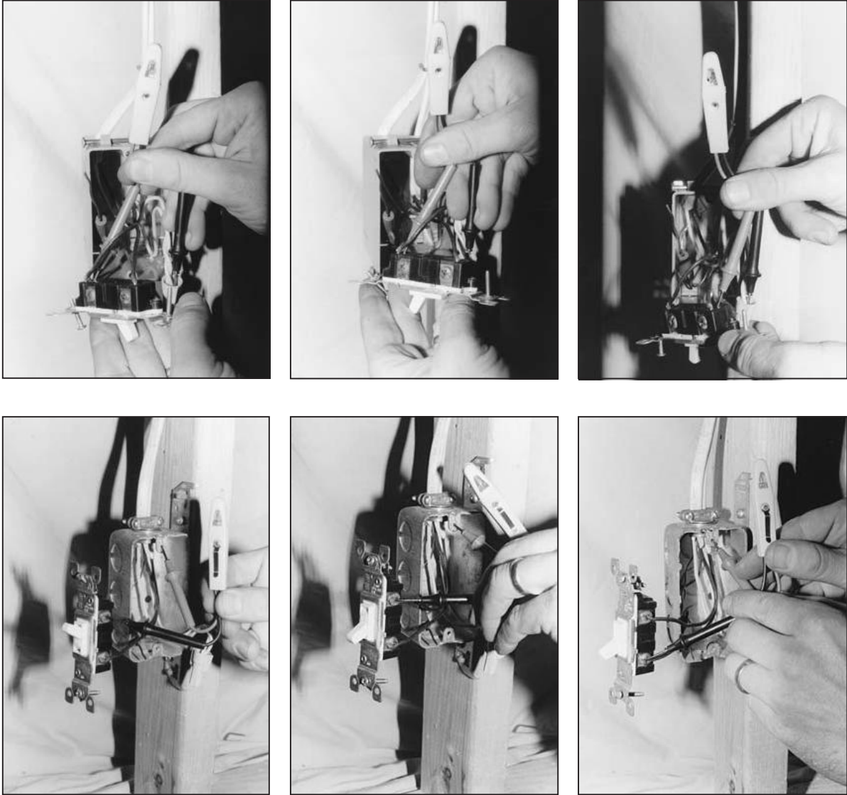
Testing terminals and testing back wiring.
