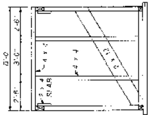
SIDE FRAMING ELEVATION
