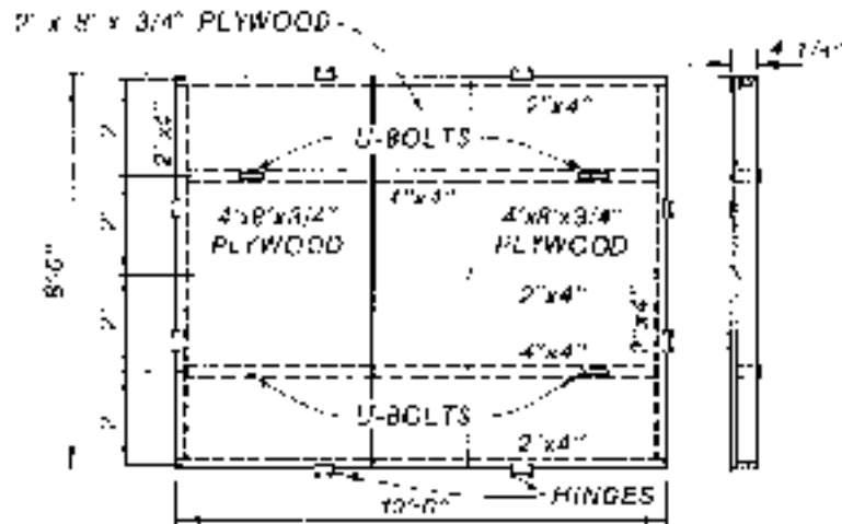
FLOOR DETAIL 1 NEEDED
