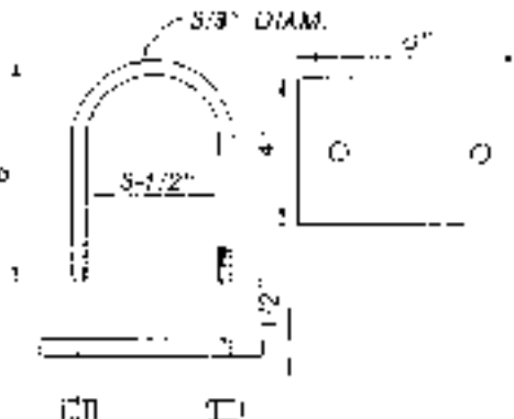
U-BOLT & BEARING PLATE 4 NEEDED
