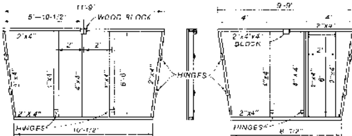
SIDE WALL DETAIL 2 NEEDED
