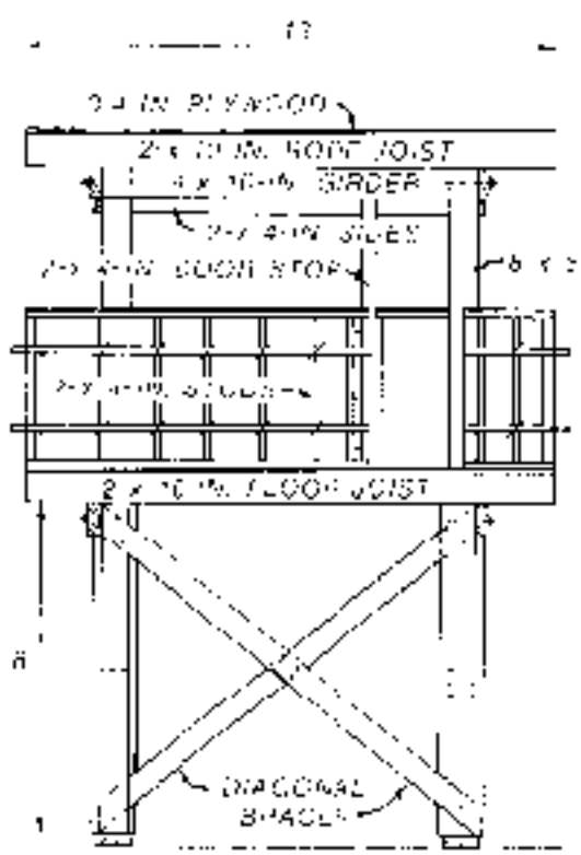
FRONT ELEVATION
