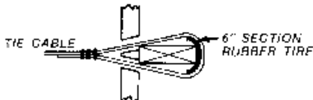
ALTERNATE TIE CABLE ATTACHMENT
