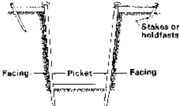
METHOD OF PLACING STAKES
