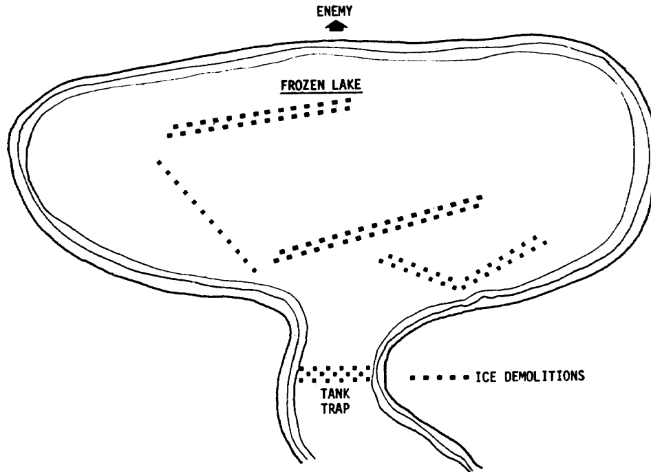
Figure 6-36. Ice demolitions.
