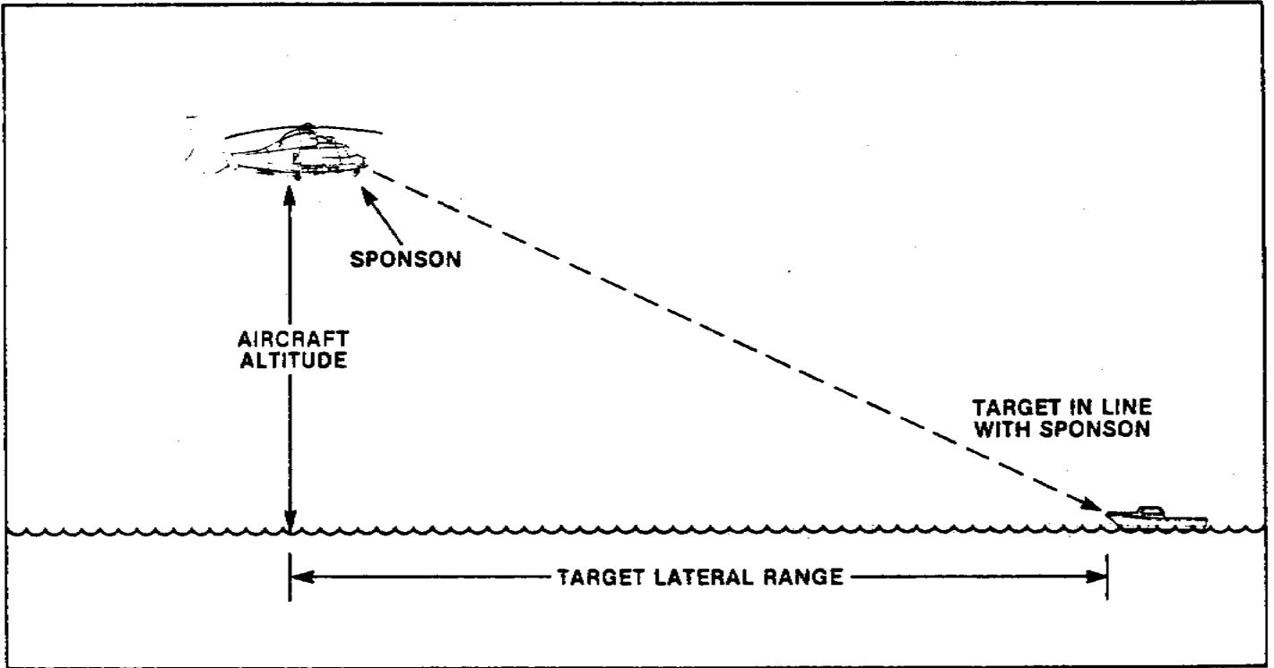
Figure 6-9. Range Estimation
