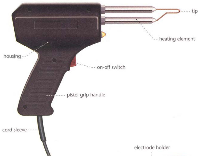
SOLDERING GUN
