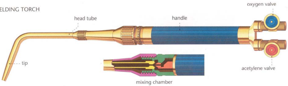
OXYACETYLENE WELDING
