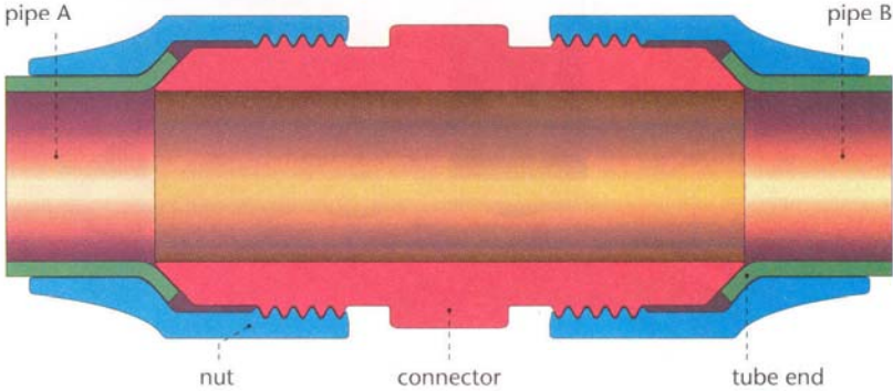
flare joint
