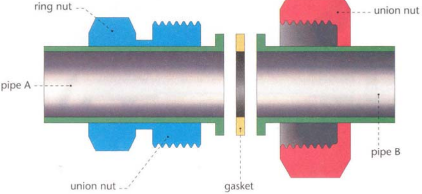
union
