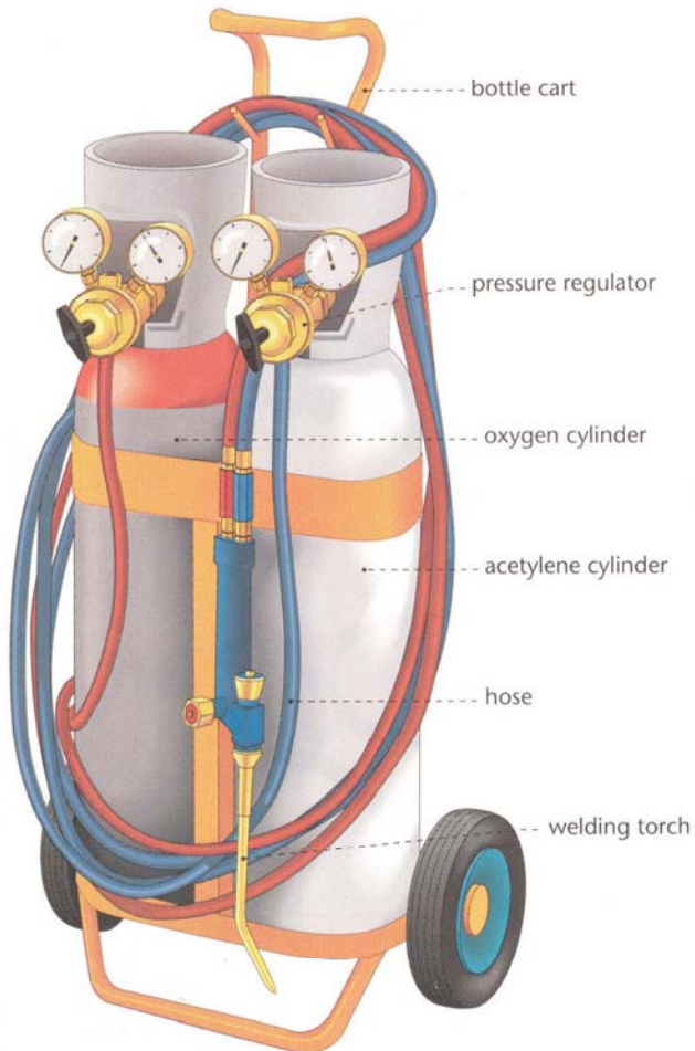
OXYACETYLENE WELDING
