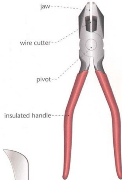
lineman's pliers
