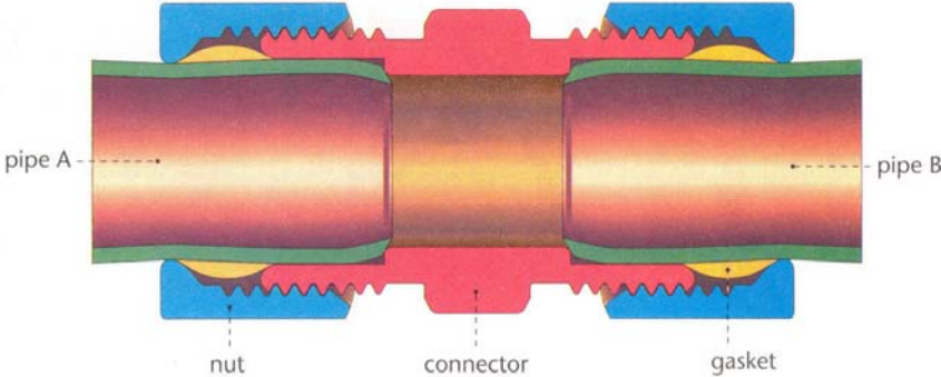
compression fitting
