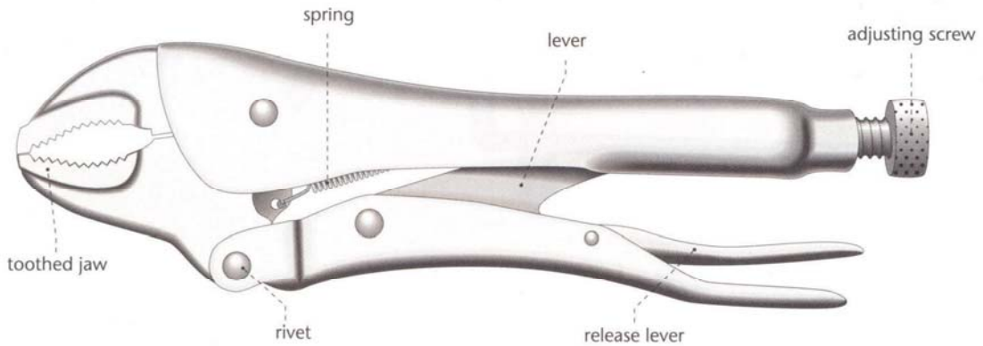
LOCKING PLIERS
