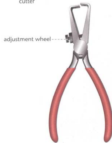
wire stripper
