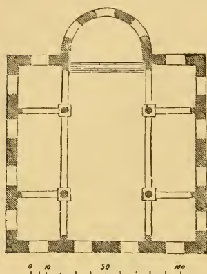
Fig. 122.—Cathedral of Trier. Groundplan.
