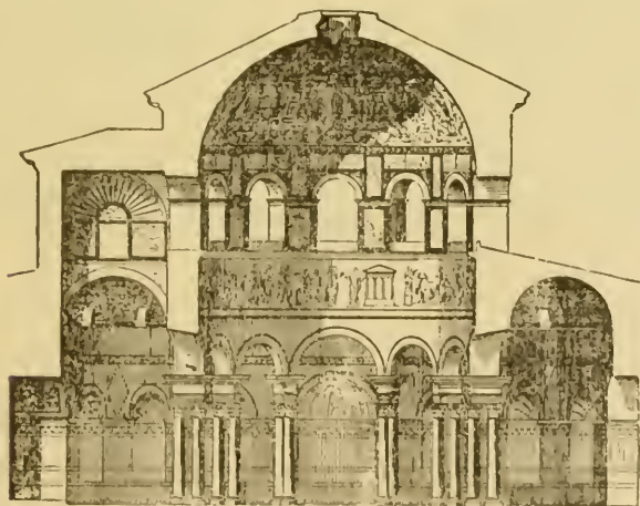
Fig. 113.—Section of Santa Costanza, Rome.
