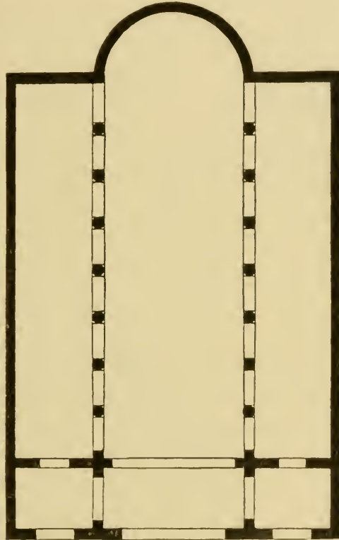
Fig. 78.—Plan of basilica from the villa of Quintillian.
