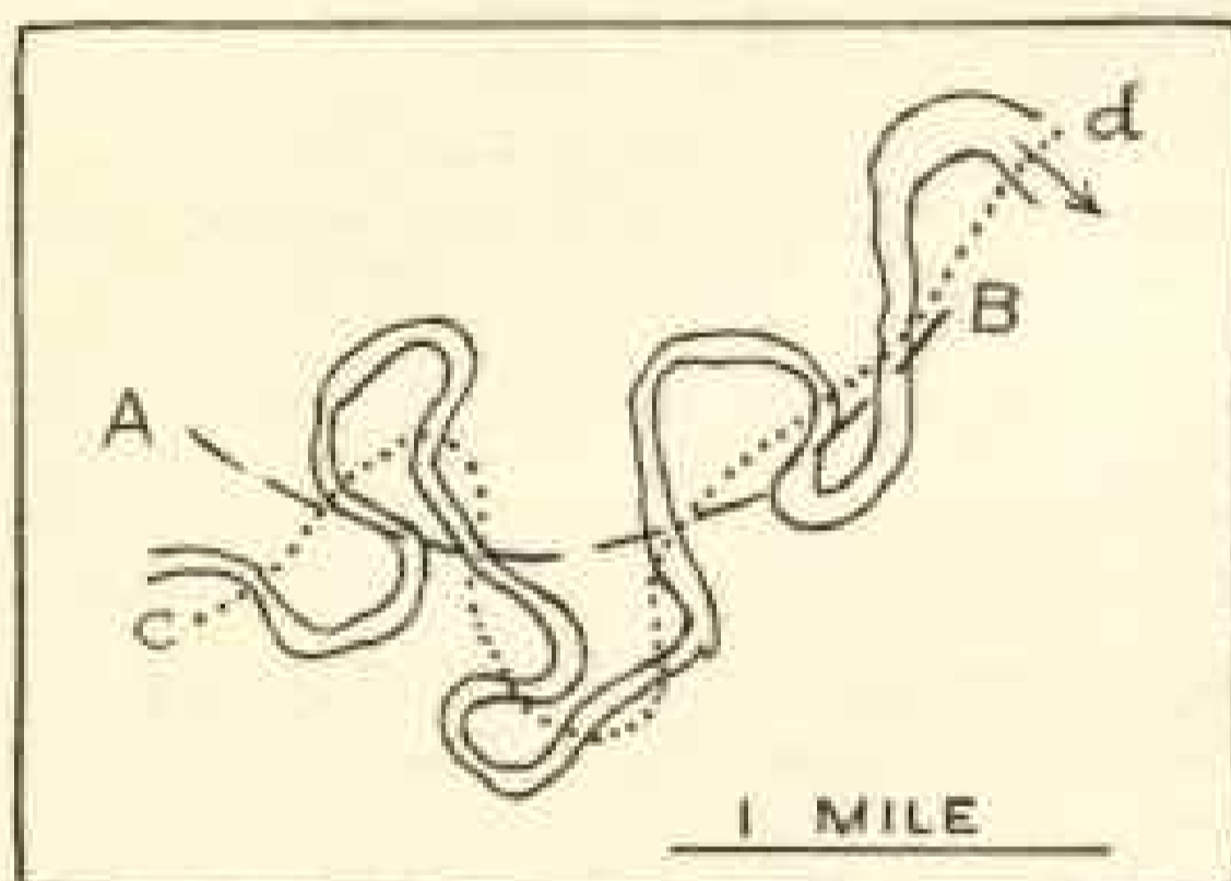
The Forth at Stirling
