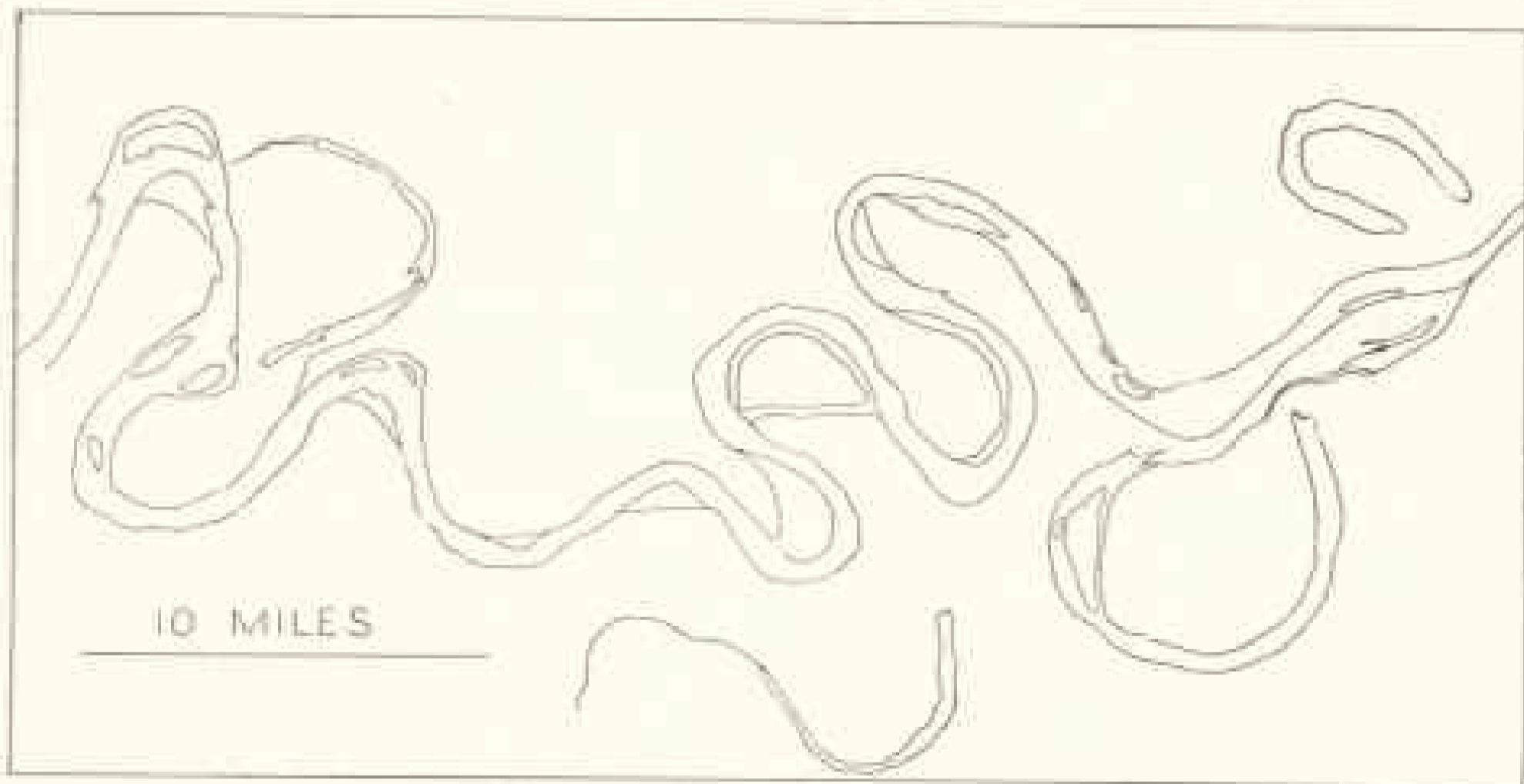
The Mississippi at Greenville
