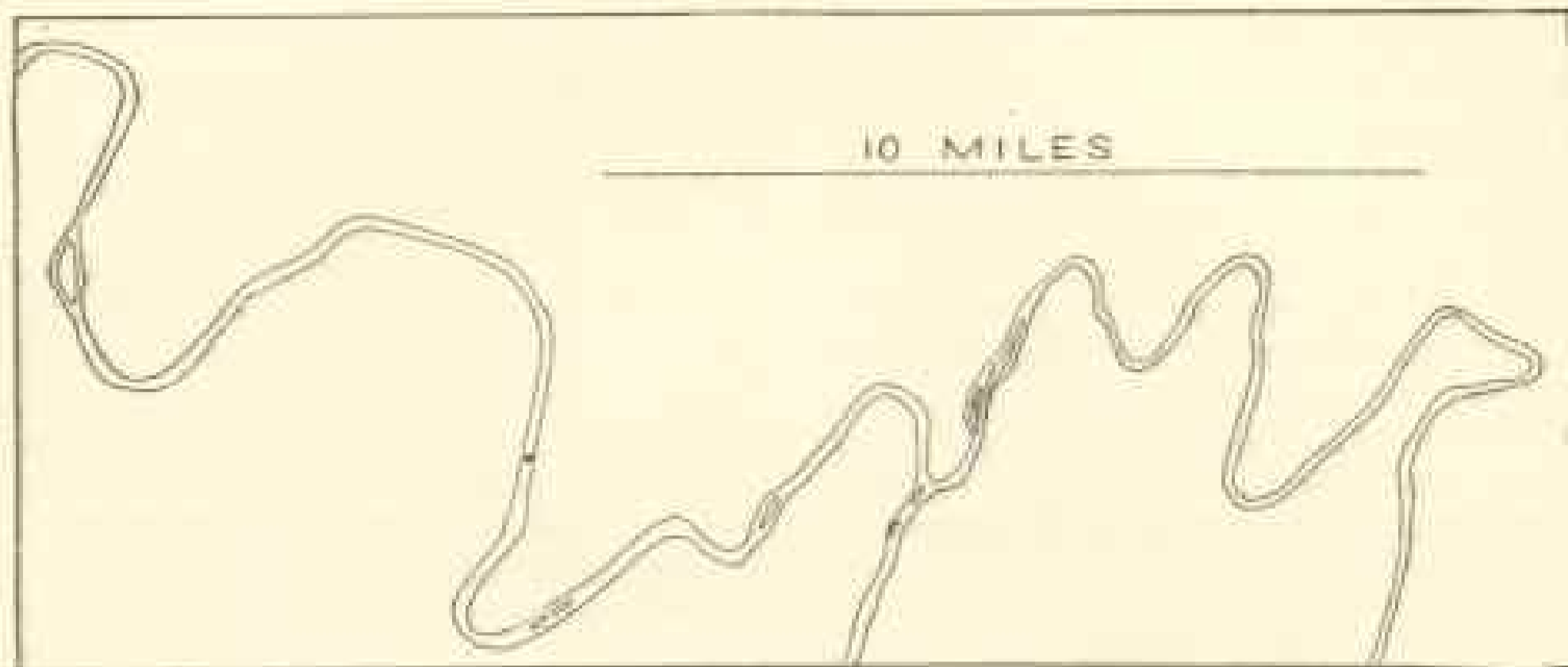
French Broad and Nolichucky
