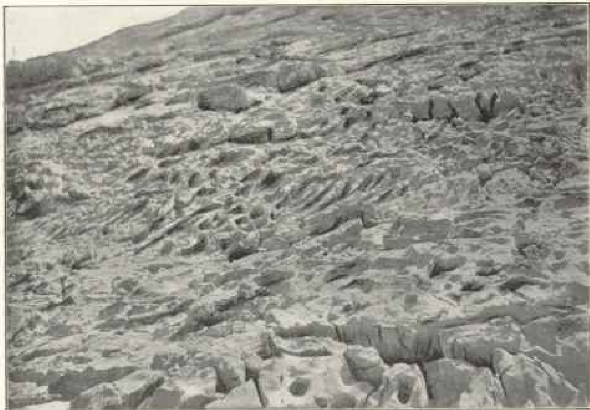
Erosion of Limestone near Silvertip Peak
