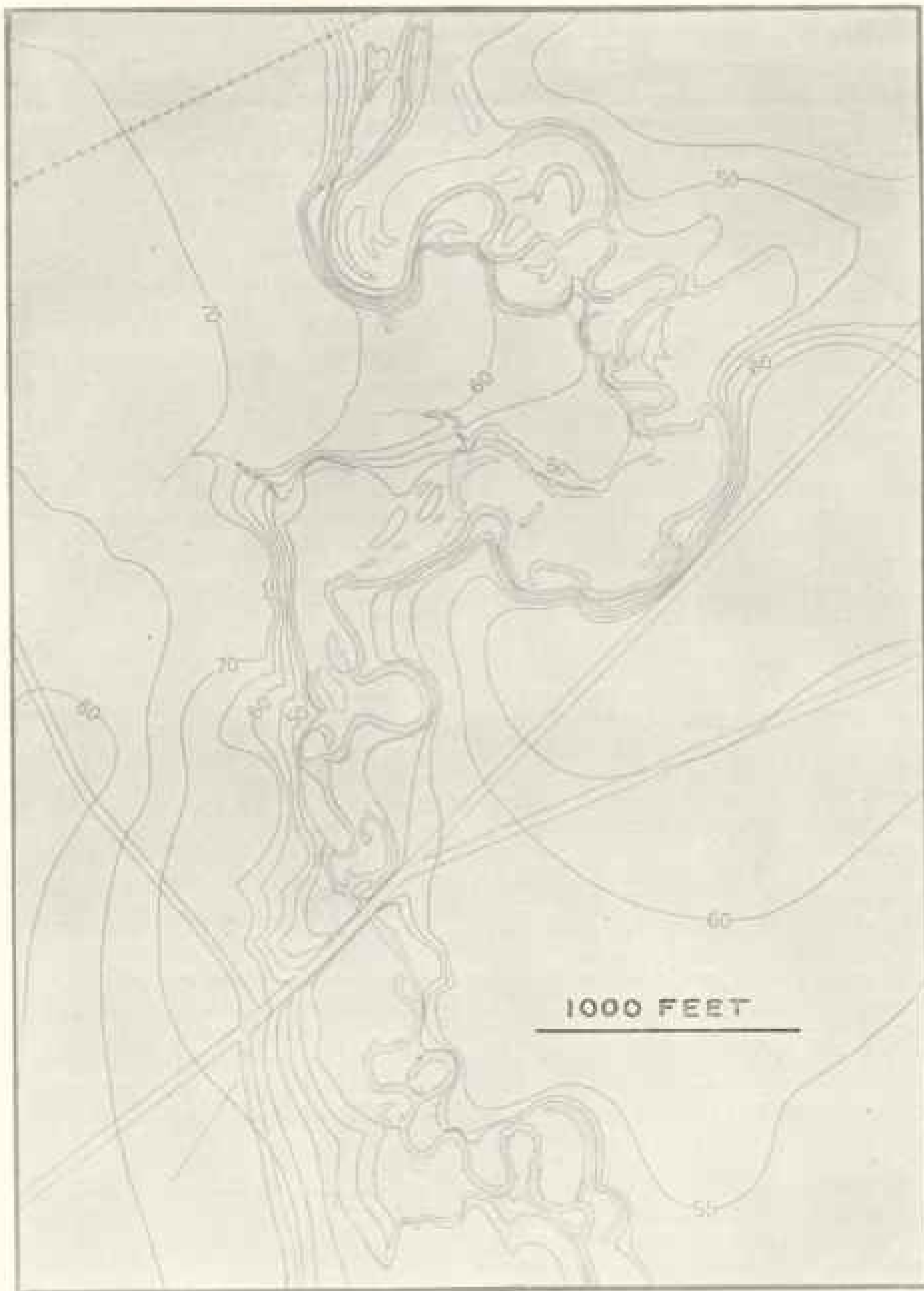
The Matfield at Elmwood, Mass.
