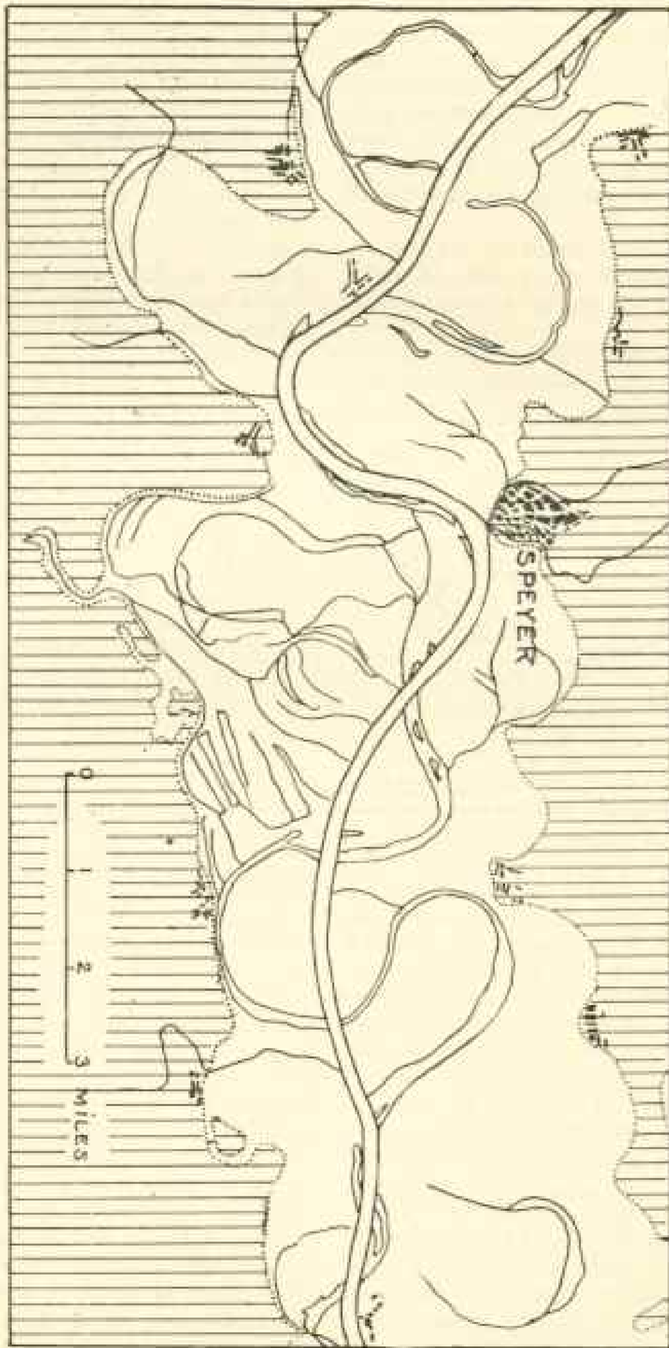
The Rhine—A Corrected Meandering Stream
