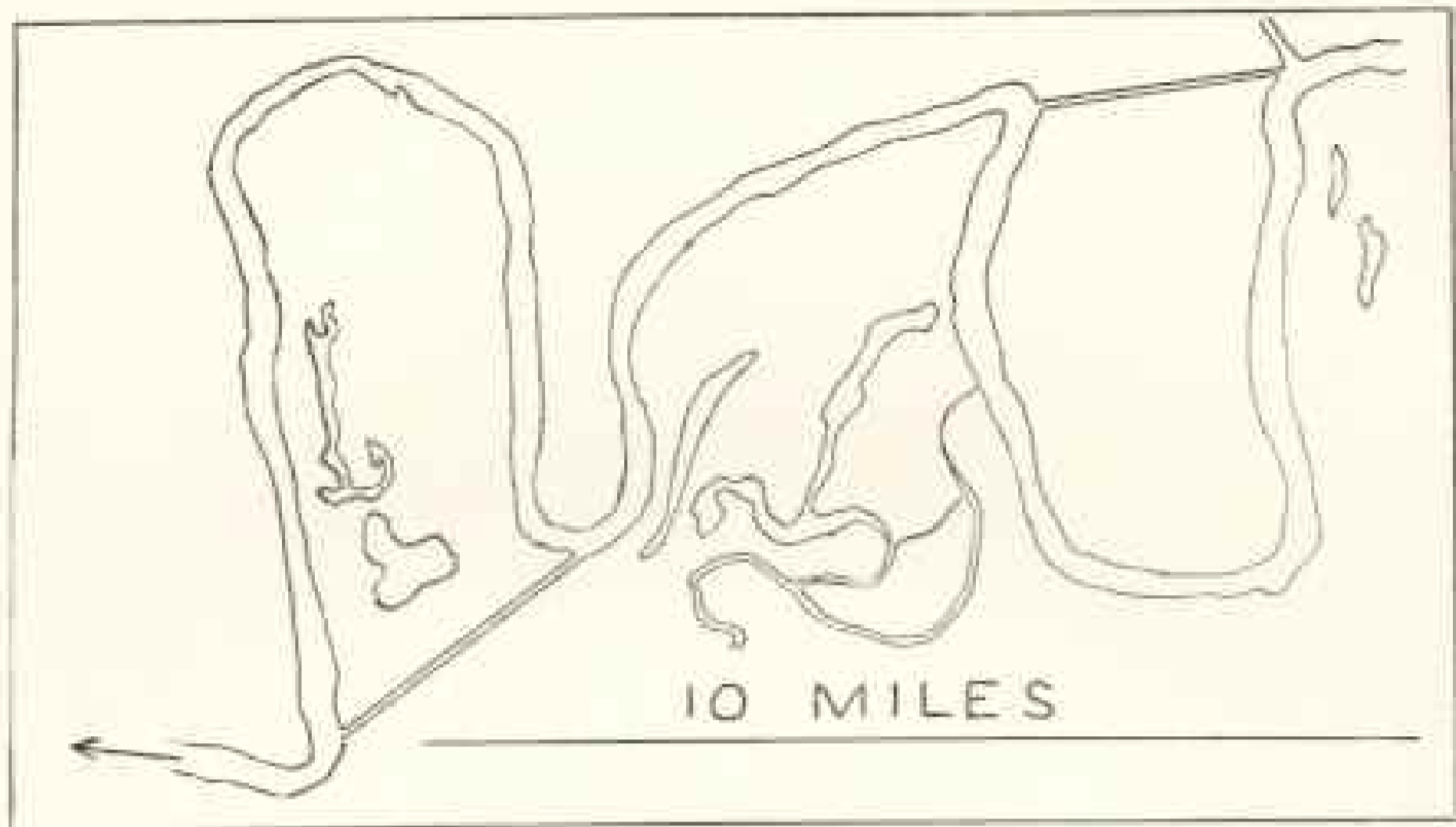
The Theiss, Basin of Hungary
