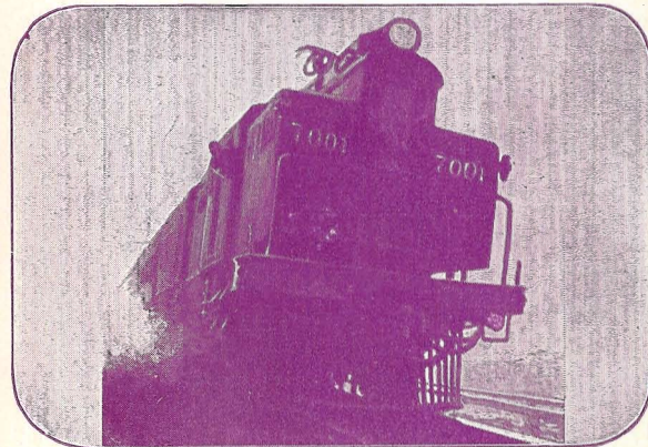
AN ELECTRIC LOCOMOTIVE
