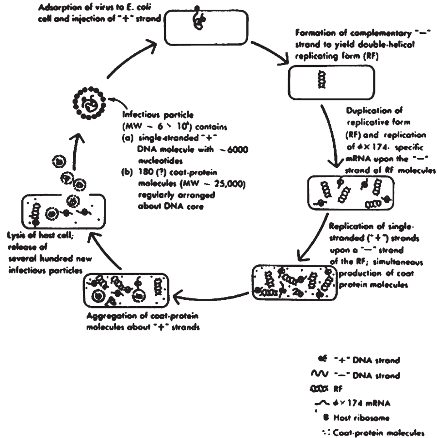
Life cycle of the \phi X174 virus. This virus employs a circular DNA. The diagram shows only a small portion of the (+), (-), and (RF) circles. MW, relative weight of a single particle or molecule, the hydrogen atom being approximately one. (from Watson)
