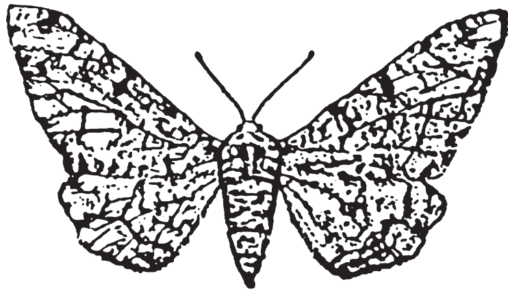
LIGHT FORM OF THE PEPPERED MOTH
