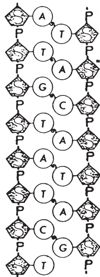
CHEMICAL COMPOUNDS IN DNA
