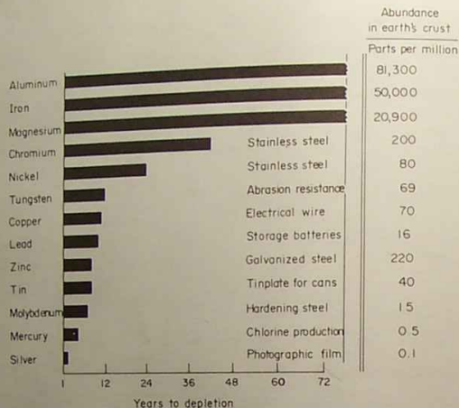
Fig. 5. Depletion of world reserves of commercial grade ores if world population had U.S. living standard. (Source: Gough and Eastland, 1969, based on data from U.S. Bureau of Mines.)
