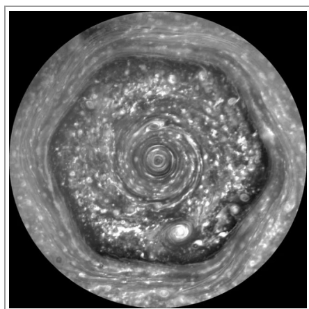
Hexagon on Saturn's North Pole. One
