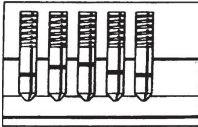
Pins are in the unpicked position
