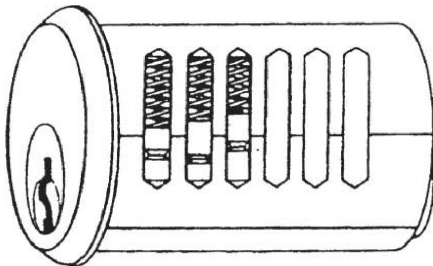
Example of three pin combination
