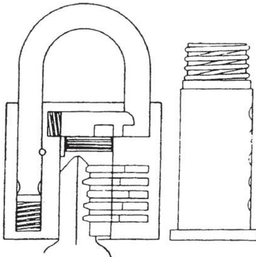
Cut-away view of spring loaded plug
