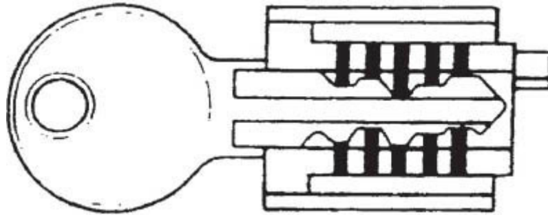
Double sided disc tumbler cylinder
