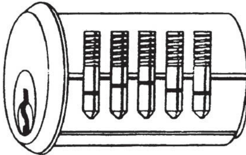
Clearance between plug and body
