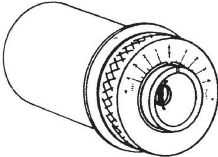
HPC Torque N' Tension Tool in position over lock cylinder face
