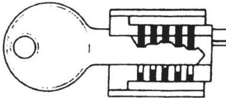
Single sided disc tumbler cylinder
