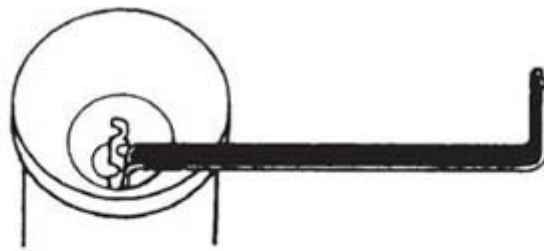
Grooved ends, rigid tension tool
