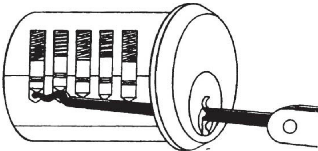
Pick is able to come into contact with all pins
