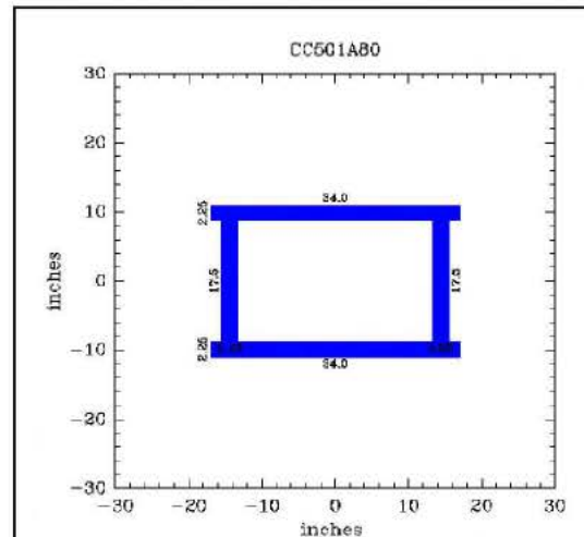
Dimensions of one of the 47 steel core columns between the 77 th and 80 th floors as reported by NIST
