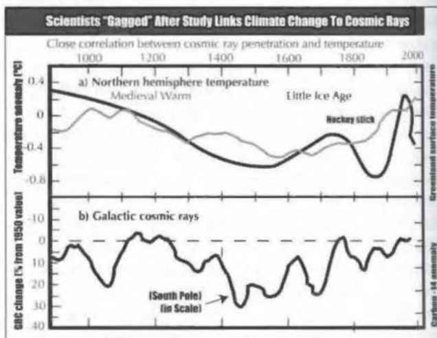
Figure 545: Correlation between cosmic rays and temperature.
