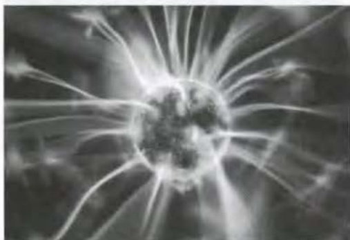
Figure 121: Plasma is a near-perfect medium for electricity.
