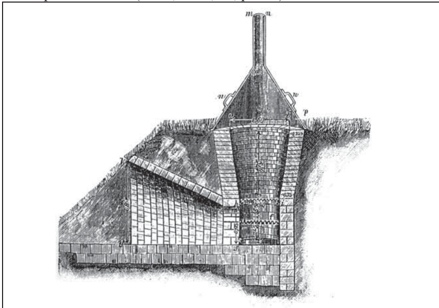
Document 11: Feist oven for the destruction of carcasses of infected animal. (de Cristoforis 1890, p. 126)
