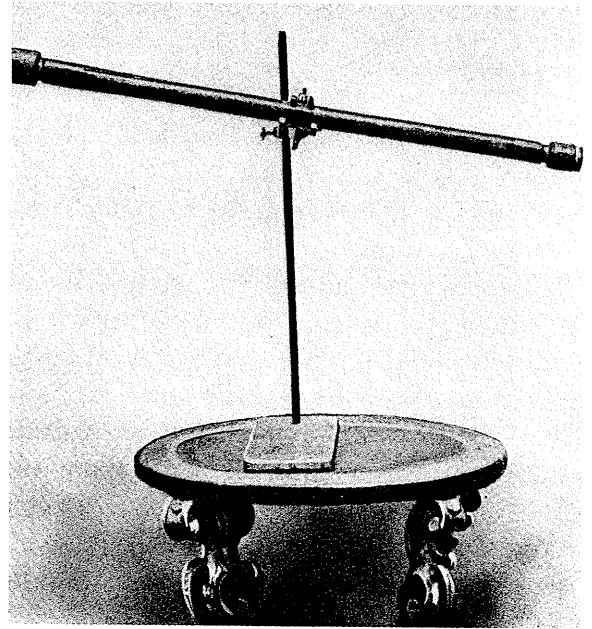
Galileo's telescope.
