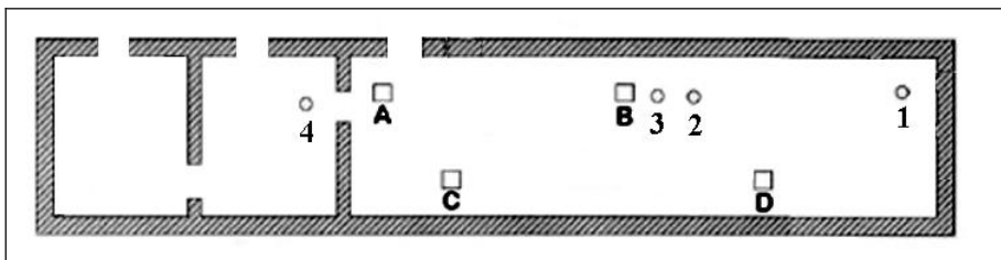
III. 75: Schematic floor plan of the morgue of crematory I with washing and surgery room (original situation). A, B, C, D: location of current openings in the roof made after the war. 1, 2, 3, and 4: location of original openings of the air raid shelter for ventilation and heating ducts, today closed. 573
