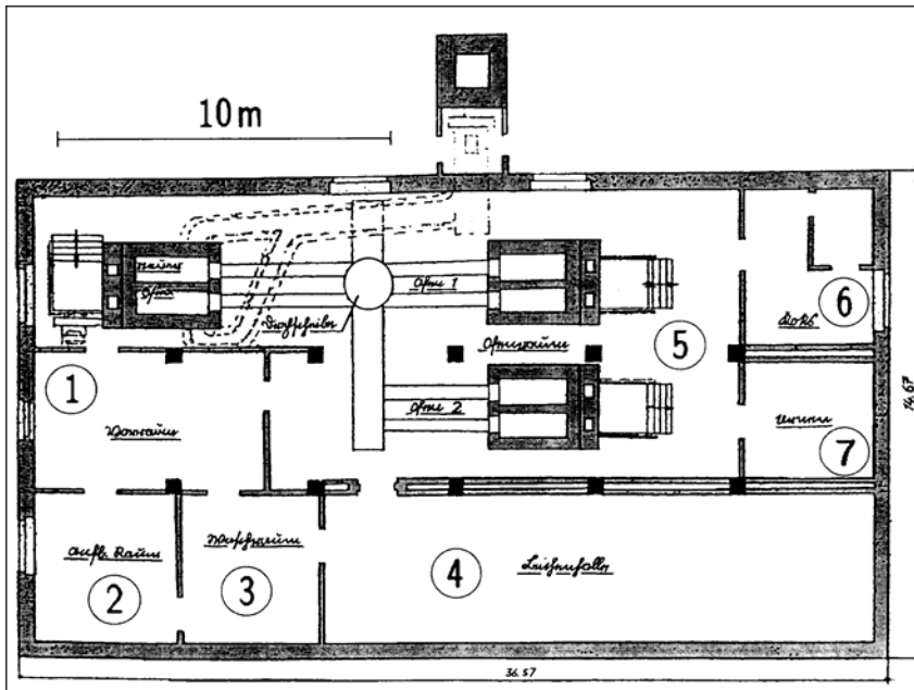
III. 71: Floor plan of crematory I, Auschwitz main camp, as originally planned. The morgue is alleged to have been used later as a gas chamber. 562 1: ante-chamber; 2: laying out room; 3: wash room; 4: morgue; 5: oven room; 6: coke; 7: urns
