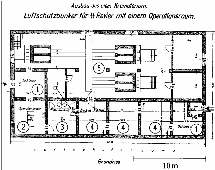
III. 72: Floor plan of crematory 1 at Auschwitz main camp after conversion to air raid shelter in 1944. 566 1: air lock; 2: surgery room; 3: former washroom, now room of air raid shelter with toilets; 4: air raid shelter rooms; 5: former oven room
