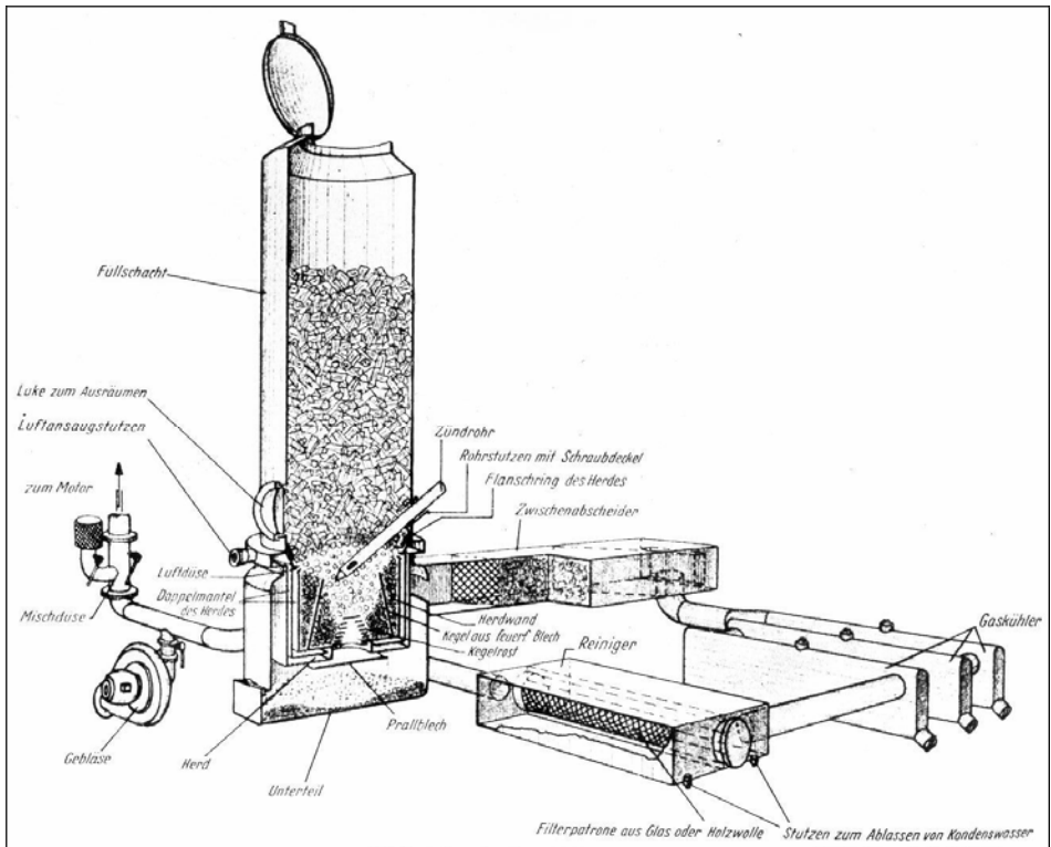
III. 92: Design of an Ostmark Gas Generator.
