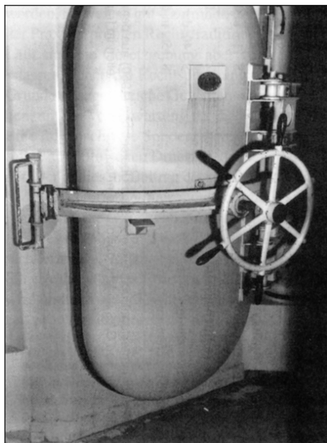
III. 85: Door to an execution gas chamber for one single person (Baltimore, USA, 1954, technology from the 1930s).
