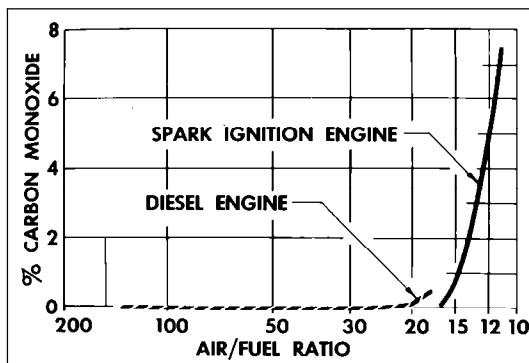
III. 88: Carbon monoxide content of exhaust gases from spark engines and diesel engines as a function of engine load (air/fuel ratio)
