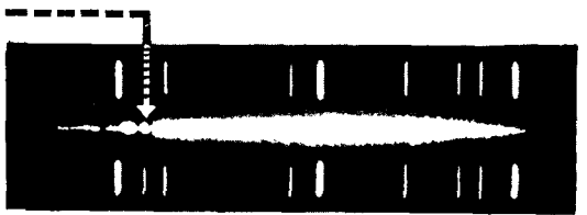
VIOLET RED Spectrum of galaxy in the constellation Virgo; distance 10,000,000 light years; the red shift indicates a recession of 1,000 km/sec.
