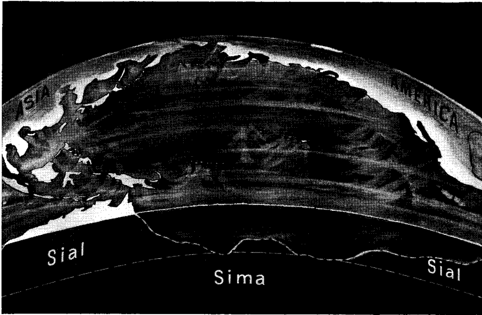
Fig. 129. THE HOLE IN THE PACIFIC
