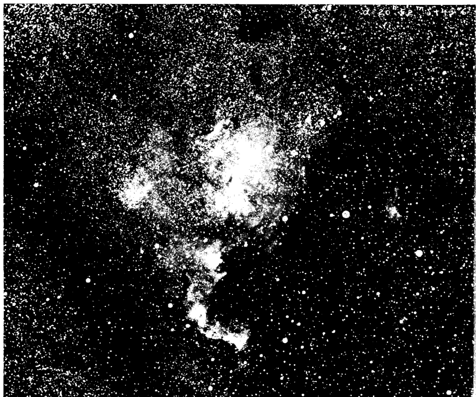
Fig. 3. THE INFINITY OF THE UNIVERSE IS RECOGNIZED
