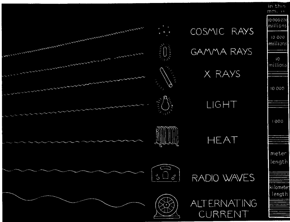
Fig. 23. THE GAMUT OF ELECTROMAGNETIC WAVES Electromagnetic waves are rhythmical disturbances of the electromagnetic field. Their length varies from cosmic rays to the waves of alternating current.
