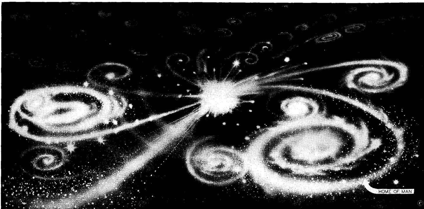
Fig. 64. THE EXPLODING UNIVERSE
