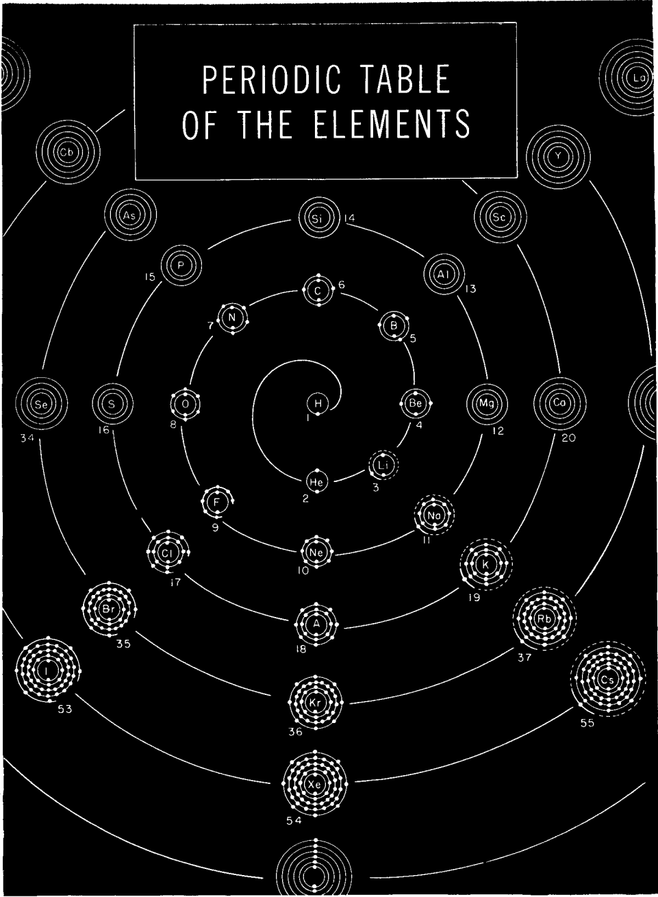
Fig. 19. THE PERIODIC TABLE OF THE ELEMENTS The chemical properties of the elements are determined by the number of the electrons in the outer orbit of the atom. Elements having the same number of electrons or gaps in the outer orbit resemble each other in chemical properties and form "families," such as the atoms 2, 10, 18, 36, 54, which are filled to capacity and known as the rare gases.
