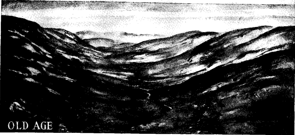
Fig. 136. FROM MOUNTAINS TO MOUNDS
