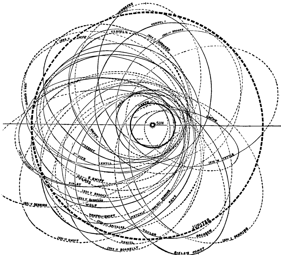
Fig. 88. THE "COMET-FAMILY" OF JUPITER Huge Jupiter has "captured" several dozen comets which shuttle between Jupiter and the sun in elliptic and parabolic orbits. The small black circle is the orbit of the earth, the large broken circle is the orbit of Jupiter.
