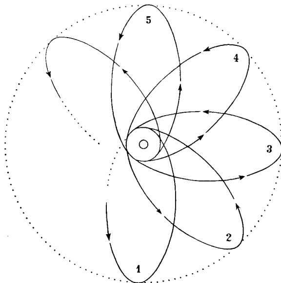
Fig. 11. FIRST PROOF OF THE CURVATURE OF SPACE
