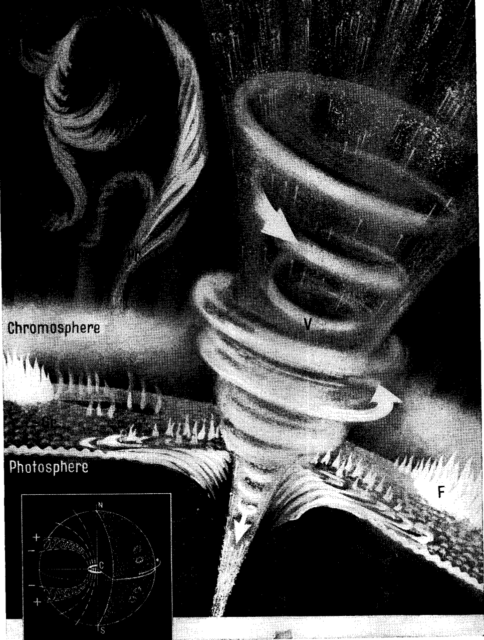
Fig. 68. SURFACE OF THE SUN
