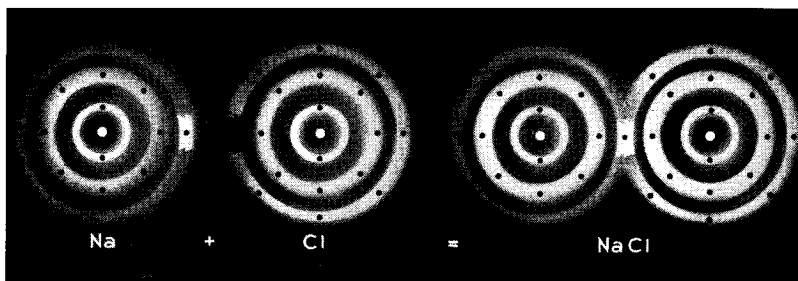
Fig. 20. CHEMICAL AFFINITY
