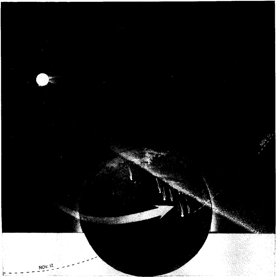
Fig. 90. SHOOTING STARS
