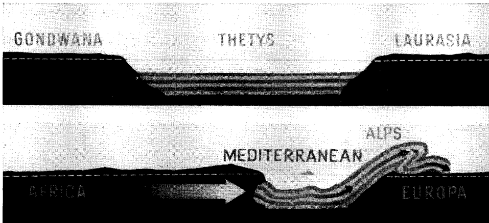
Fig. 106. THE THEORY OF THE DRIFTING CONTINENTS I
