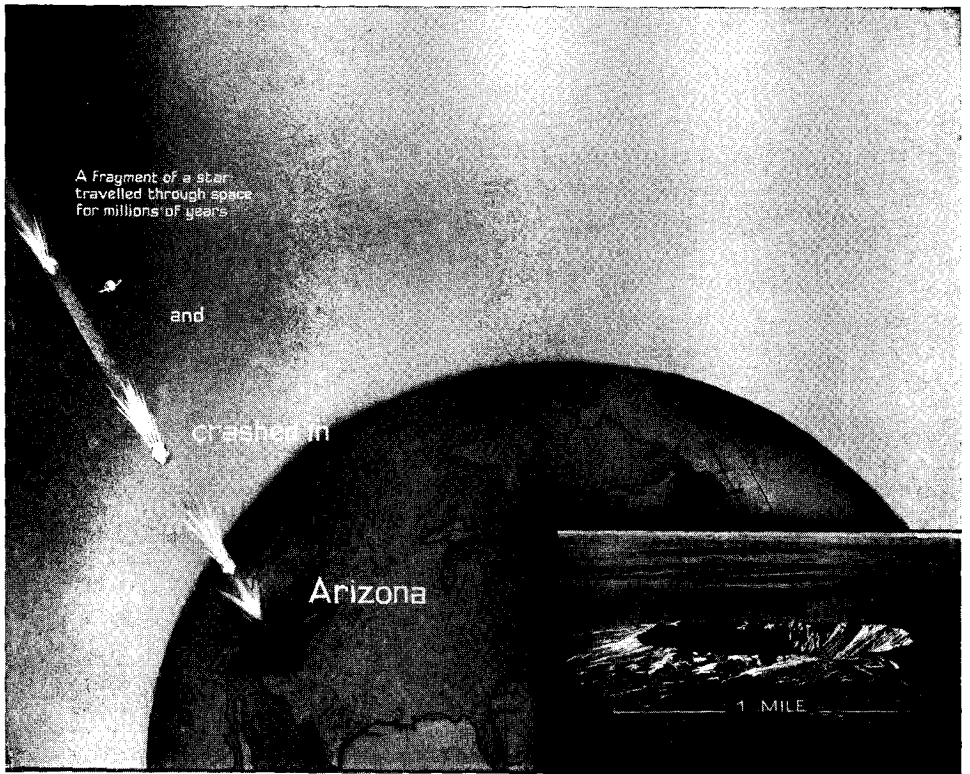
Fig. 91. METEORITES
