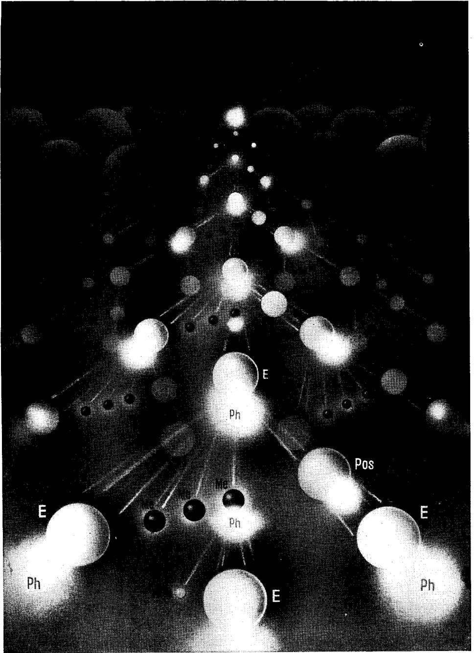
Fig. 33. COSMIC RADIATION One atmospheric atom hit by a cosmic proton ( above ) touches off the chain reaction of cosmic radiation ( below ). E, electron; Ph, photon; Me, meson; Pos, positron; Neu, neutrino.
