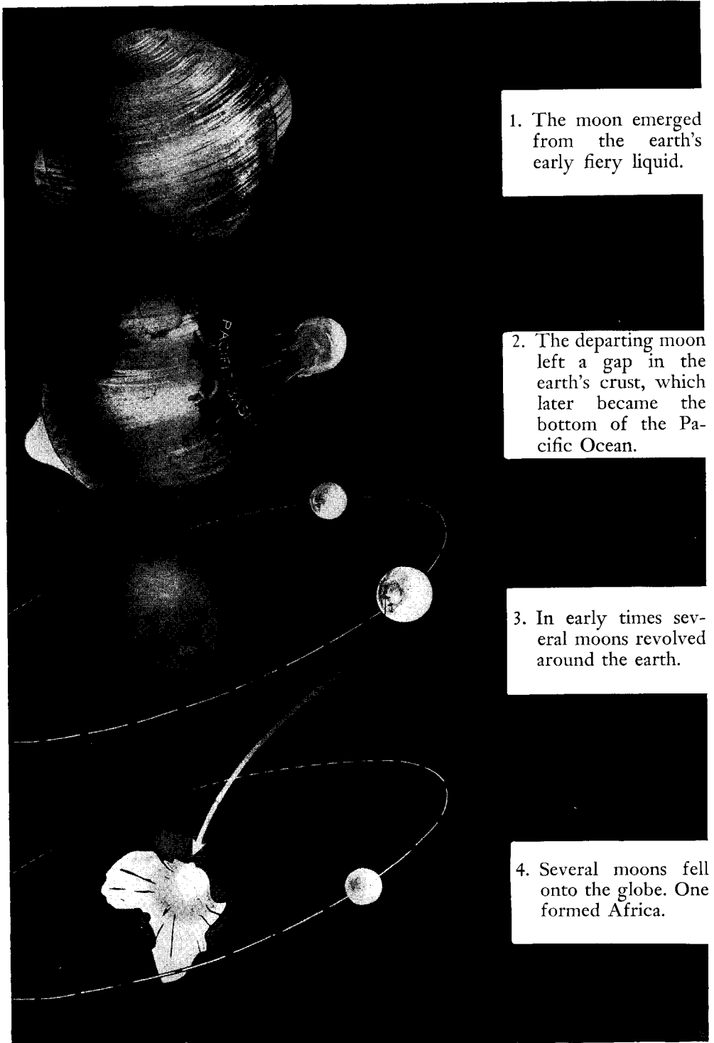
Fig. 96. HYPOTHESES ABOUT THE MOON
