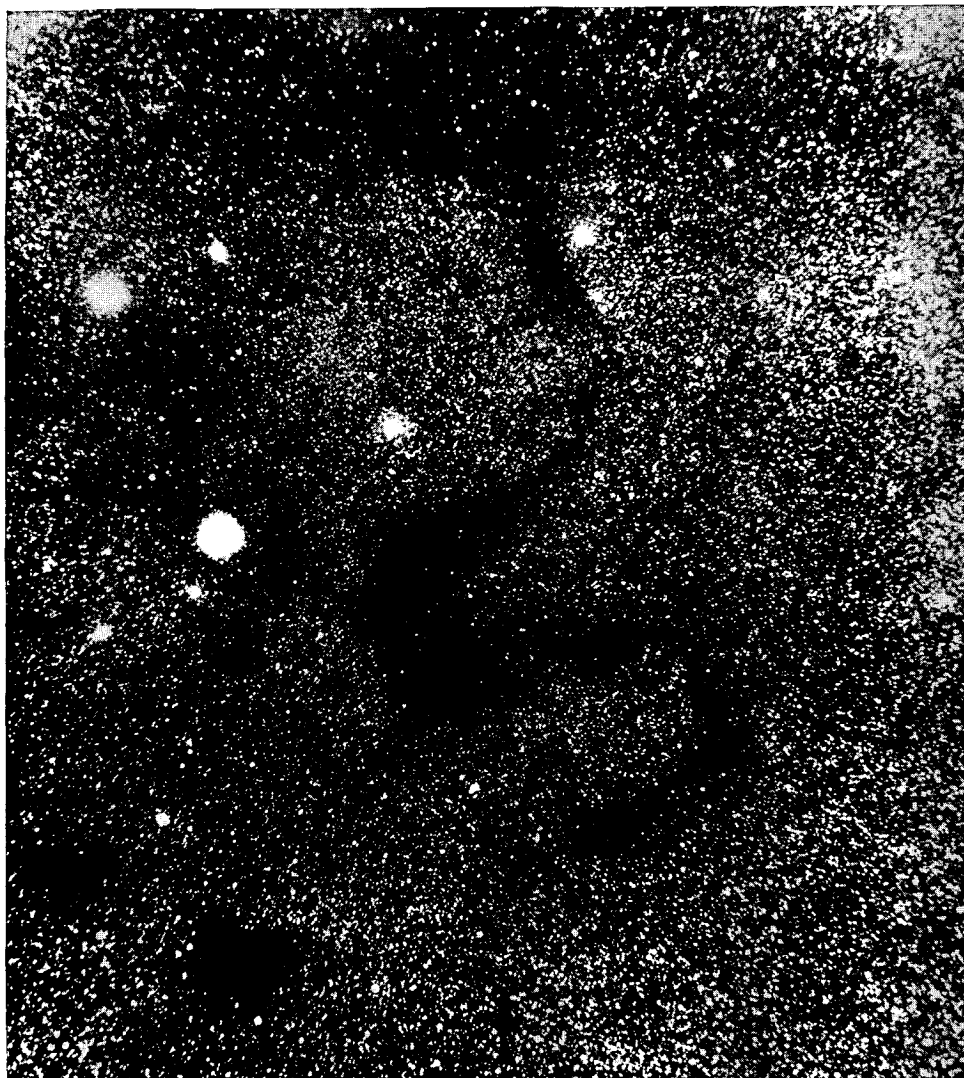
Fig. 60. THE COAL SACKS IN THE MILKY WAY
