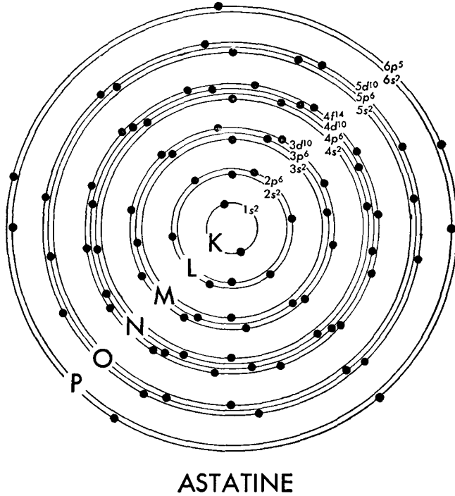
Fig. 18. THE SHELLS OF THE ATOM
