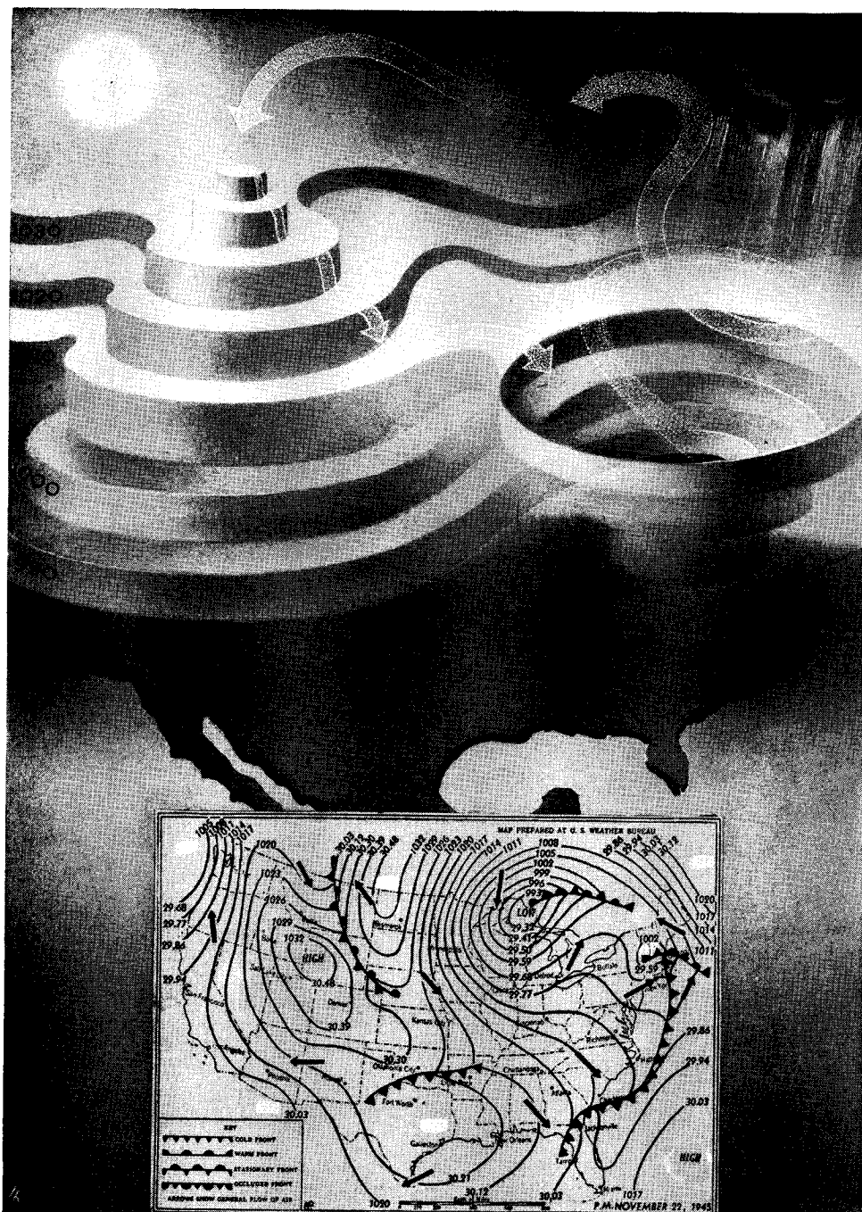
Fig. 125. WEATHER MAP
