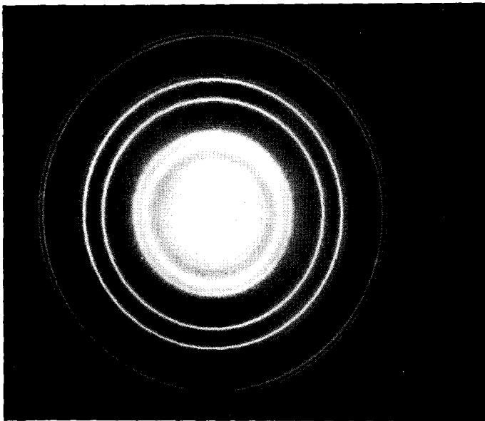
Fig. 48. THE WAVE- CHARACTER OF THE ELECTRON
