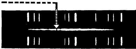
Galaxy in Corona borealis; distance 150,000,000 light years; recession 20,000 km/sec.
