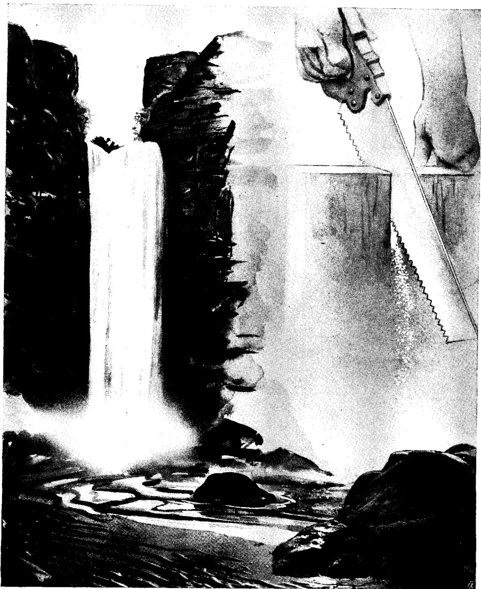
Fig. 133. WATERFALLS
