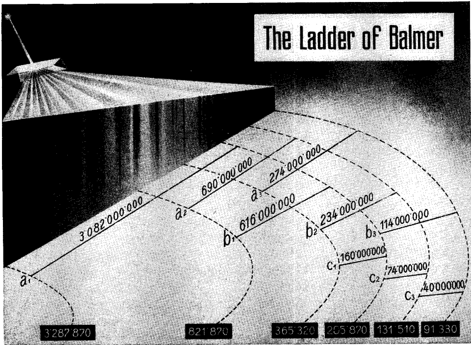
Fig. 54. THE SPECTROGRAM
