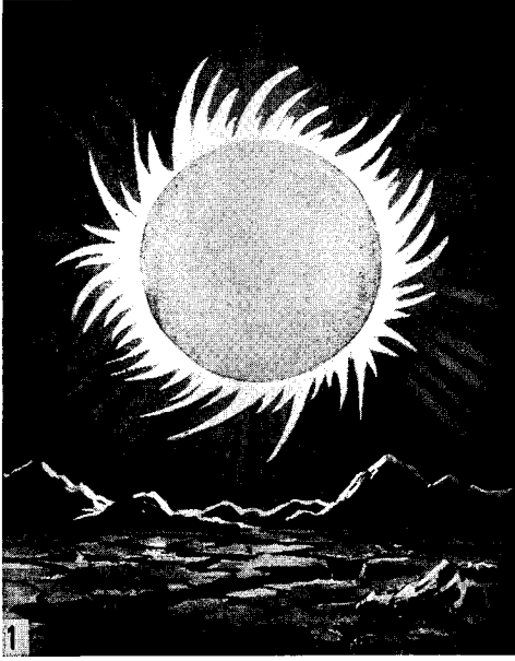
MERCURY
