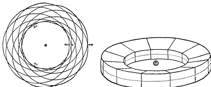
Fig. 95. THE COURSE OF THE MOON
