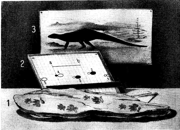
Fig. 102. FOSSILS
