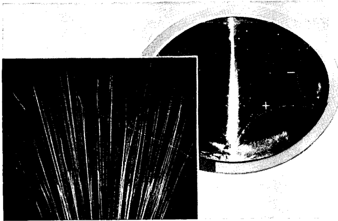
Fig. 15. PHOTOGRAPHY OF FLYING PAR- TICLES OF THE ATOM
