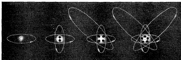
Fig. 35. THE LAW OF PROTONS AND THE RULE OF NEUTRONS The law of protons: the nucleus of the atom contains as many protons as there are electrons in the shells. The rule of neutrons: the higher the number of protons, the greater the excess of neutrons.
