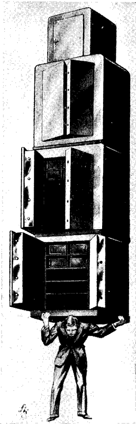
Fig. 116. THE ATMOSPHERIC PRESSURE
