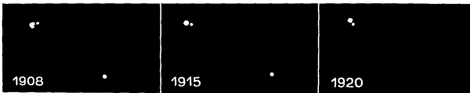
Fig. 70. DOUBLE STARS
