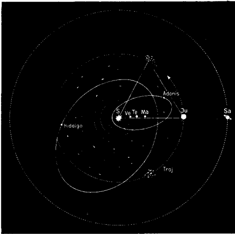
Fig. 83. THE TROJANS
