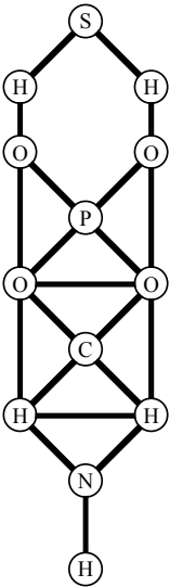
Figure 2: Schematic representation of the emergence of key biomolecular functional groups using the Tree of Life. In addition to H-O, C=O, O=C-O-H, N-H 3 , S-H and P-O 4 groups, molecules such as H 2 O and CO 2 can be seen.
