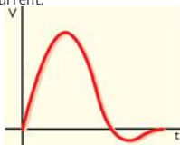
Fig 1. The damped sine monophasic waveform.
