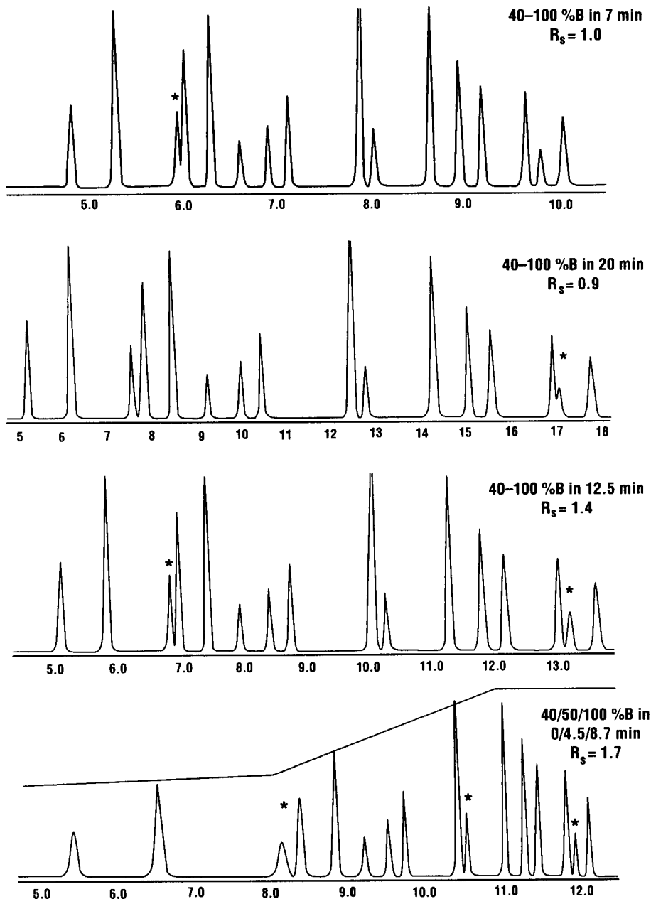
FIGURE 8.13 Gradient separations of a polyaromatic hydrocarbon sample as a function of gradient steepness. Sample: 16 compounds ranging from naphthalene to indenopyrene. Conditions: 15 \times 0.46 -cm Supelco LC-PAH (reversed-phase) column; acetonitrile-water gradients; 2 mL/min; 35^\circ\text{C} . (Computer simulations based on data of Ref. 21.)
