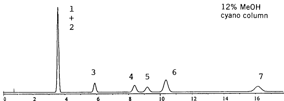
FIGURE 6.17 Separation of a mixture of substituted benzoic acids on three different column types. Conditions: 15 \times 0.46 -cm, 5\text{-}\mu\text{m} columns; mobile phase as indicated, buffer is 25 mM citrate (pH 2.5); 2.0 mL/min; 35°C. (a) % MeOH adjusted to give k = 20 for last band; (b) % MeOH adjusted to give k = 0.5 for first band; (c) % MeOH adjusted to give maximum resolution. (Chromatograms are simulations based on data of Ref. 11.)
