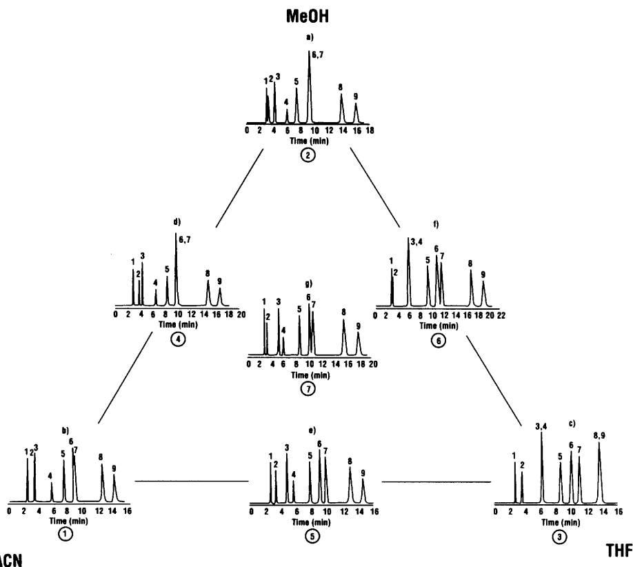
FIGURE 6.16 Seven chromatograms for solvent-selectivity experiments for substituted naphthalenes. Column 15 × 0.46-cm Zorbax-C8, flow rate 2.0 mL/min; 40°C. (Chromatograms from data in Ref. 23.)
