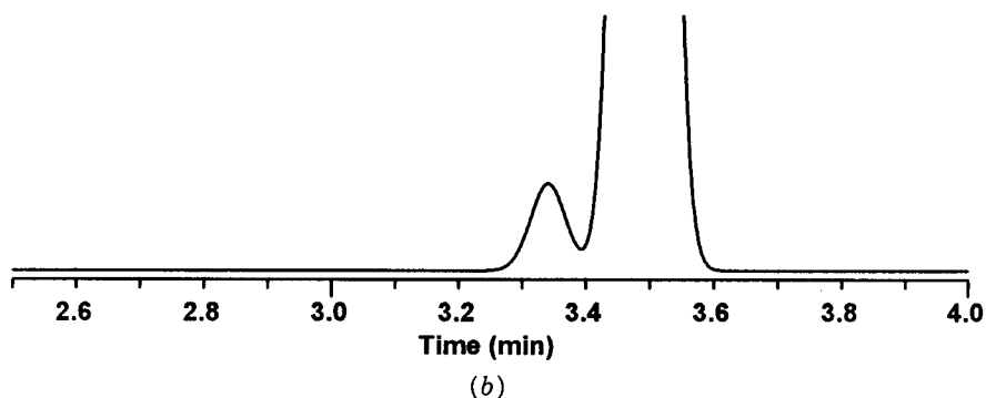
FIGURE 15.6 Collection of a peak and reinjection using a different chromatographic method. Main peak in (a) is collected and reinjected in (b), which shows evidence of a coeluting peak from the original separation.
