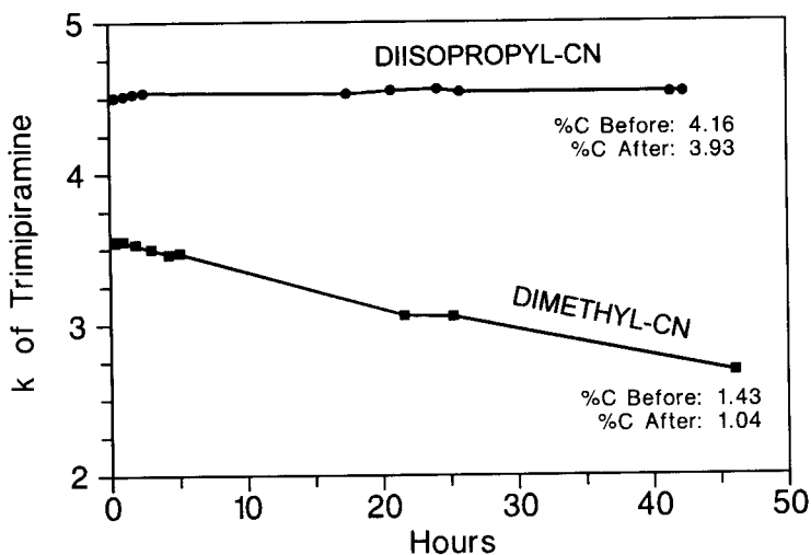
FIGURE 5.13 Comparison of stability for short-chain cyano-bonded phases. Columns: 15 \times 0.46 cm; mobile phase: 28:72 acetonitrile-0.1% trifluoroacetic acid adjusted to \text{pH} 2.0 with triethylamine; flow rate: 1.0 mL/min; 50^\circ\text{C} .
