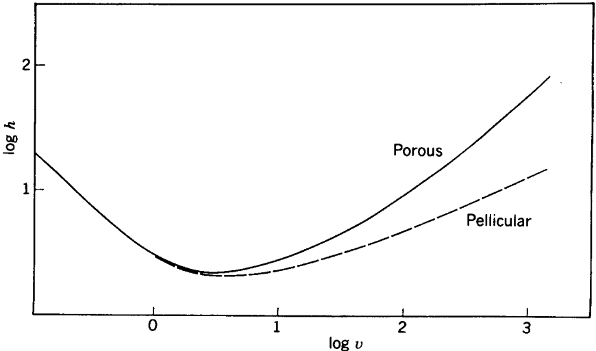
FIGURE 2.12 Theoretical dependence of column efficiency on flow rate. Knox equations for porous and nonporous columns (reduced parameter plots). See the text for details. For porous column, Eq. 2.10a with A = 1 , B = 2 , and C = 0.05 . For nonporous columns, Eq. 2.10a with A = 1 , B = 2 , and C = 0.003 .
