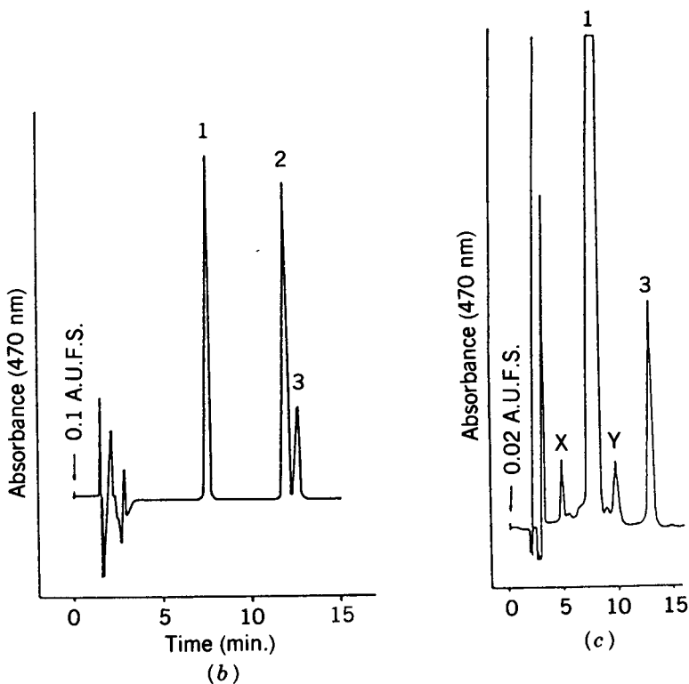
FIGURE 6.20 Non-aqueous reversed-phase (NARP) separations of carotenes. Conditions: 25 \times 0.46 -cm C_{18} column; 8% chloroform-ACN mobile phase; 2.0 mL/min; ambient temperature; UV detection at 470 nm. (Reprinted with permission from Ref. 39.)
