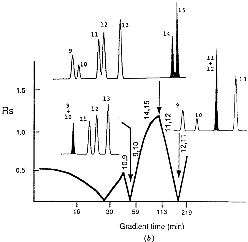
FIGURE 2.4 Resolution map for the separation of a peptide mixture by gradient elution. (a) Chromatogram for 120-min gradient; (b) resolution map with separation of bands 9 to 15 superimposed for gradient times of 52, 93, and 185 min. See the text for details. (Reprinted with permission from Ref. 3.)
