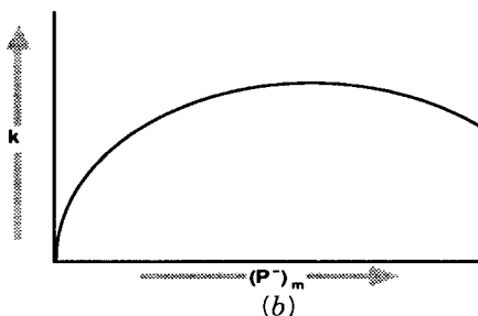
FIGURE 7.10 Effect of ion-pair reagent concentration on separation. (a) Sorption of the ion-pair reagent as a function of concentration for reagents of differing hydrophobicity ( \text{C}_6^- and \text{C}_8^- -sulfonates); (b) retention as a function of reagent concentration. See the text for details.
