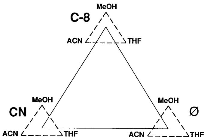
FIGURE 6.18 Method development using combined solvent- and column-type selectivity. Schematic diagram of experimental approach using C_8 , cyano, and phenyl ( \emptyset ) columns with mobile phases containing ACN, MeOH, and THF. Solvent strength and run time held constant. (Reprinted with permission from Ref. 29.)
