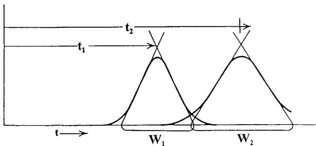
FIGURE 2.2 Calculation of resolution R_s for two adjacent bands 1 and 2. See the text for details.
