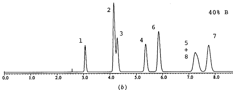
FIGURE 7.5 Separation of substituted anilines as a function of percent methanol (% B). Sample: 1, 4-methoxy; 2, N -ethyl; 3, 3-methyl; 4, 3,5-dimethyl; 5, 4-chloro; 6, 3-cyano; 7, 3-chloro; 8, 2-chloro. Conditions: 25-cm Zorbax SB-C8 column; methanol–buffer (25 mM sodium citrate, pH 3.5); mobile phases; 35°C; 1.0 mL/min. (a) 20% methanol; (b) 40% methanol. (Simulated chromatograms based on experimental data of Ref. 3.)
