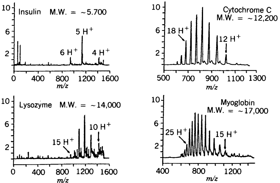
FIGURE 3.17 Typical ion envelope from multiply charged peptide and protein ions in ESP. (Reprinted with permission from Ref. 37.)
