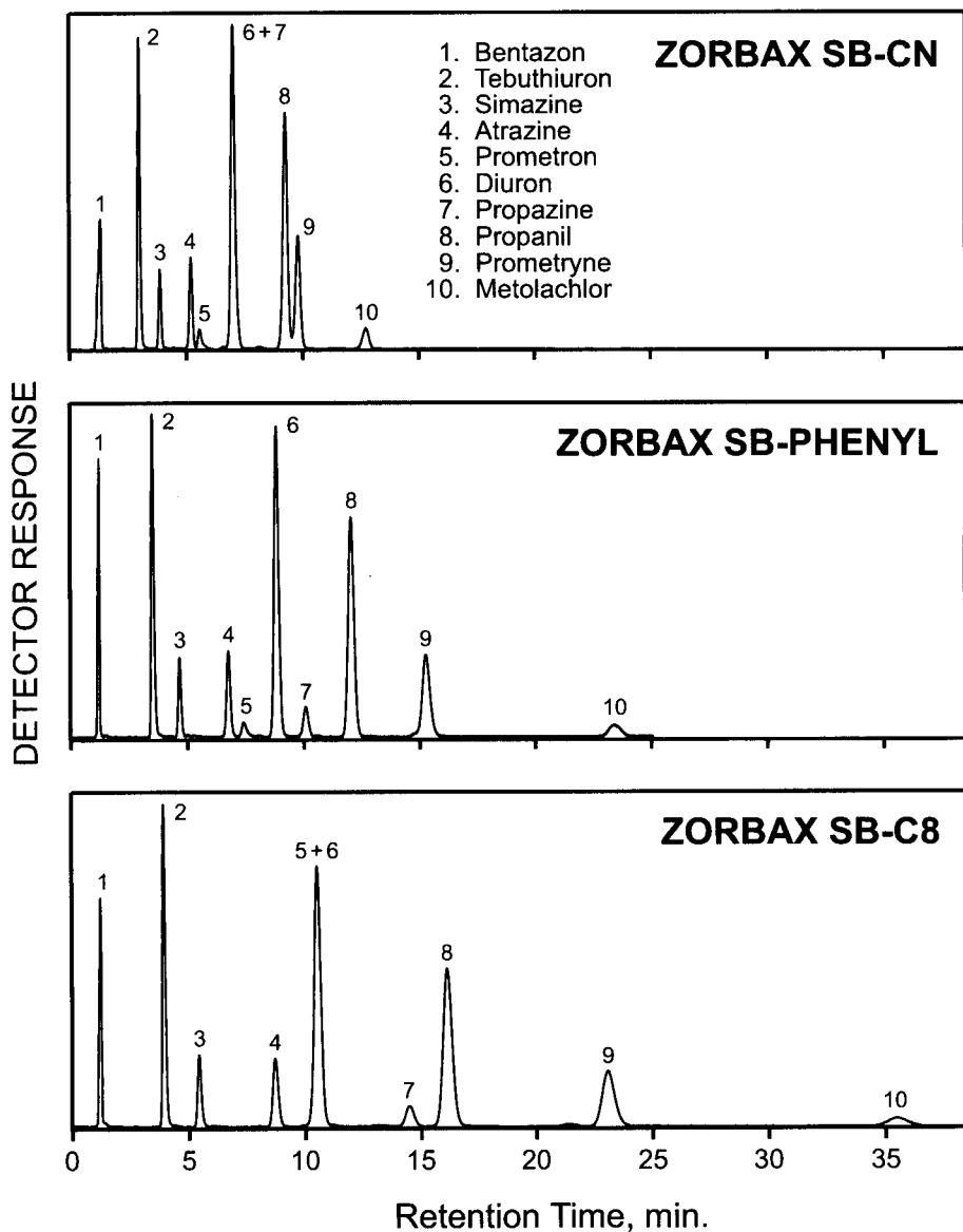
FIGURE 6.11 Effect of column type on selectivity. Columns: Zorbax SB-CN, SB-phenyl, SB-C8, 15 \times 0.46 cm; 35% ACN–65% water; 1.0 mL/min; 22°C; 254-nm UV detection. (Reprinted with permission from Ref. 28.)
