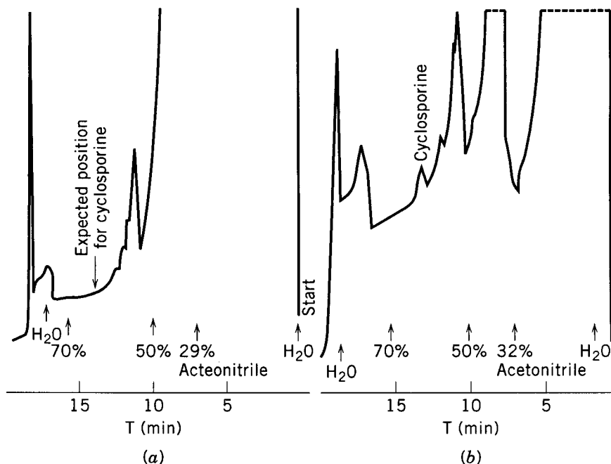
FIGURE 14.15 On-column trace enrichment with a step gradient. Column: 3 \times 0.4 cm, Merck RP-8, 5 \mu\text{m} ; step gradient with acetonitrile and 0.1 M ammonium carbonate; flow rate: 4 \text{ mL/min} ; 70^\circ\text{C} ; detector: UV, 215 \text{ nm} ; sample: 1.78 \text{ mL} ; (a) urine blank; (b) 360 \text{ ppb} cyclosporin (MW 1202) in urine. (Reprinted with permission from Ref. 22.)
