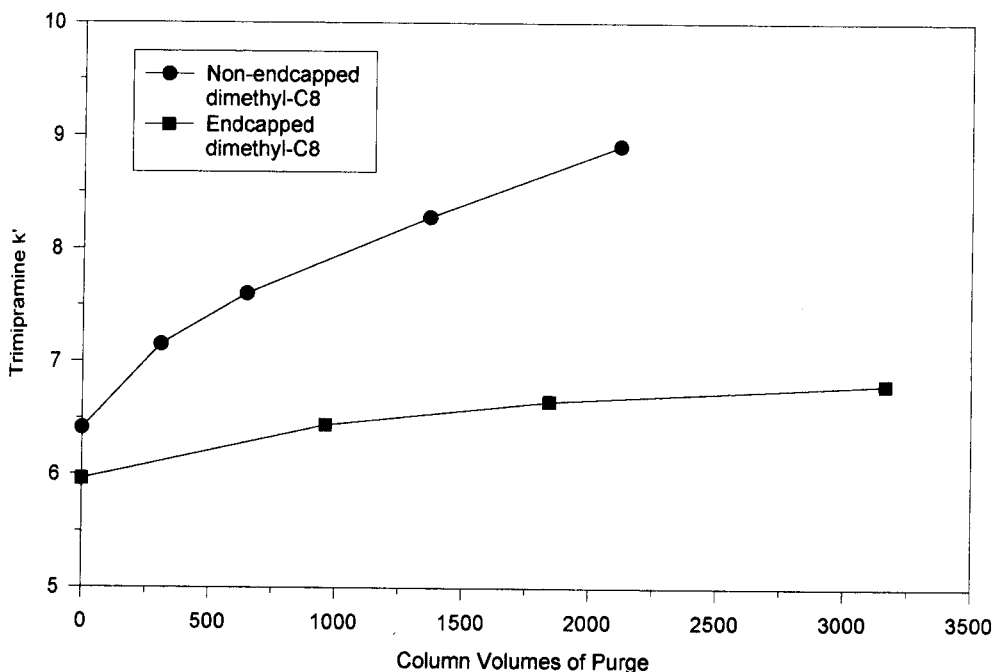
FIGURE 5.15 Comparative stability of non-endcapped and endcapped C 8 columns. Columns: 15 × 0.46 cm, dimethyl-C 8 and double-endcapped dimethyl-C 8 (Zorbax XDB-C8) purge: 20% methanol–80% 0.25 M sodium phosphate buffer, pH 7.0; 60°C; 1.0 mL/min; test: 60% acetonitrile–40% sodium phosphate buffer, 0.01 M, pH 7.0; 1.5 mL/min; 40°C. (Reprinted with permission from Ref. 37.)
