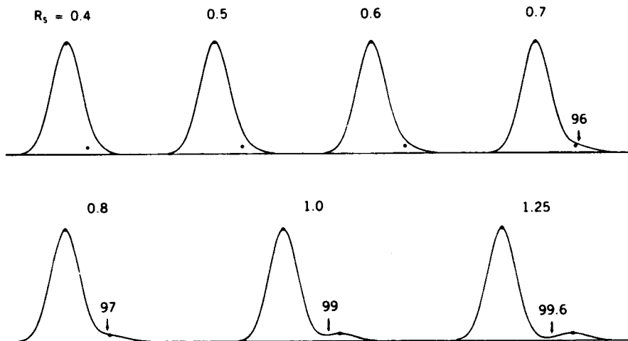
FIGURE I.6 Calculated resolution curves for different values of R_s and band pairs with an area ratio of 16:1. (Reprinted with permission from Ref. 2.)
