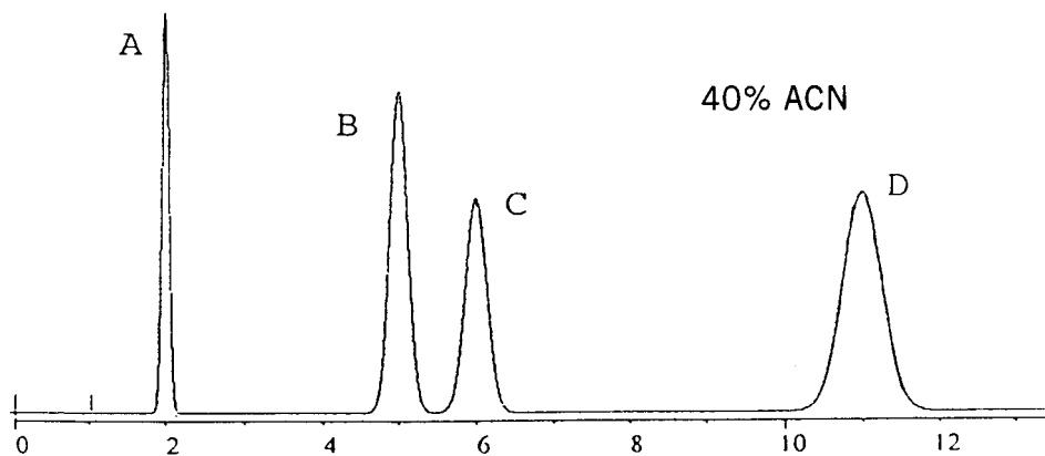
FIGURE 6.2 Effect of a change in percent organic on RPC separation of a hypothetical sample. Conditions: 15 \times 0.46 -cm C_{18} column, 1.5 mL/min flow rate ( t_0 = 1.0 min).
