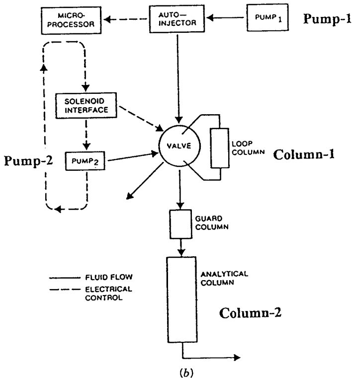
FIGURE 4.16 Column-switching arrangements for (a) removal of protein from plasma samples [76], and (b) removal of hydrophobic late eluters from a cream formulation [77]. See the text for details. (Reprinted with permission from Refs. 76 and 77.)
