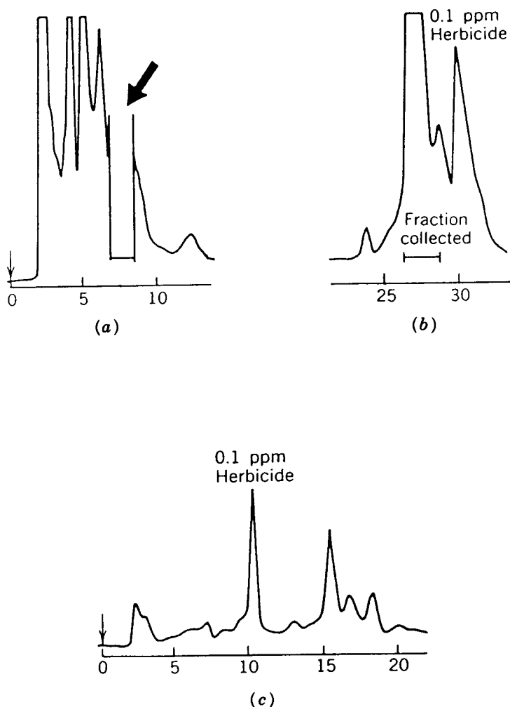
FIGURE 6.26 Separation of a herbicide contained in a green oats extract by sequential separation on a cyano, diol, and silica column. (a) Chromatogram from the cyano column; (b) chromatogram from the diol column; (c) chromatogram from the silica column. See the text for details. (Adapted from Ref. 61.)
