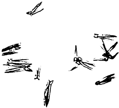
FIG. 3.—Quinidine 1 : 50. Crystals formed with potassium ferrioxalate ( \times 150 ).
