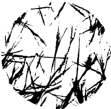
FIG. 5.—Berberine 1 : 500, with hydrochloric acid ( \times 150 ).
