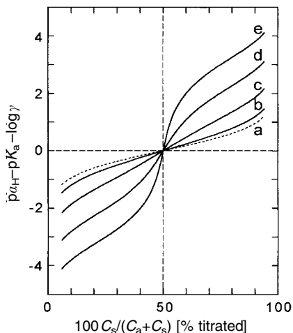
Fig. 3.3 The effect of homoconjugation on the neutralization titration curve of a weak acid HA. Values of K'(\text{HA}_2^-) ( C_a + C_s ): 0 for a, 10 for b, 10^2 for c, 10^3 for d, and 10^4 for e. The original figure in Ref. [11] was modified.
