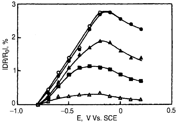
FIGURE 27.28 Potential dependence of reflectivity change for Au electrode in 0.1M \text{HClO}_4 containing NaI. Concentration: \circ , 1.0 \times 10^{-4} M ; \bullet , 5.0 \times 10^{-5} M ; \blacktriangle , 1.0 \times 10^{-5} M ; \blacksquare , 5.0 \times 10^{-6} M ; \triangle , 1.0 \times 10^{-6} M . (From Arai et al., 1997, with permission from Elsevier.)
