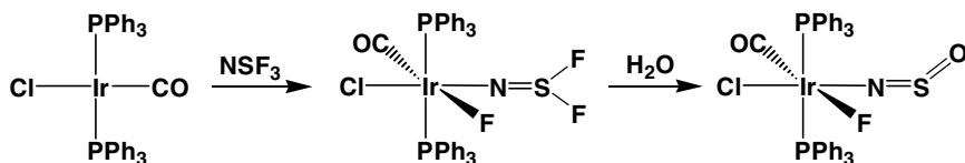
Scheme 7.3 Formation of an [\text{NSF}_2]^- complex
