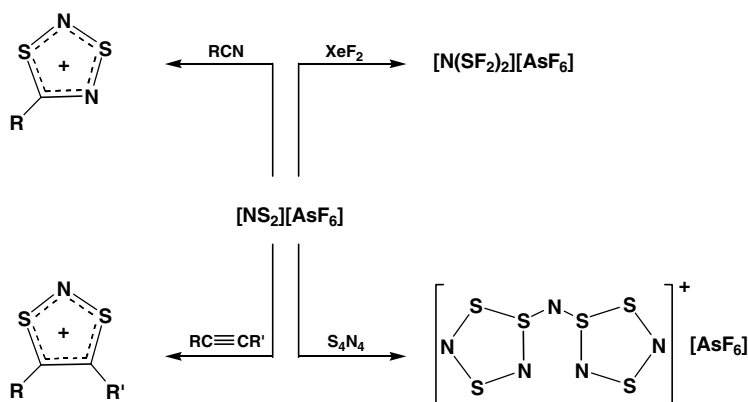
Scheme 5.4 Some cycloaddition reactions of [\text{NS}_2][\text{AsF}_6]
