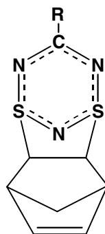
12.10 ( \text{R} = \text{Ph}, \text{CF}_3, \text{NMe}_2 )
