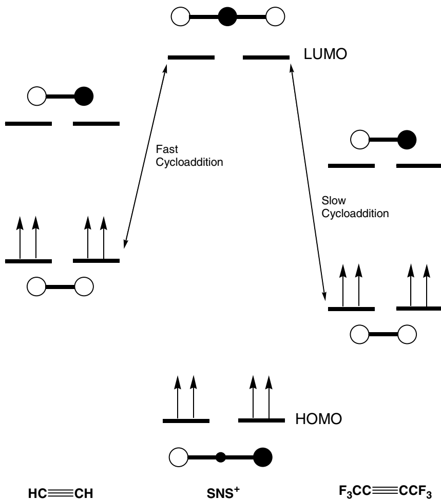
Fig. 4.13 The frontier orbitals of [\text{NS}_2]^+ , \text{HC}\equiv\text{CH} and \text{CF}_3\text{C}\equiv\text{CCF}_3
