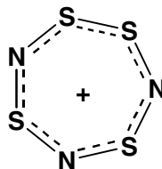
1.16 ( 10\pi e^- )
