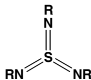
8.5a (R = \text{SiMe}_3 )
