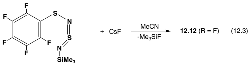
Scheme 12.2 Synthesis of benzodithiadiazines
