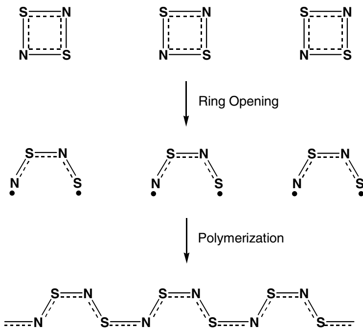
Fig. 14.1 Synthesis and structure of (SN)_x
