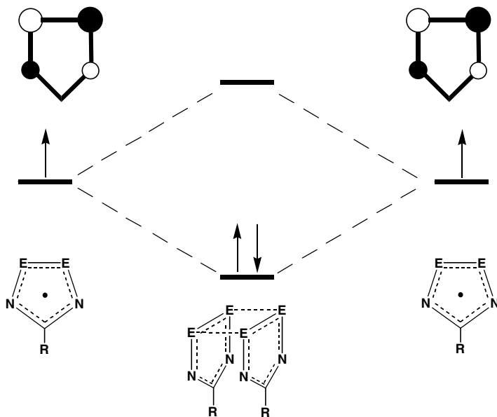
Fig. 4.10 Structure and bonding in (PhCN_2E_2)_2 ( E = S, Se )
