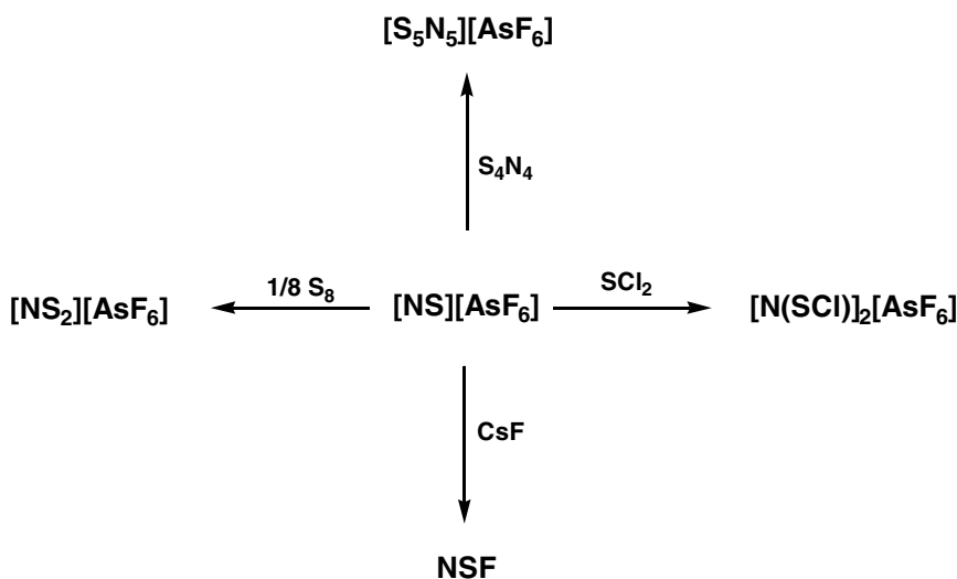
Scheme 5.3 Some reactions of [\text{SN}][\text{AsF}_6]
