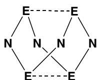
5.6a (E = S)
