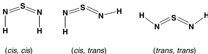
Scheme 5.5 Isomers of sulfur diimide, HNSNH
