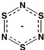
1.15 ( 10\pi e^- )
