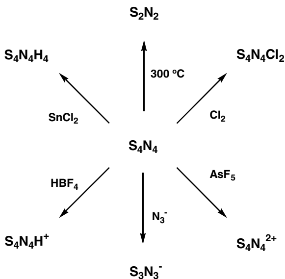
Scheme 5.1 Preparation of S–N rings from S_4N_4
