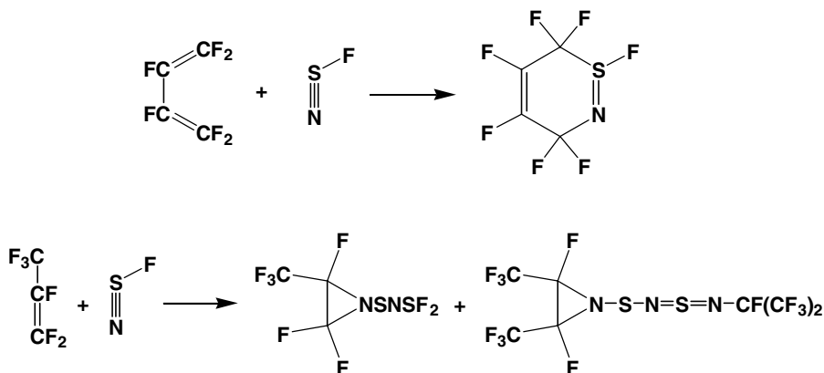
Scheme 8.1 Cycloaddition reactions of NSF
