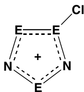
8.11a (E = S)
