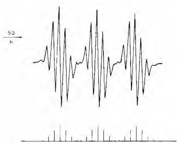
Fig. 3.3 EPR spectrum of [(CF_3S)_2N]^\bullet [Reproduced with permission from J. Am. Chem. Soc. , 105 , 1504 (1983)]
