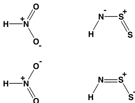
Scheme 10.3 Resonance structures for \text{HNO}_2 and \text{HNS}_2
