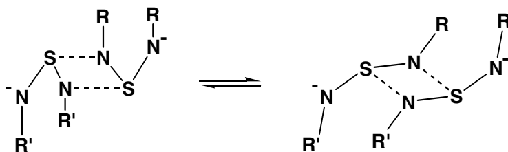
Scheme 10.5 Skeletal scrambling of sulfur diimide radical anions
