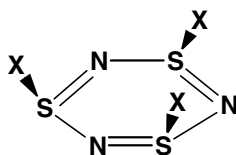
8.12a (X = Cl)
