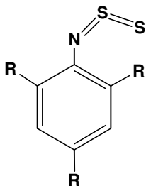
10.3a (R = Me)
