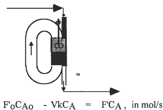
Figure 4.1.2: Dimerization reaction
