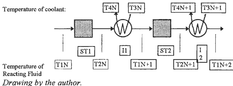
Figure 9.7.1: Staged adiabatic reactor with intercoolers.
