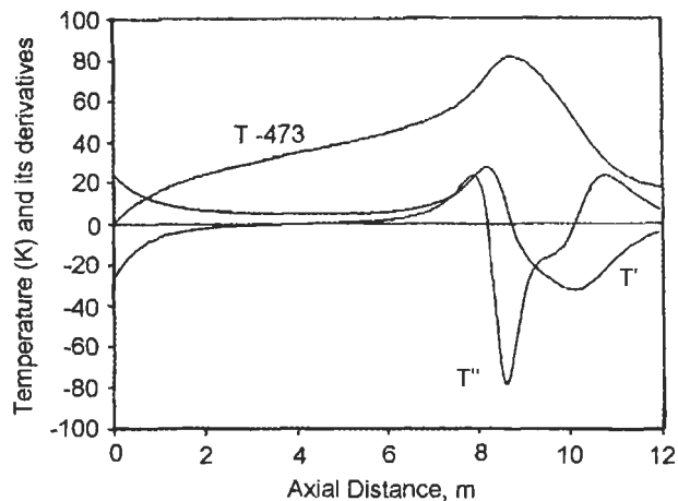
Figure 9.7.3: Plug-flow reactor simulation at T_{\text{wall}} = 485.3\text{K}
