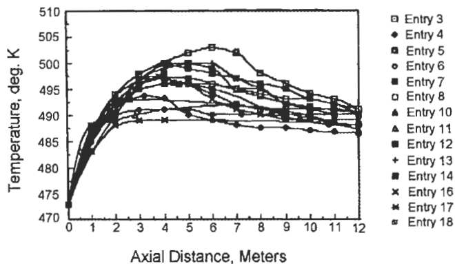
Figure 6.4.6: Models that showed runaway behavior.
