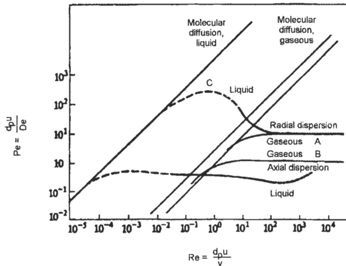
Figure 3.2.1: Mixing in packed beds.
