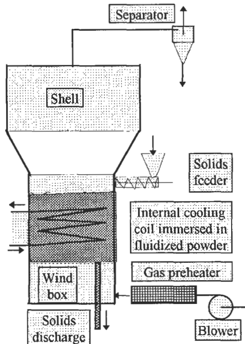
Figure 8.2.4: Fluidized bed reactor
