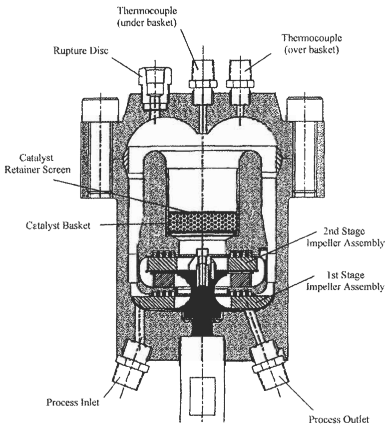
Figure 2.4.4: The ROTOBERTY ® .
