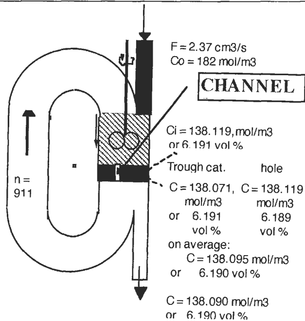
Figure 7.2.3: Channeling in methanol synthesis.
