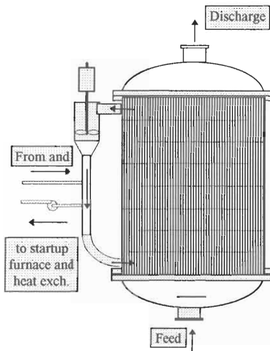
Figure 8.2.1: Tubular reactor.
