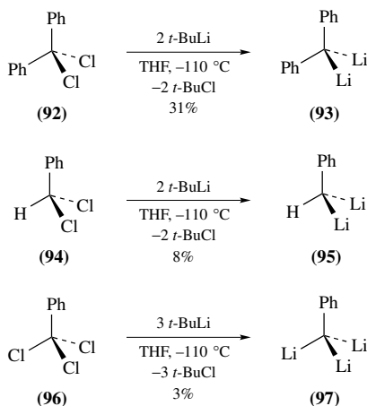
SCHEME 33
