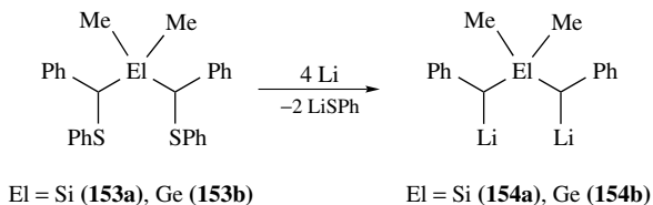
SCHEME 55
