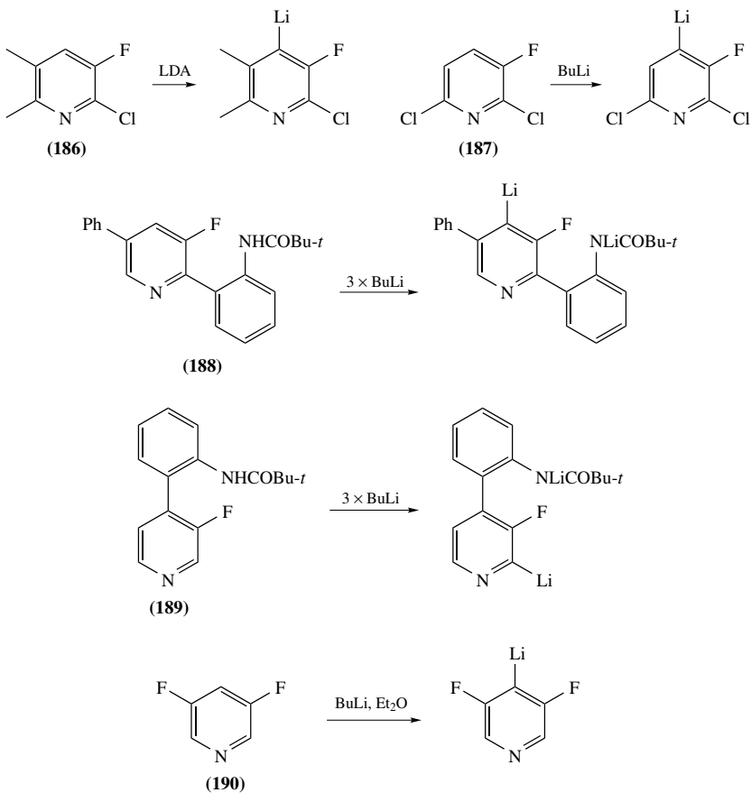
SCHEME 95
