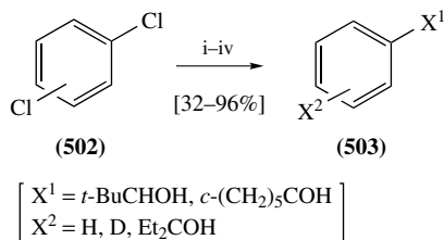
SCHEME 140. Reagents: (i) Li, C 10 H 8 (3%), THF, -78 °C; (ii) E 1 = t -BuCHO, c -(CH 2 ) 2 CO, -78 °C; (iii) E 2 = H 2 O, D 2 O, Et 2 CO, -78 to 20 °C; (iv) H 2 O
