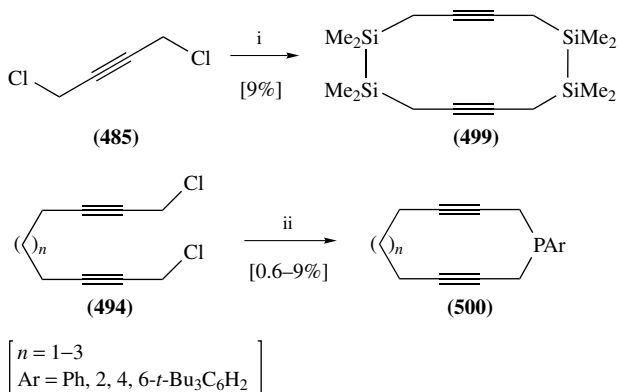
SCHEME 139. Reagents: (i) Li, Ph 2 (20%), (Me 2 ClSi) 2 , THF, -20 °C; (ii) Li, Ph 2 (20%), ArPCl 2 , THF, -20 °C
