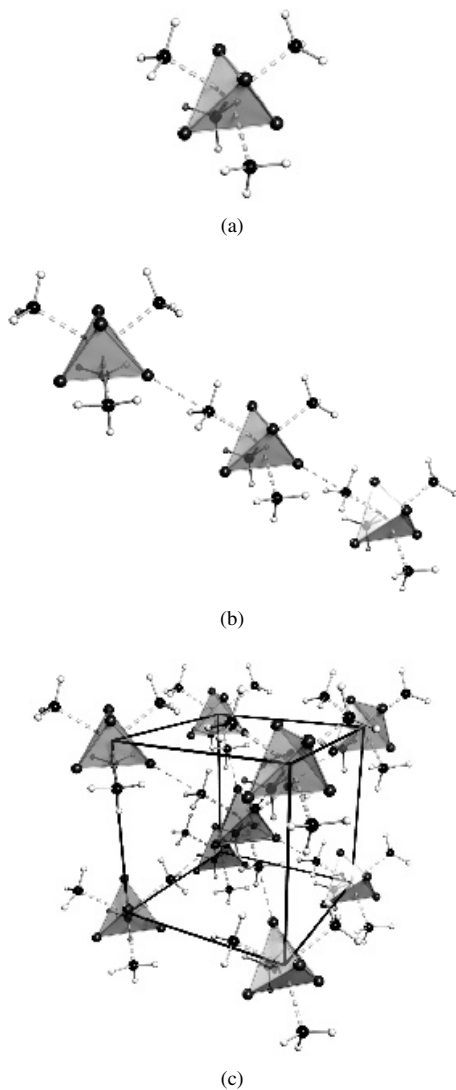
FIGURE 1. Solid-state structure of: (a) [(\text{H}_3\text{CLi})_4] , (b) [\{(\text{H}_3\text{CLi})_4\}_3] and (c) [\{(\text{H}_3\text{CLi})_4\}_\infty] . Reproduced with permission from Ref. 24
