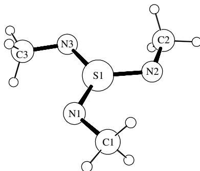
FIGURE 9. DFT-calculated geometry of S(NMe)_3 , resulting in a molecule of C_{3h} symmetry 98 . This structure is known for S(NBu-t)_3 , and S(NSiMe_3)_3 from crystal structure analyses 95,101 . Reproduced with permission from Reference 98. Copyright 1998 Wiley-VCH
