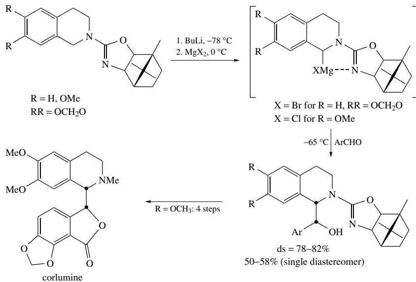
SCHEME 60
