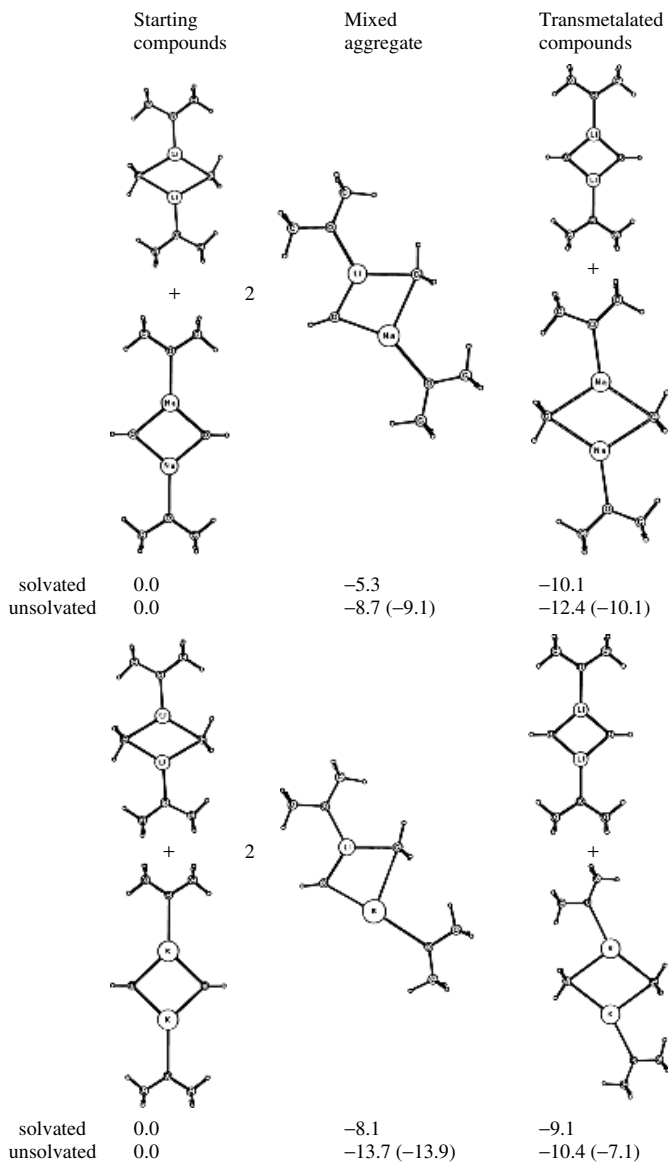
FIGURE 14a. Relative energies for dimethyl ether solvated mixtures [(\text{MOH})_2 / (\text{LiCH}_3)_2] ; M = \text{Na}, \text{K} ] compared to the uncomplexed species at B3LYP basis D //RHF basis A. (D //MP2(full) basis B energies for the unsolvated equilibria are given in parentheses.) Basis A: Li, Na, H, C, N, O, F (6-31+G*) K, Rb, Cs: 9VE-ECP MWB 6s6p1d/4s4p1d; basis B: Li, Na, H, C, N, O, F (6-31++G**), K, Rb, Cs: 9VE-ECP MWB 6s6p2d/5s5p2d; basis D: Li, Na, H, C, O (6-311+G*), K: 9VE-ECP MWB 6s6p2d/5s5p2d. Reprinted with permission from Reference 17. Copyright 1996 American Chemical Society
