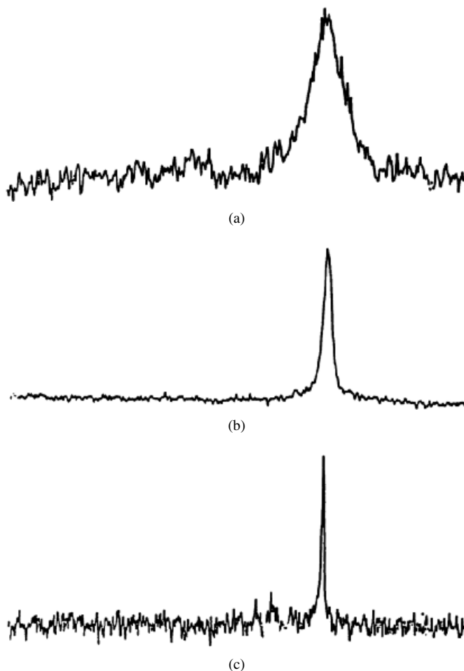
FIGURE 6. The first (proton decoupled) ^{13}\text{C} CP/MAS NMR spectrum of an organolithium spectrum, methyllithium at -150^\circ\text{C} : (a) \text{CH}_3^7\text{Li} , (b) \text{CH}_3^6\text{Li} , (c) \text{CH}_3^6\text{Li} with both ^1\text{H} and ^6\text{Li} high-power decoupling. Reprinted with permission from Reference 95. Copyright 1984 American Chemical Society
