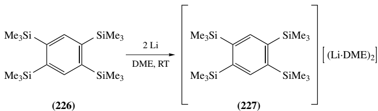
SCHEME 78
