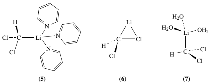
SCHEME 5. Structure of dichloromethyl lithium: X-ray structure analysis of \text{LiCHCl}_2 \cdot 3 pyridine ( 5 ), calculated structure of \text{LiCHCl}_2 ( 6 ), calculated structure of \text{LiCHCl}_2 \cdot 3\text{H}_2\text{O} ( 7 )
