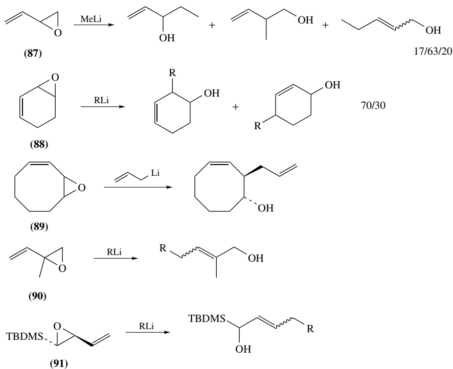
SCHEME 38
