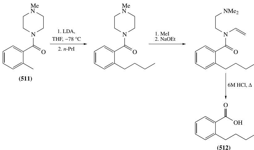
SCHEME 198
