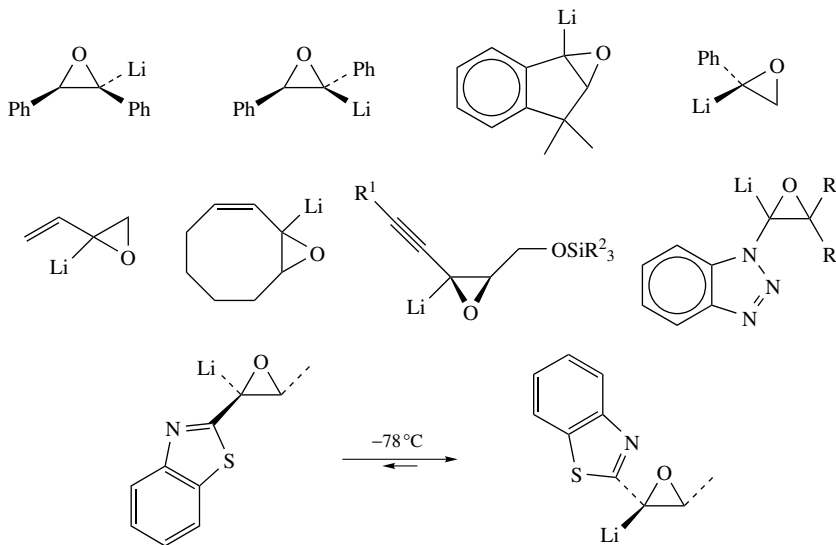
SCHEME 82
