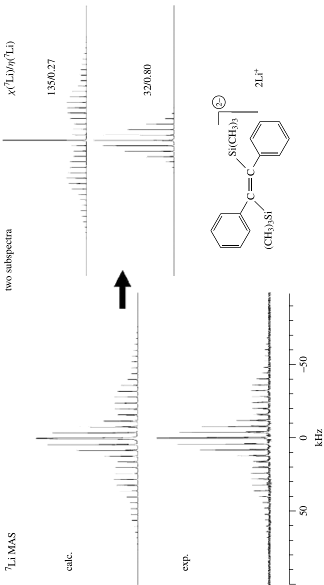
FIGURE 19. Solid state 7 Li MAS spectrum of the dianion formed by Li reduction of ( E )-1,2-diphenyl-1,2-bis(trimethylsilyl)ethene 2,19
