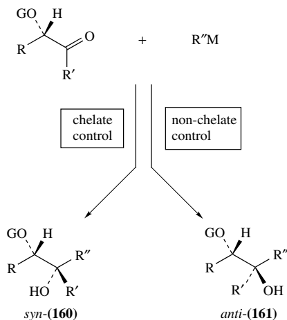
SCHEME 22. Stereochemical outcome of the addition of polar organometallic compounds \text{R}''\text{M} to \alpha -alkoxy aldehydes and ketones (G = protecting group)
