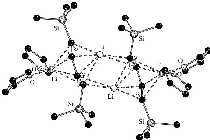
FIGURE 7. Molecular structure of 14 in the solid state
