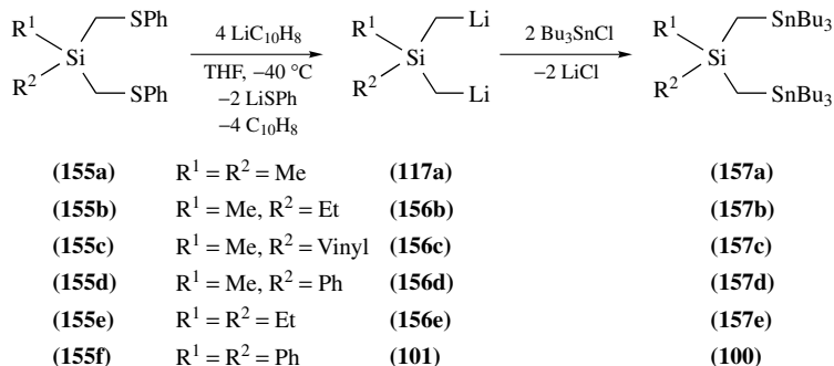
SCHEME 56
