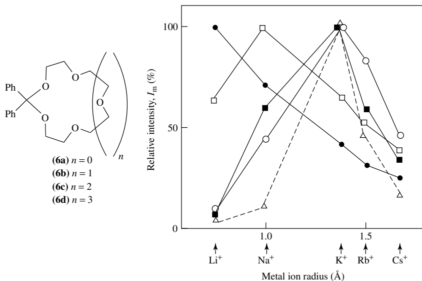
FIGURE 8. Relative intensities of ions corresponding to alkali cationized crown ethers 6a (●), 6b (□), 6c (■), 6d (○) and benzo-18-crown-6, 7 (Δ). Reproduced with permission from Ref. 42
