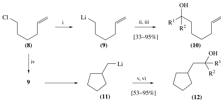
SCHEME 4. Reagents: (i) Li, DTBB (10%), THF, -78^{\circ}\text{C} ; (ii) \text{B}(\text{OEt})_3 , -78 to 25^{\circ}\text{C} ; (iii) \text{HOCH}_2\text{-CMe}_2\text{CH}_2\text{OH} , THF, 25^{\circ}\text{C}
