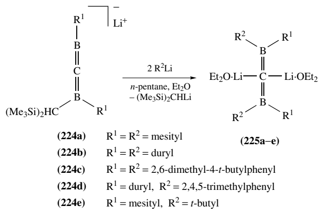
SCHEME 77
