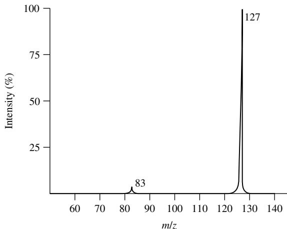
FIGURE 1. CID spectrum of \text{LiC}_6\text{H}_4\text{CO}_2^- ( m/z 127). The fragment ion at m/z 83 corresponds to \text{C}_6\text{H}_5\text{Li}^- . Reproduced with permission from Ref. 15
