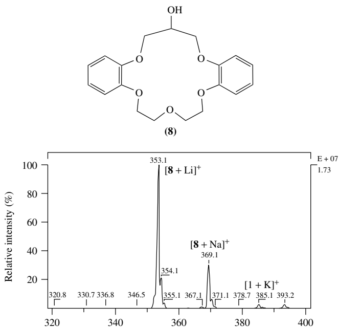
FIGURE 9. ESI mass spectrum of compound 8 with LiCl 43
