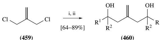
(459)
