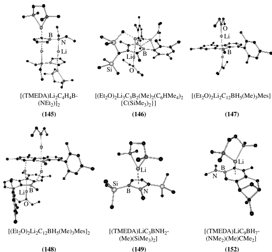
FIGURE 27. Solid-state structures of lithium organics with heterocyclic perimeters containing boron as a group 13 element
