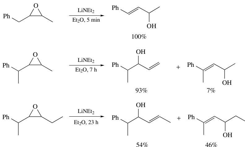
SCHEME 20
