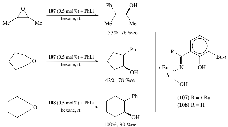
SCHEME 48
