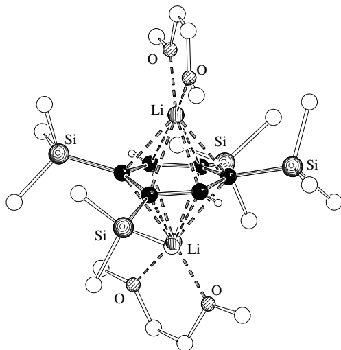
FIGURE 29. Molecular structure of 227 in the solid state
