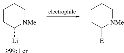
SCHEME 9
