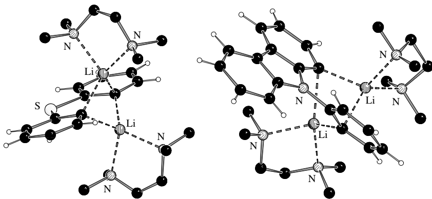
FIGURE 10. Molecular structures of 26 and 27 in the solid state
