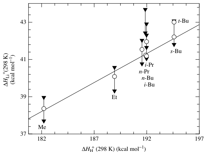
FIGURE 2. LCA vs PA at 298 K (in \text{kcal mol}^{-1} ) 26 . Open circles show CID results from Reference 26 and inverted triangles show a range of values measured with an FT-ICR and cited in Reference 26
