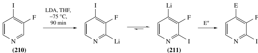
SCHEME 102
