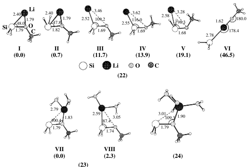
FIGURE 20. Optimized geometries and relative energies (kcal mol -1 ) for (\text{MeO})_2\text{H}_2\text{SiLi} ( 22 ), (\text{MeO})_2\text{H}_2\text{SiLi}(\text{H}_2\text{O})_2 ( 23 ) at MP2/HF/6-31G** and optimized geometry for (\text{MeO})_2\text{H}_2\text{SiLi}(\text{H}_2\text{O})_3 ( 24 ) at HF/6-31G**. Bond lengths are in angstroms, bond angles in degrees. Reprinted with permission from Reference 26. Copyright 1998 American Chemical Society
