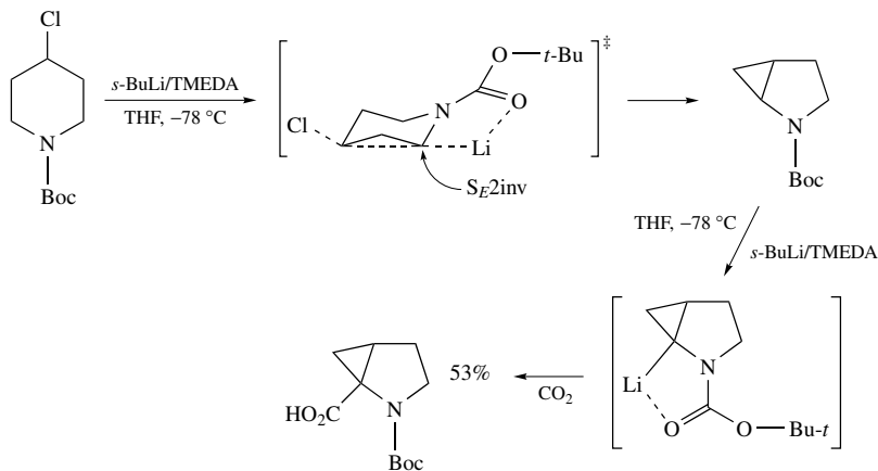
SCHEME 31
