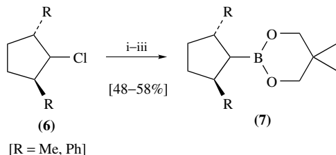
SCHEME 4. Reagents: (i) Li, DTBB (10%), THF, -78^{\circ}\text{C} ; (ii) \text{B}(\text{OEt})_3 , -78 to 25^{\circ}\text{C} ; (iii) \text{HOCH}_2\text{-CMe}_2\text{CH}_2\text{OH} , THF, 25^{\circ}\text{C}
