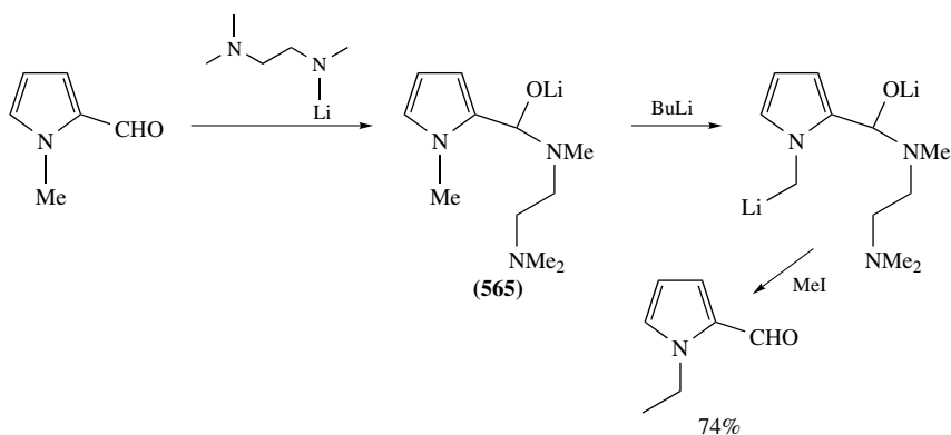
SCHEME 228
