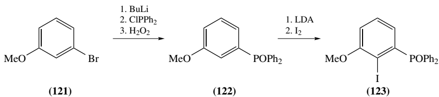
SCHEME 53
