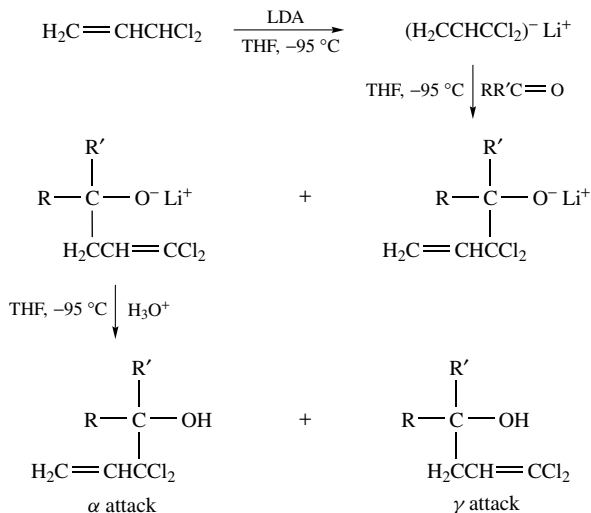
SCHEME 2. The \alpha - and \gamma -selectivity in the addition reaction of carbonyl electrophiles to gem -dichloroallyl anion
