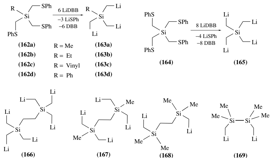
SCHEME 59
