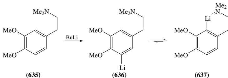
SCHEME 247
