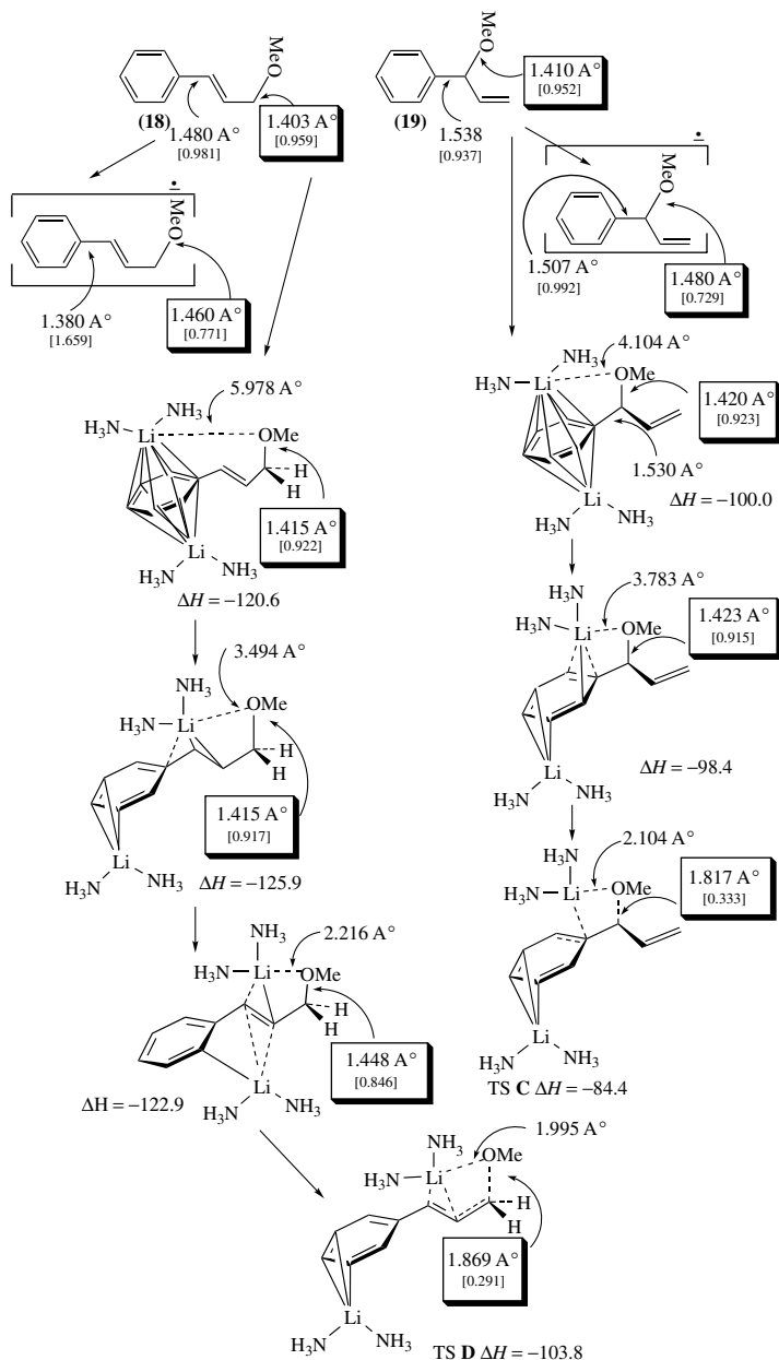
FIGURE 18b. MNDO-determined structures of intermediates and transition states for the cleavage of cinnamyl and phenylpropenyl ethers 18 and 19 , through dianion-radical routes involving contact ion pairs (CIP) and isolated ion pairs (IIP). All energies are in kcal mol -1 . Geometrical features relevant to haptomeric activation are shown: (1) C-OMe bond length and bond order (in brackets), (2) Li-OMe distance and (3) enthalpy of formation. Reprinted with permission from Reference 22. Copyright 1996 American Chemical Society
