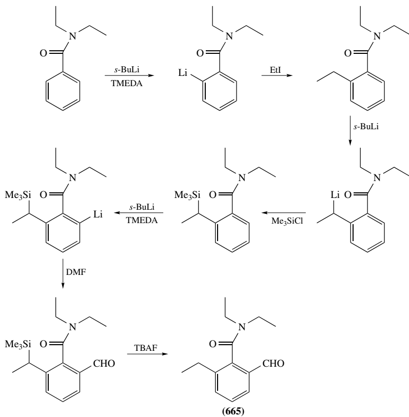
SCHEME 257
