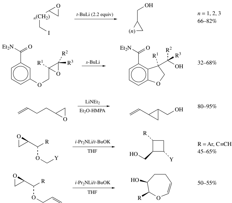
SCHEME 37
