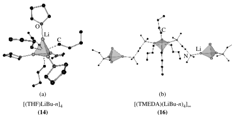
FIGURE 10. Solid-state structures of donor-base-coordinated [\textit{n}\text{-BuLi}]_4 tetramers
