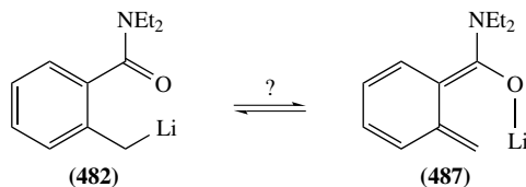
SCHEME 191
