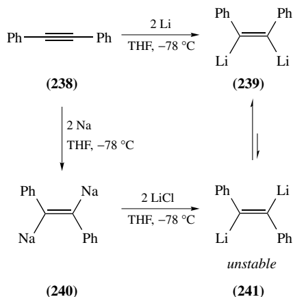
SCHEME 84
