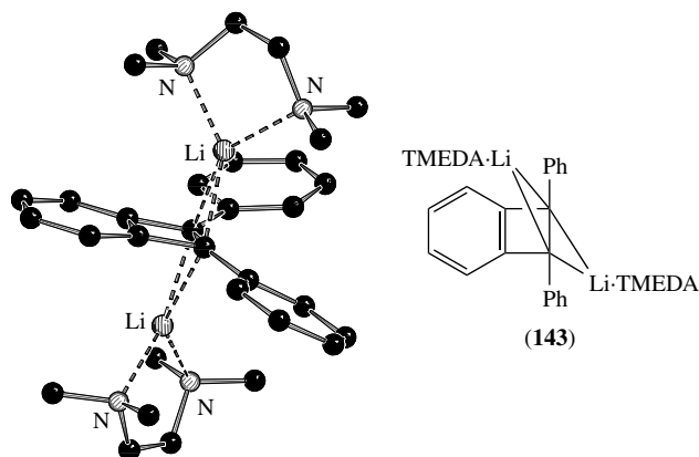
FIGURE 17. Molecular structure of 143 in the solid state and Lewis formula
