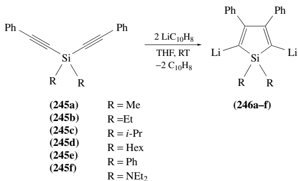
SCHEME 86
