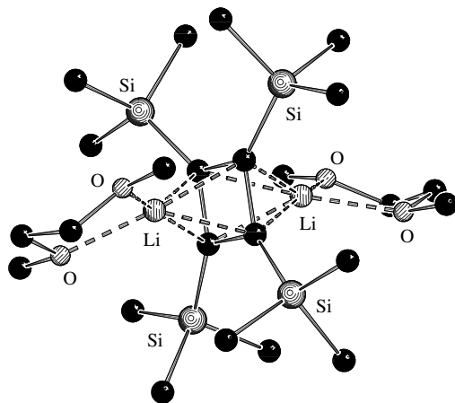
FIGURE 18. Molecular structure of 142a in the solid state
