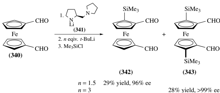
SCHEME 151
