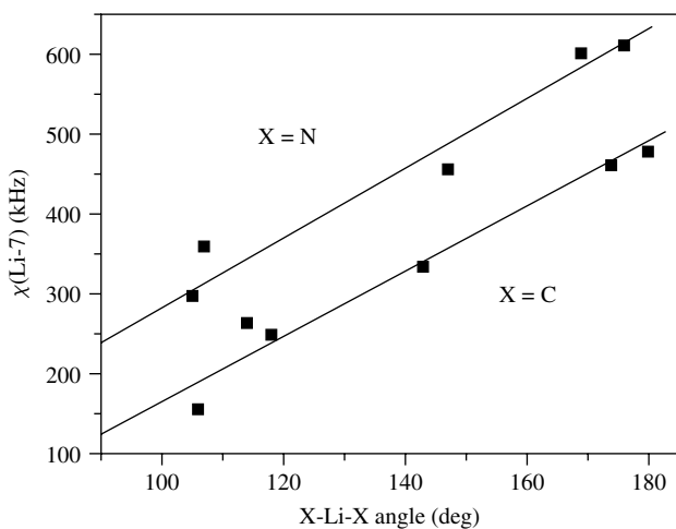
FIGURE 18. \chi(^7\text{Li}) vs. the X–Li–X angle in lithium amides (X = N) and organolithium compounds (X = C)
