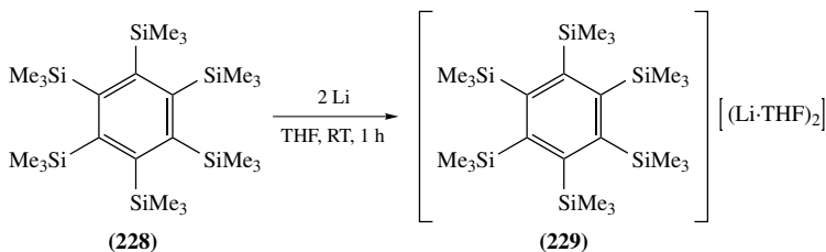
SCHEME 79
