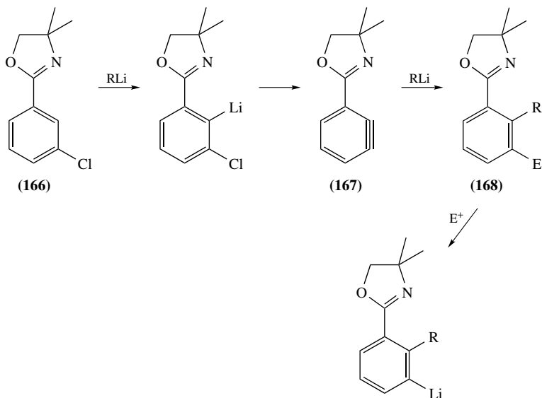
SCHEME 84
