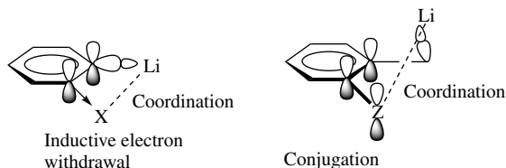
SCHEME 187
