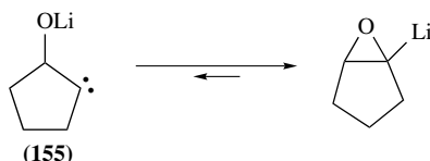
SCHEME 66
