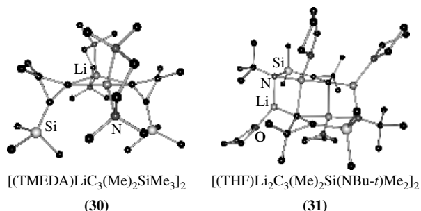
FIGURE 12. Solid-state structures of monolithium and dilithium cyclopropenyl dimers. While in-plane dimerization is hampered by the donor-base in 30 , side-arm donation promotes a planar R 1 R 2 CLi 2 -fragment in 31
