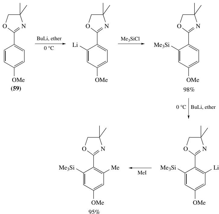
SCHEME 29
