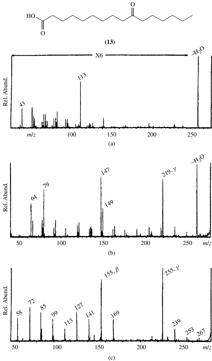
FIGURE 13. High-energy CID spectra of (a) MH^+ , (b) [M + Li]^+ and (c) [M - H + 2Li]^+ ions of 10-oxohexadecanoic acid 13 . Reproduced with permission from Ref. 63
