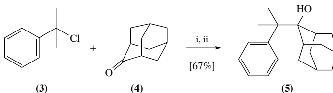
SCHEME 3. Reagents: (i) Li, DTBB (1–3%), THF, 0 °C; (ii) NH 4 Cl–H 2 O
