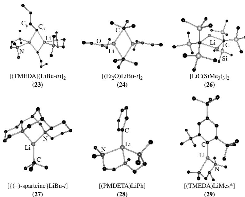
FIGURE 11. Solid-state structures of donor-base-coordinated dimers and monomers
