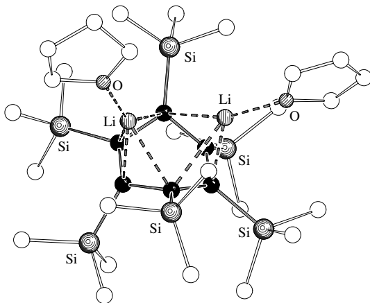
FIGURE 30. Molecular structure of 229 in the solid state
