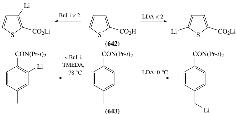
SCHEME 249
