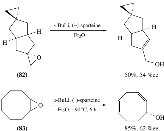
SCHEME 33
