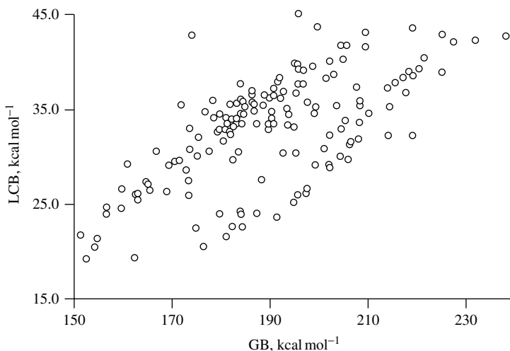
FIGURE 6. Correlation between experimental LCBs and gas-phase basicities towards the proton (GB). Reproduced with permission from Ref. 34
