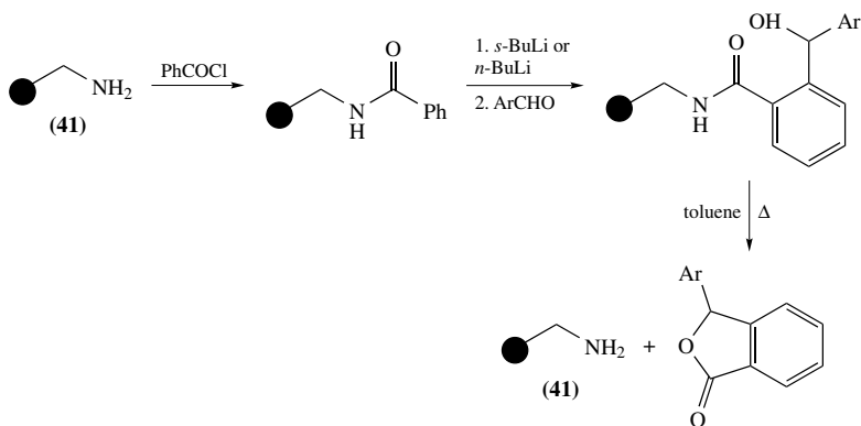
SCHEME 21
