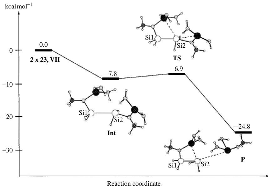
FIGURE 22. Potential-energy profile for the self-condensation reaction of lithium(alkoxy)silylenoid 23, VII (see Figure 20) at MP2//HF/6-31G**. Reprinted with permission from Reference 26. Copyright 1998 American Chemical Society
