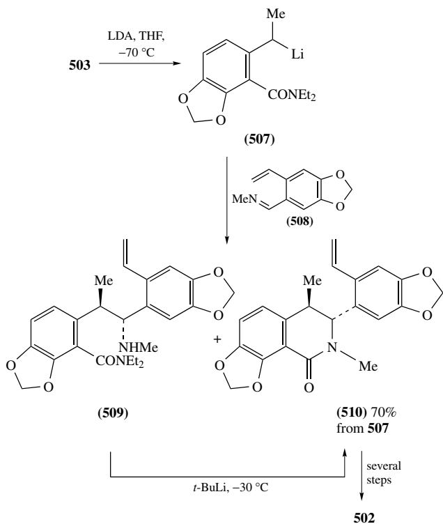
SCHEME 197
