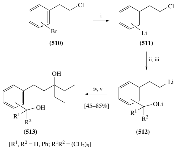
SCHEME 142. Reagents: (i) t -BuLi, THF, -100^\circ\text{C} ; (ii) \text{R}^1\text{R}^2\text{CO} = \text{PhCHO} , c -( \text{CH}_2 ) 2 CO, -100^\circ\text{C} ; (iii) Li, \text{C}_{10}\text{H}_8 (8%), THF, -78^\circ\text{C} ; (iv) \text{Et}_2\text{CO} , -78 to 20^\circ\text{C} ; (v) \text{H}_2\text{O}
