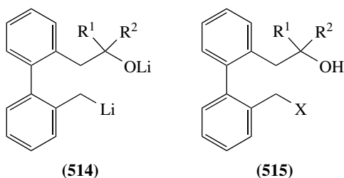
SCHEME 142. Reagents: (i) t -BuLi, THF, -100^\circ\text{C} ; (ii) \text{R}^1\text{R}^2\text{CO} = \text{PhCHO} , c -( \text{CH}_2 ) 2 CO, -100^\circ\text{C} ; (iii) Li, \text{C}_{10}\text{H}_8 (8%), THF, -78^\circ\text{C} ; (iv) \text{Et}_2\text{CO} , -78 to 20^\circ\text{C} ; (v) \text{H}_2\text{O}
