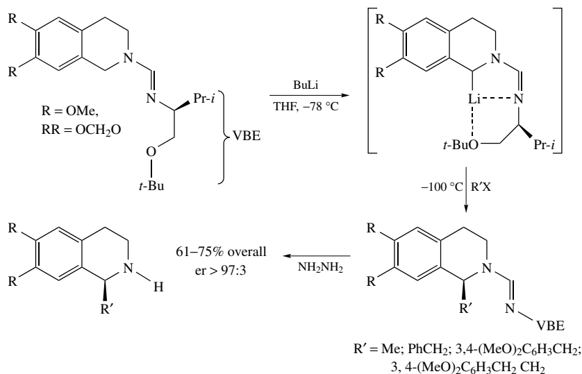
SCHEME 55
