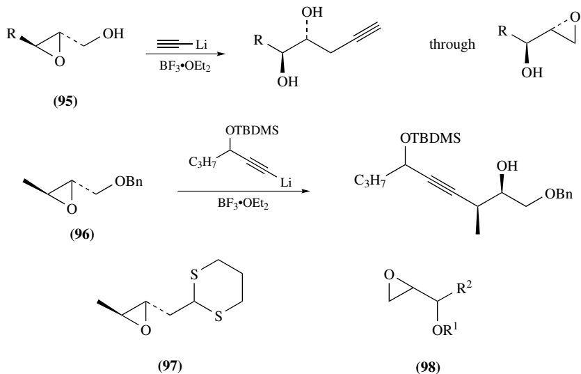
SCHEME 43
