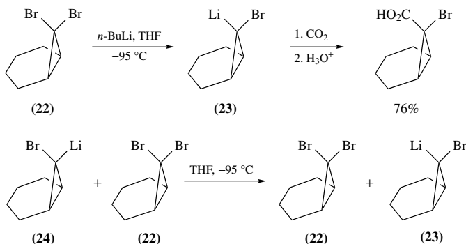
SCHEME 8. Diastereoselective bromine–lithium exchange reaction in dibromonorcaradiene 22
