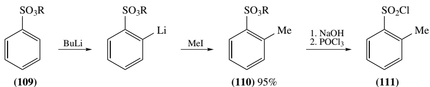
SCHEME 48
