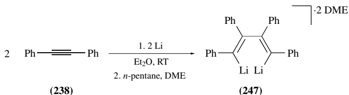
SCHEME 87
