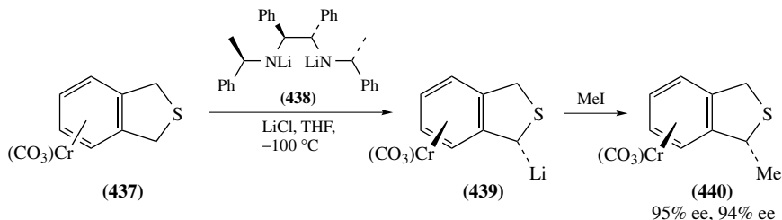
SCHEME 177
