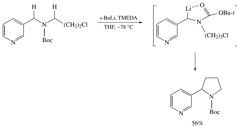
SCHEME 48
