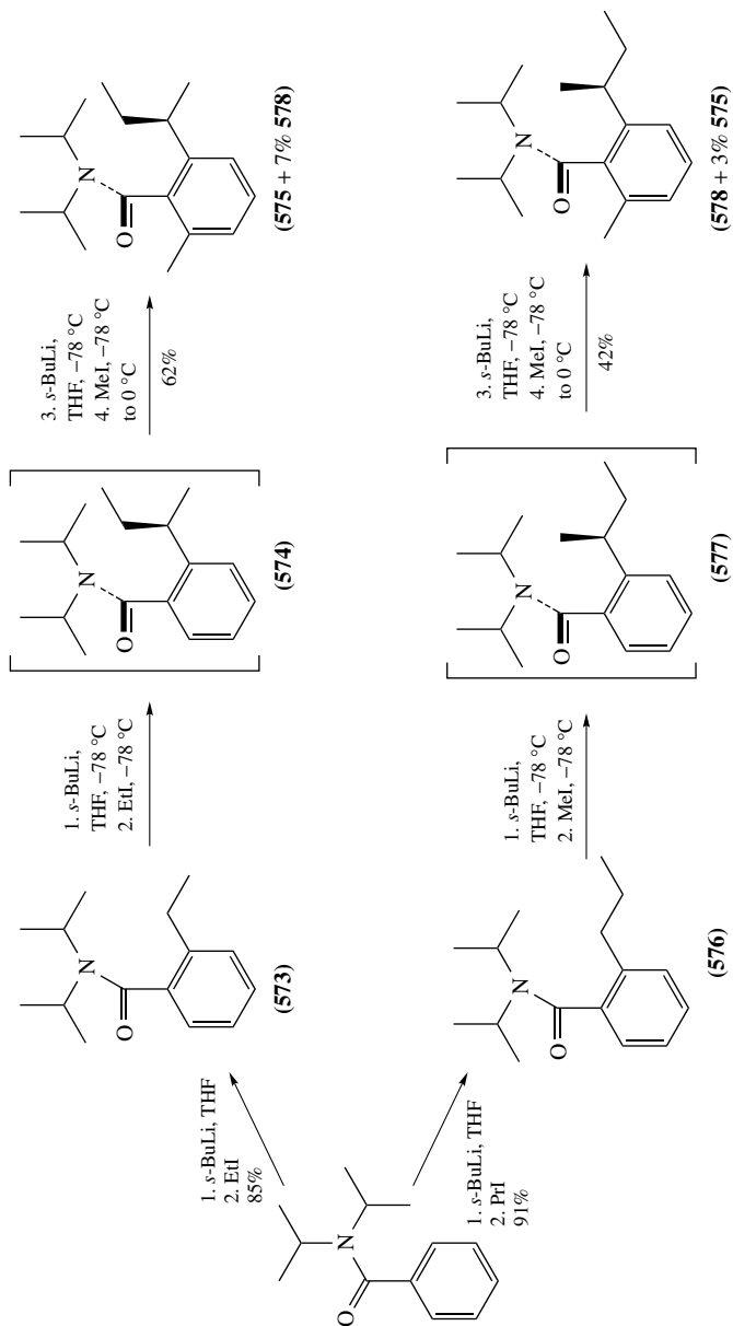
SCHEME 231
