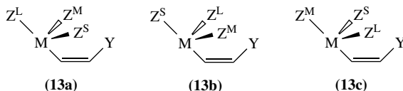
FIGURE 1. The three possible conformations of a cis -1,2-disubstituted ethene having a spherical reaction site in contact with a tetrahedral substituent consisting of a central atom M bearing large ( \text{Z}^{\text{L}} ), medium ( \text{Z}^{\text{M}} ) and small ( \text{Z}^{\text{S}} ) sized groups. The energies of the conformations are 13a , lowest, and 13c , highest. The same types of conformation occur in other 1,2- and 1,3-disubstituted systems in which substituent and reaction site are in contact
