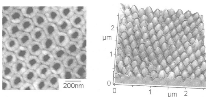
Fig. 2.20. AFM pictures of (left) a porous crystal made from a core-shell latex: the crystalline lattice of the \text{SiO}_2 appears grey while the nanopores are black; (right) surface of a dried core-shell latex
