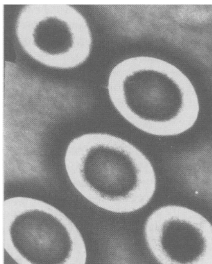
Fig. 3.5. TEM image of a cut through a SAN matrix with incorporated core/double shell particles. dark core : PMMA; bright area : PBA shell; diameter of the particles of the first shell: about 220 nm; the second PMMA shell is compatible with SAN matrix, therefore the contrast is very weak (details see references at the end of Chap. 3)
