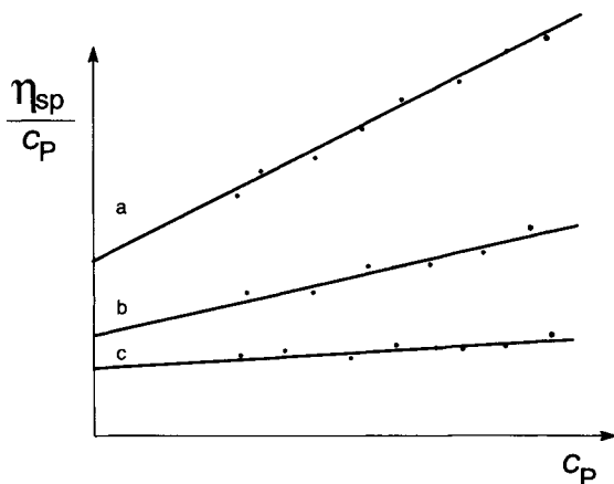
Fig. 2.13. Graphical evaluation of the limiting viscosity number (intrinsic viscosity) from viscosity measurements at different concentrations for a high-molecular-weight, b a medium-molecular-weight, and c a low-molecular-weight polymer sample
