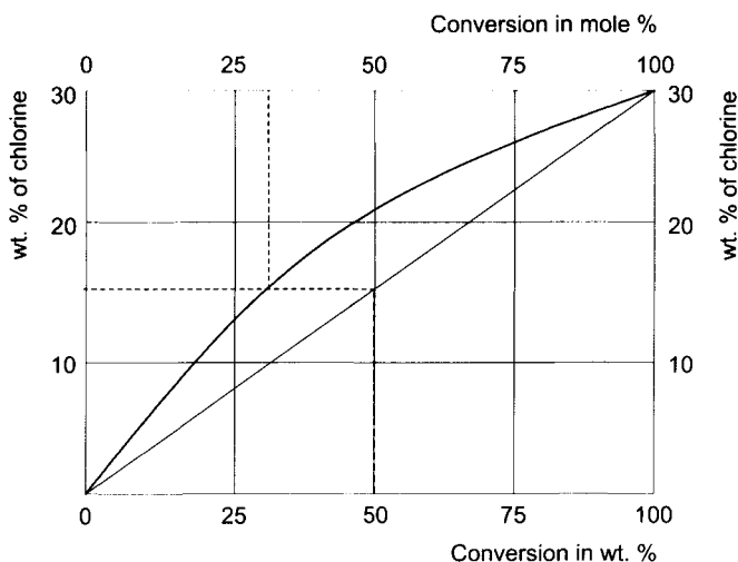
Fig. 5.1. Example of graphical determination of wt% conversion ( lower line ) and mol% conversion ( upper line ) from chlorine content in the esterification of poly(vinyl alcohol) with chloroacetic acid to give (C_4H_5ClO_2)_n at 100% conversion (29.5 wt% of chlorine). Dashed lines indicate values corresponding to an observed composition of 14.75 wt% of chlorine
