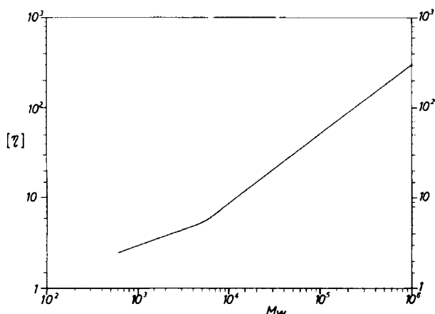
Fig. 2.14. Relation between viscosity and molecular weight for polystyrene in benzene at 20 °C
