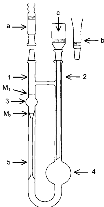
Fig. 2.15a. Ostwald viscometer: Total length: 25 cm; capillary length: 10 cm; bulb 3: diameter 1.3 cm, bulb 4: diameter 2.2 cm, filling level: 2 or 3 ml, flow volume: 0.5 ml; a , b : head pieces; c : sintered glass filter for filtration of solvent and polymer solution
