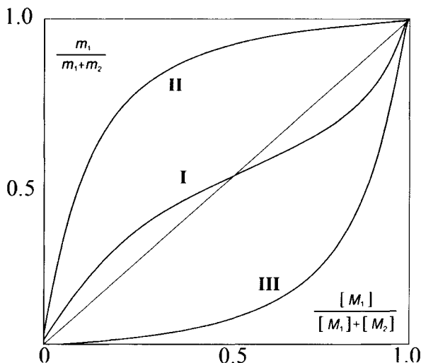
Fig. 3.4. Copolymerization diagram for the system styrene ( M_1 )/methyl methacrylate ( M_2 ). I: radical copolymerization at 60 °C; r_1 = 0.52 , r_2 = 0.46 ; II: cationic copolymerization initiated by \text{SnBr}_4 at 25 °C; r_1 = 10.5 , r_2 = 0.1 ; III: anionic copolymerization initiated by Na in liquid \text{NH}_3 at -50 °C; r_1 = 0.12 , r_2 = 6.4
