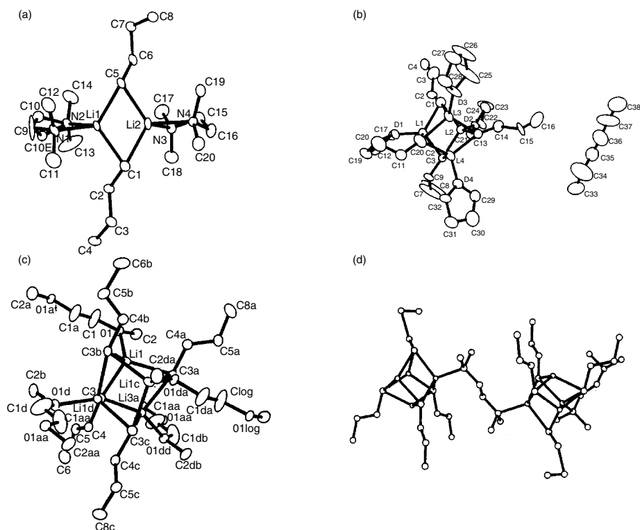
Fig. 6.2. Crystal structures of n -butyllithium: (a) [(n\text{-BuLi-TMEDA})_2] ; (b) [(n\text{-BuLi-THF})_4\text{hexane}] ; (c) [(n\text{-BuLi-DME})_4] ; (d) [(n\text{-BuLi})_4\text{.TMEDA}] . Reproduced from J. Am. Chem. Soc. , 115 , 1568, 1573 (1993), by permission of the American Chemical Society.
