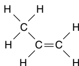
propene (propylene)
