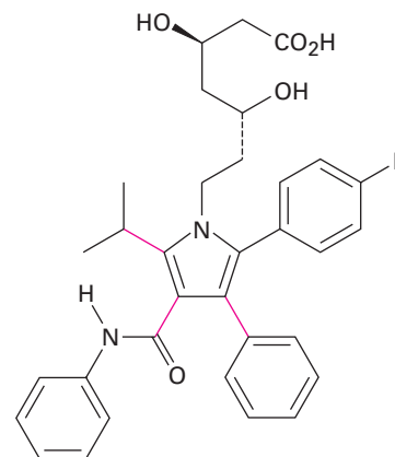
Atorvastatin (Lipitor)
