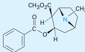
Cocaine
