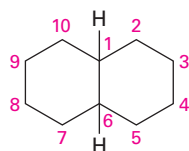
Decalin—two fused cyclohexane rings
