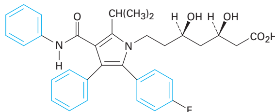
Atorvastatin (Lipitor)
