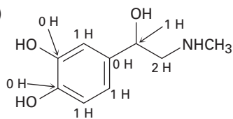
Adrenaline— C_9H_{13}NO_3
