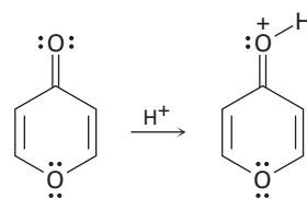
4-Pyrone
