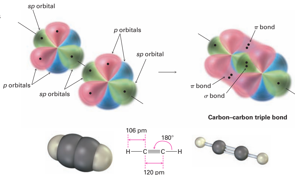
Figure 1.16 The structure of acetylene. The two carbon atoms are joined by one sp-sp \sigma bond and two p-p \pi bonds.
