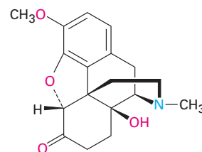
Oxycodone (OxyContin)
