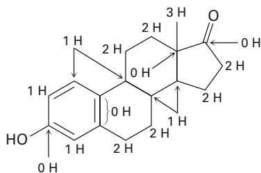
Estrone— C_{18}H_{22}O_2
