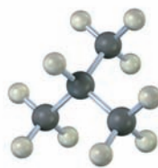
\begin{array}{c} \text{CH}_3 \\ | \\ \text{CH}_3\text{CHCH}_3 \end{array}
