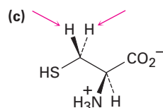
Cysteine
