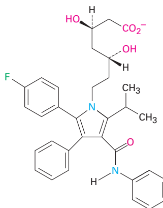
Atorvastatin (Lipitor)
