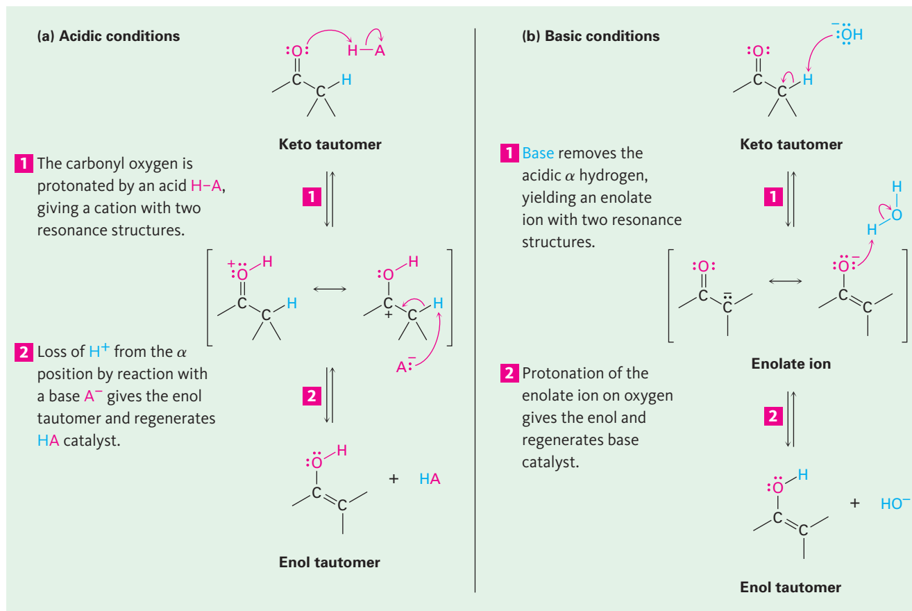
Figure 22.1 | MECHANISM
