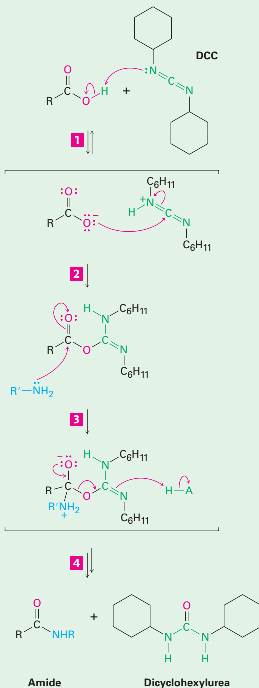
Figure 21.5 | MECHANISM
