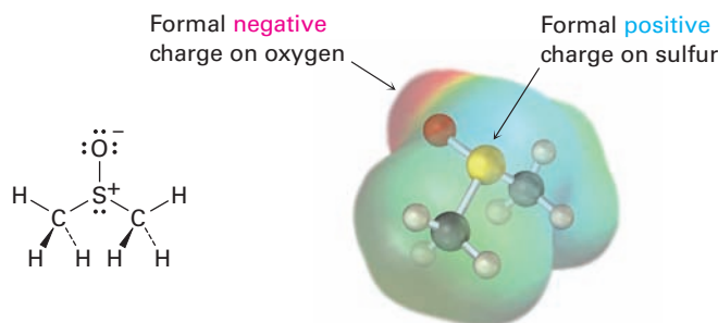
Dimethyl sulfoxide
