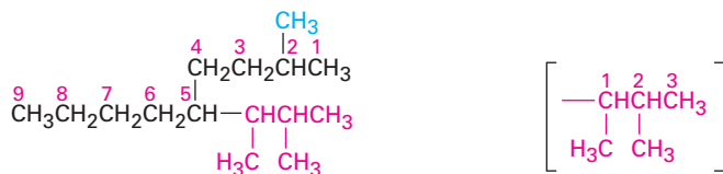
5-(1,2-Dimethylpropyl)-2-methylnonane
