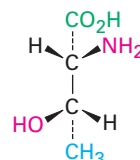
2R,3S-2-Amino-3-hydroxybutanoic acid
