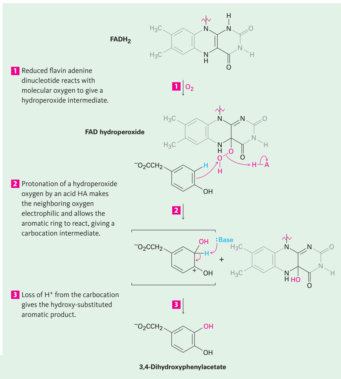
Figure 16.6 | MECHANISM
