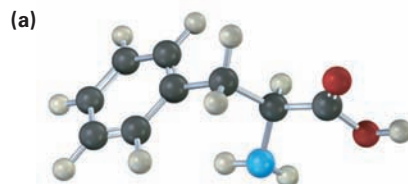
Phenylalanine
