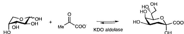
Scheme 6 Reversible aldol addition reaction catalyzed by KDO aldolase.
