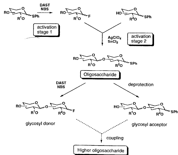
Scheme 9 The two-stage activation procedure for glycoside bond formation [23].
