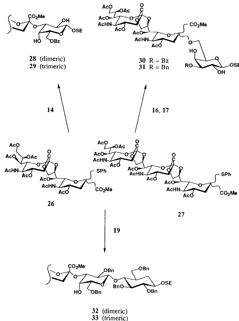
Figure 3 An efficient regio and \alpha -stereoselective synthesis of oligo-sialyl glycosides.
