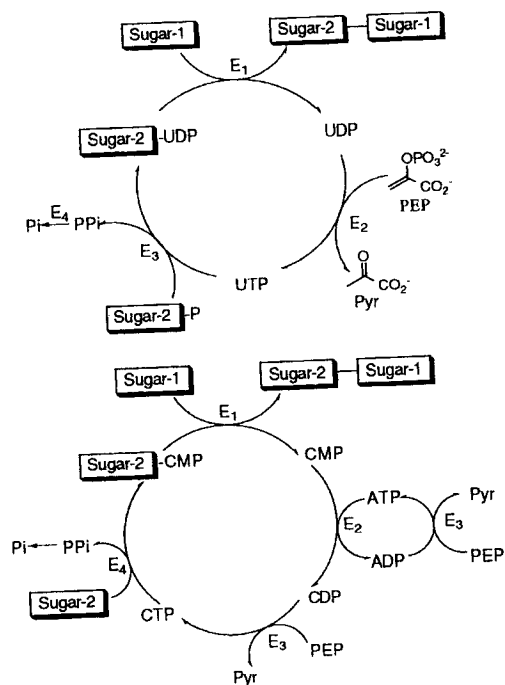
Figure 4 (a) Regeneration systems for UDP-sugar cofactors. E 1 , glycosyltransferase; E 2 , pyruvate kinase; E 3 , UDP-sugar pyrophosphorylase; E 4 , pyrophosphatase. (b) Regeneration systems for CMP-sugar cofactors. E 1 , glycosyltransferase; E 2 , myokinase; E 3 , pyruvate kinase; E 4 , CMP-sugar synthetase.
