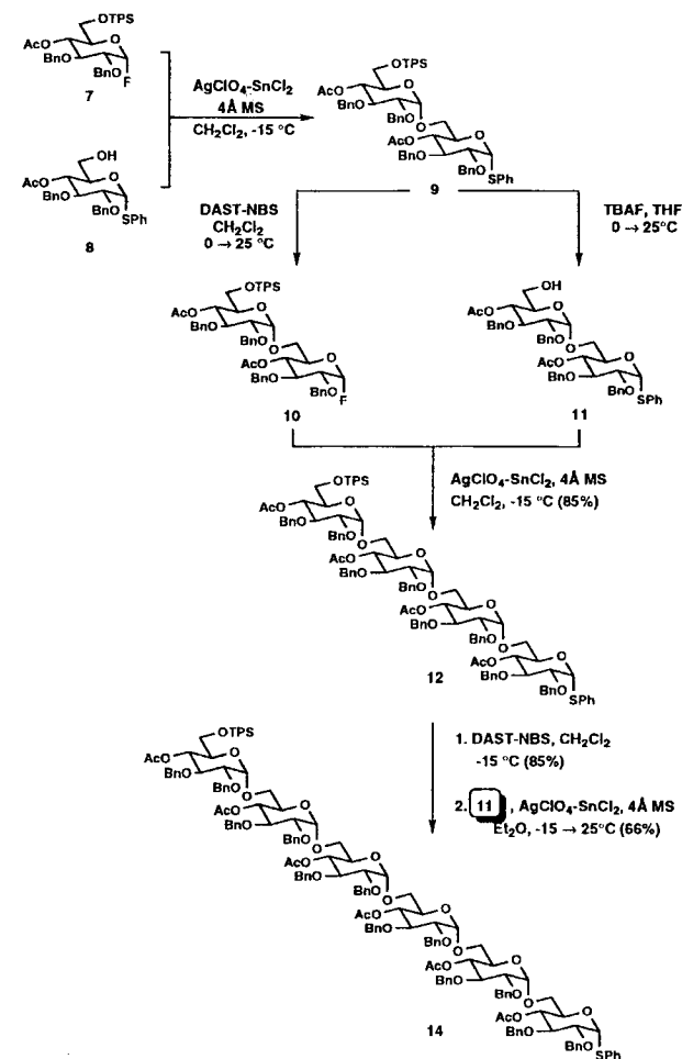
Scheme 11 Synthesis of hexasaccharide 14 [23].
