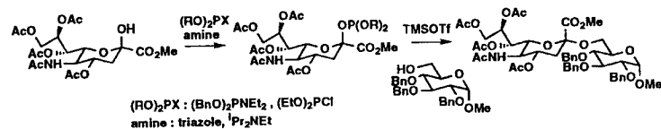
Scheme 6 Phosphite-based glycosidation method [18,19].
