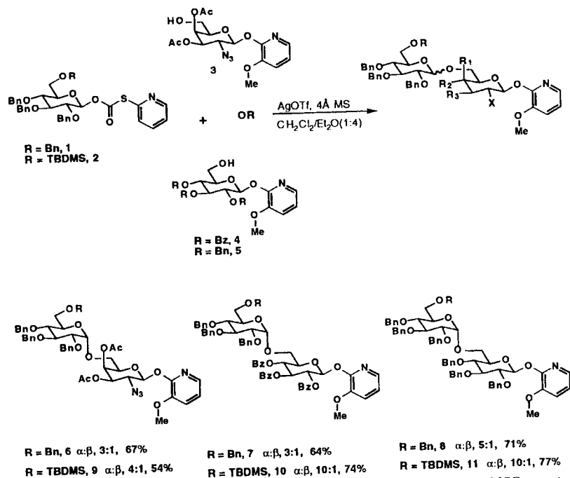
Scheme 3 Selective activation of TOPCAT glycosyl donors in the presence of MOP acceptors: TOPCAT versus MOP.
