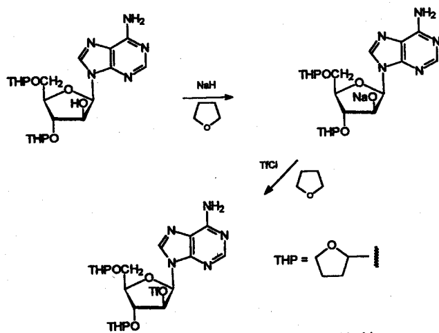
Scheme 2 Triflate formation with triflyl chloride.
