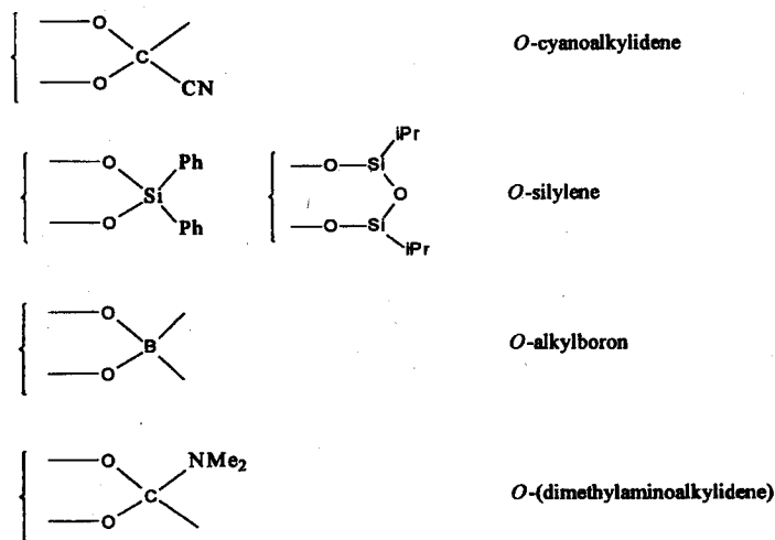
Chart 2 Derivatives related to acetals used in carbohydrate chemistry
