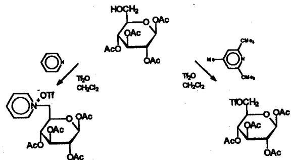
Scheme 1 Triflate reaction with pyridine.
