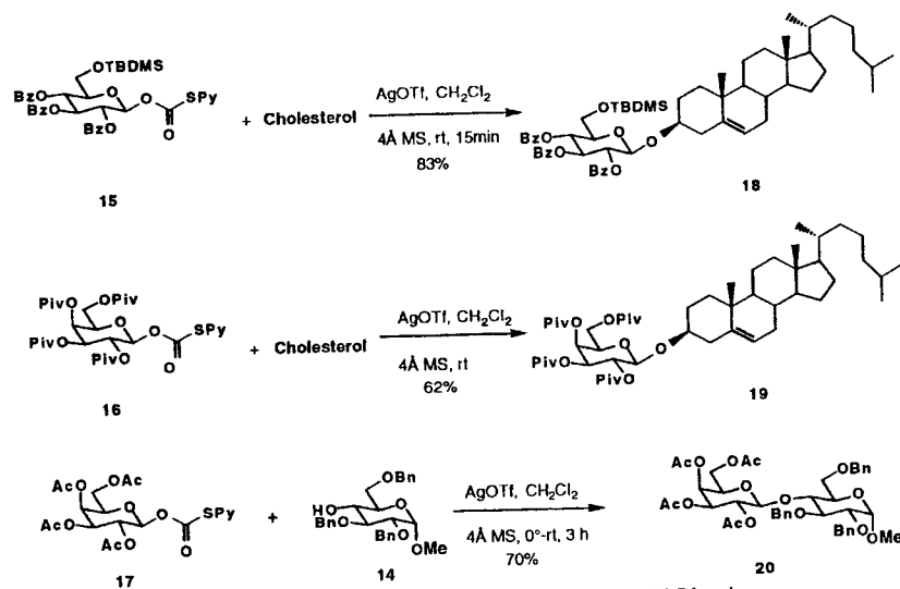
Scheme 5 1,2- trans -glycoside synthesis using the TOPCAT-leaving group.
