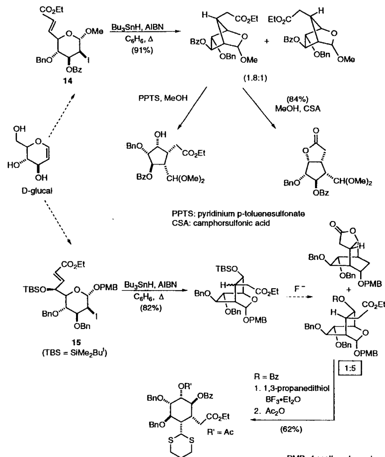
Scheme 7 Formation of bicyclic compounds via hex-5-enyl and hept-6-enyl radical cyclizations. 21
