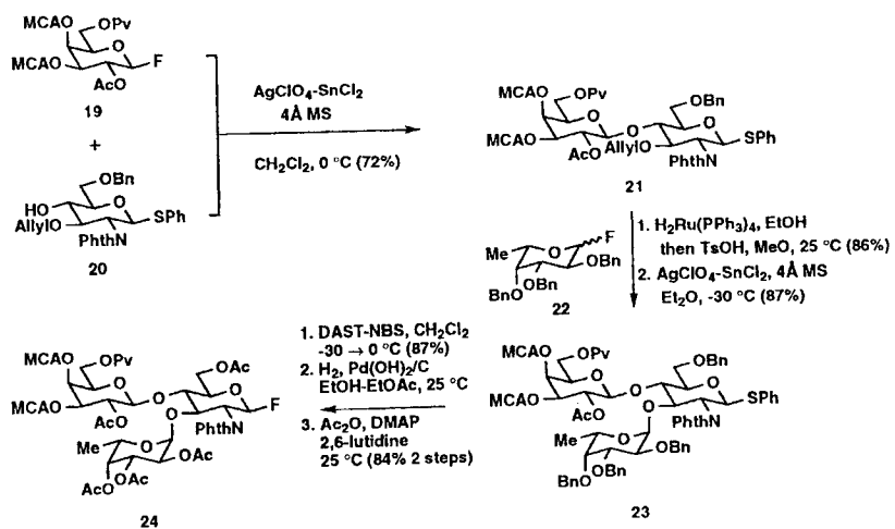
Scheme 13 Construction of the Le x fluoride 24 [47].
