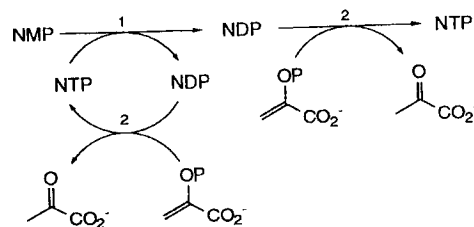
Figure 2 Synthesis of nucleoside triphosphates: (1) Adenylylation kinase (EC 2.7.4.3, N = A, C, U) or guanylate kinase (EC 2.7.4.8, N = G), or nucleoside monophosphate kinase (EC 2.7.4.4, N = U). (2) Pyruvate kinase (EC 2.7.1.40). NMP, nucleoside monophosphate; NDP, nucleoside diphosphate; NTP, nucleoside triphosphate. (From Ref. 12.)
