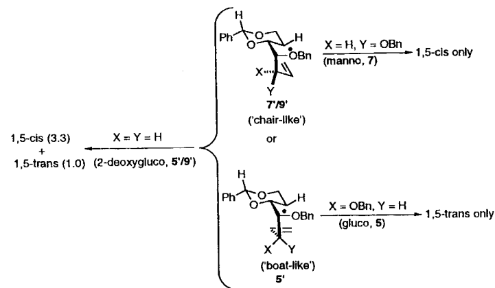
Scheme 4 Transition-state models for sugar hex-5-enyl radical cyclizations. 7
