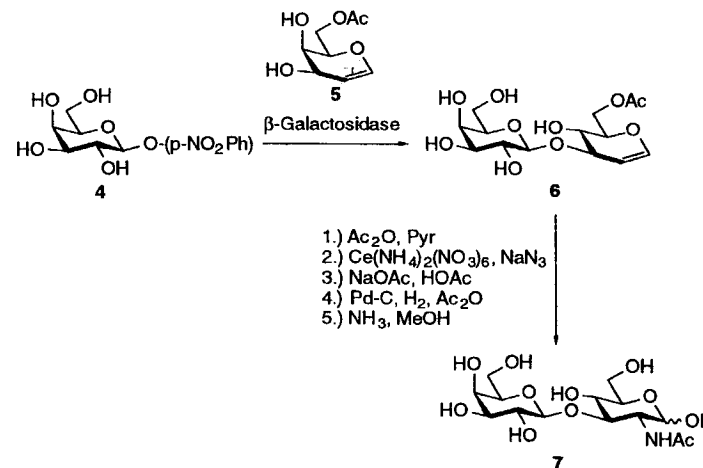
Figure 5 Synthesis of \beta 1,3-linked disaccharides. (From Ref. 34.)
