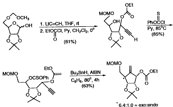
Scheme 5 Cyclization of a hex-5-ynyl radical. 16
