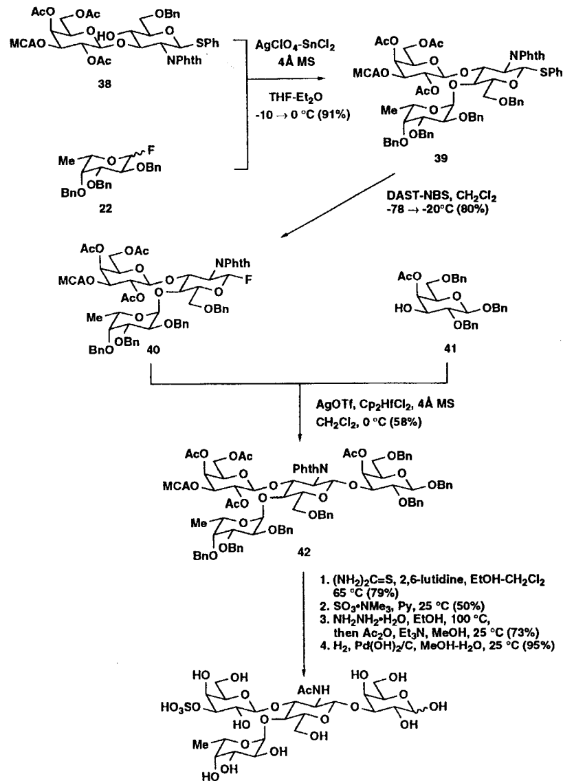
Scheme 16 Synthesis of sulfated Le^a tetrasaccharide 43 [48].
