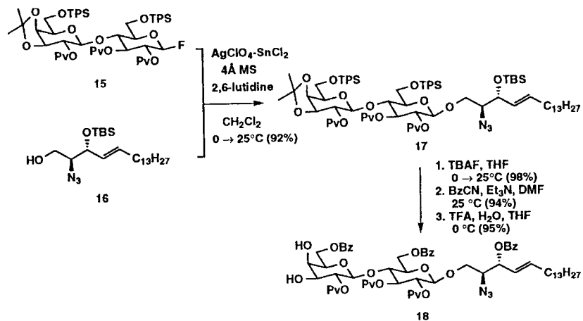
Scheme 12 Construction of Lactosyl Sphingosine Acceptor 18 (Ref. 47).
