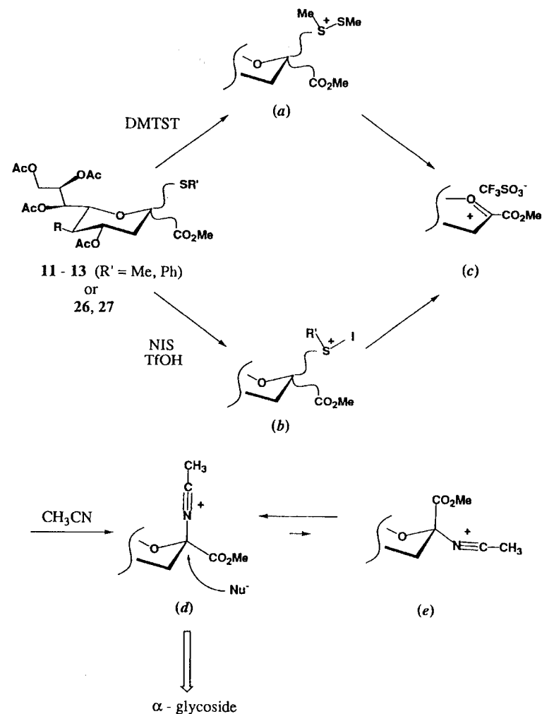
Figure 4 Reaction mechanism suggested for \alpha -predominant glycoside synthesis of sialic acids in acetonitrile.
