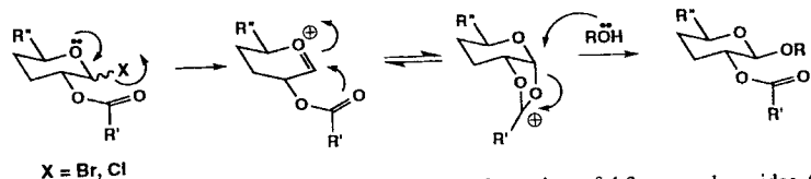
Scheme 2 Neighboring group participation in the formation of 1,2- trans -glycosides (often \beta -glycosides).
