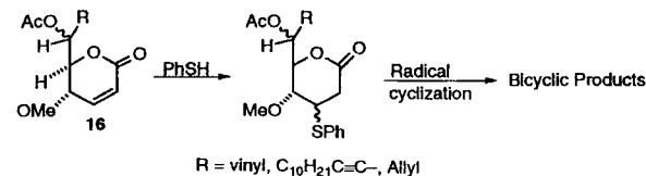
Scheme 8 Radicals from unsaturated sugar lactones. 22
