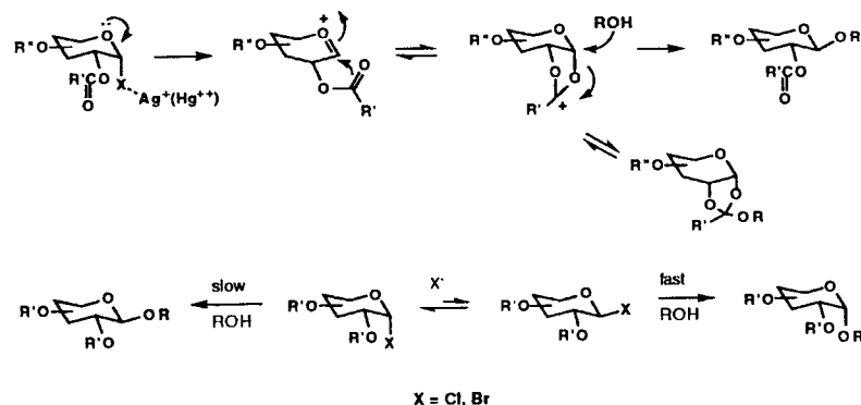
Scheme 1 1,2- trans -glycoside synthesis by Koenigs-Knorr-type glycosidations, and 1,2- cis -glycosides by the halide ion catalyzed method.
