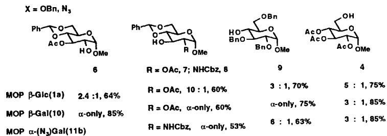
Scheme 5 Synthesis of 1,2- cis -glycosyl disaccharides using MOP glycosyl donors.
