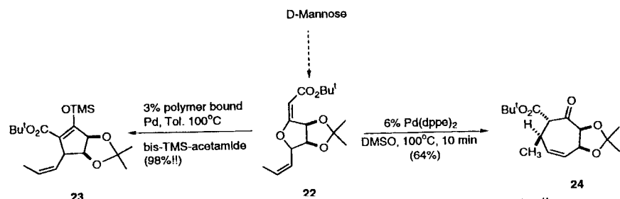
Scheme 10 Allyl palladium intermediates for the synthesis of carbocycles. 41
