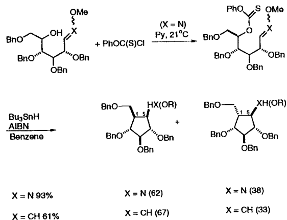
Scheme 6 Cyclization oxime and vinyl ether radicals 12,17
