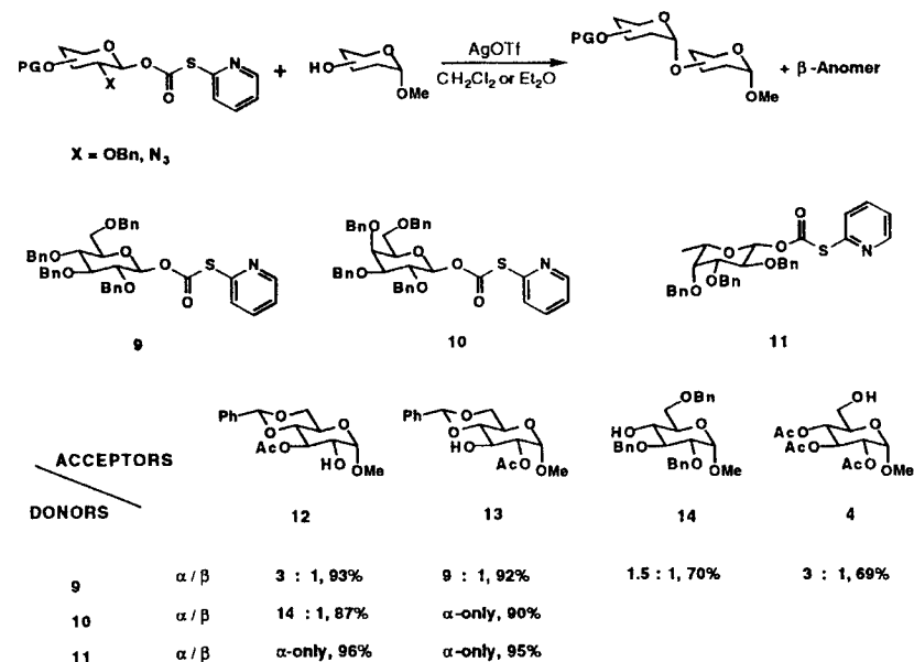
Scheme 4 Synthesis of 1,2- cis -disaccharides using TOPCAT glycosyl donors.
