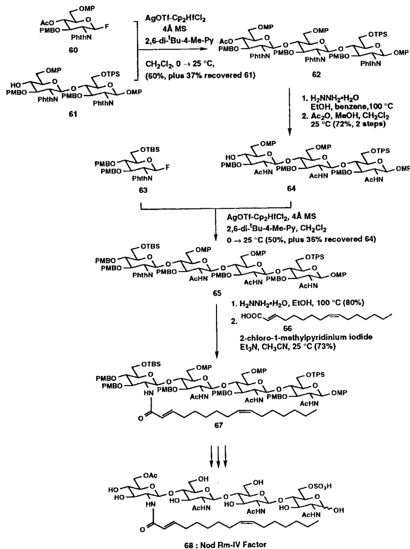
Scheme 19 Synthesis of NodRm-IV factor 68 [52].
