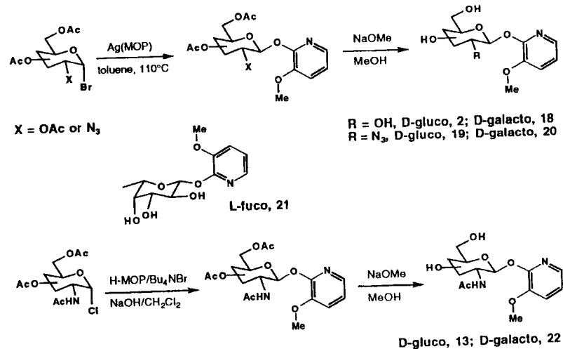
Scheme 5 Preparation of unprotected MOP-glycosyl donors.
