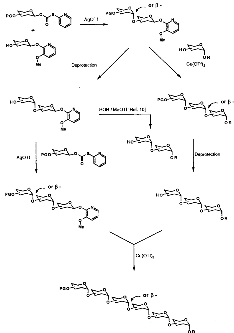
Scheme 2 Combination of TOPCAT and MOP activations.
