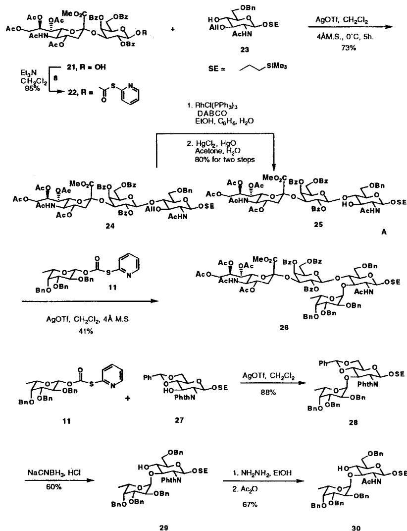
Scheme 6 Synthesis of a sialyl \text{Le}^x derivative and intermediate disaccharide by TOPCAT donors.
