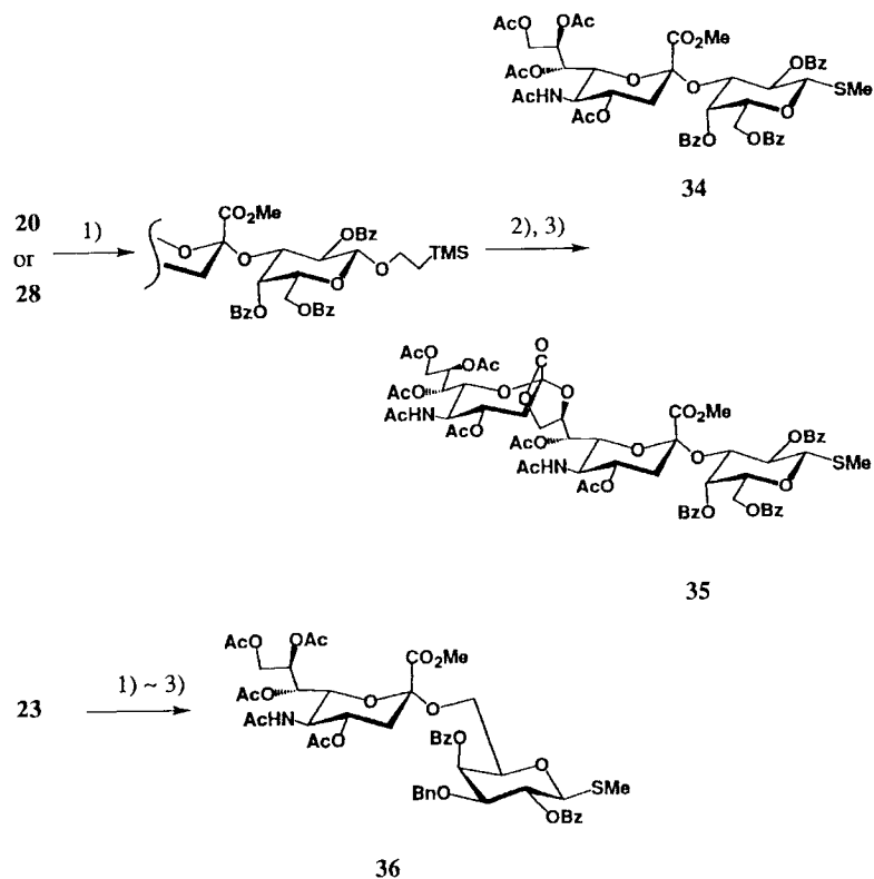
Figure 5 Mono- and oligo-sialyl galactose donors as building blocks. (1) Bz_2O , DMAP, Pyr., (2) Ac_2O , BF_3 \cdot OEt_2 , (3) TMSOTf, TMSOTf.
