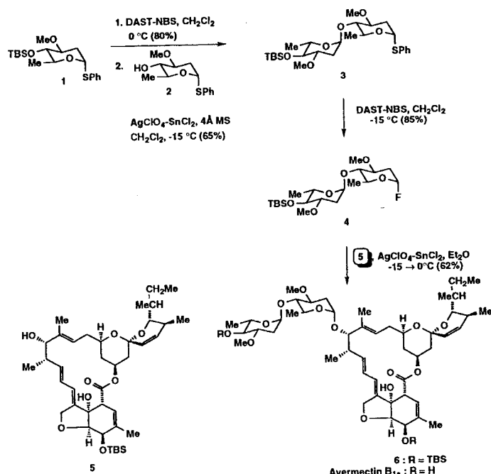
Scheme 10 Synthesis of avermectin \text{B}_{1a} [23].
