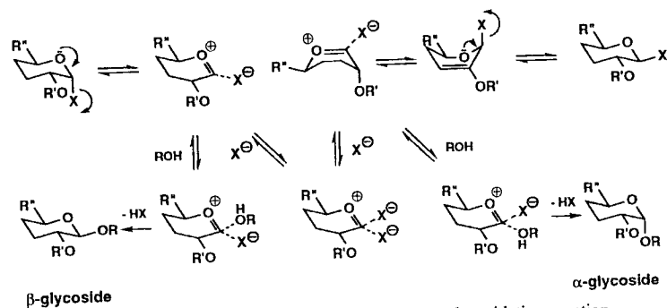
Scheme 1 Mechanism of the Koenigs-Knorr glycosidation reaction.
