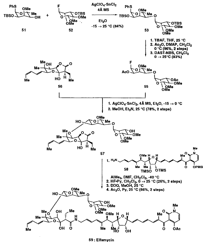
Scheme 18 Synthesis of elfamycin 59 [51].
