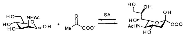
Scheme 3 Reversible aldol addition reaction catalyzed by sialic acid aldolase.
