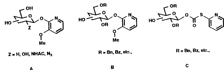
Scheme 4 MOP (A and B) and TOPCAT (C) glycosyl donors.
