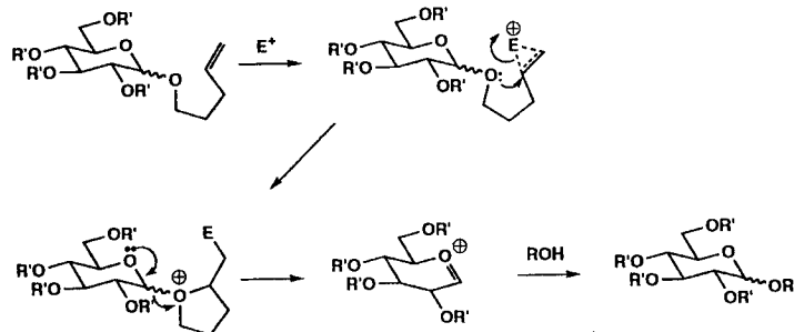
Scheme 5 The n -pentenyl glycoside-based glycosidation method, ( E^+ = I(\text{collidine})_2\text{ClO}_4 ) [17].
