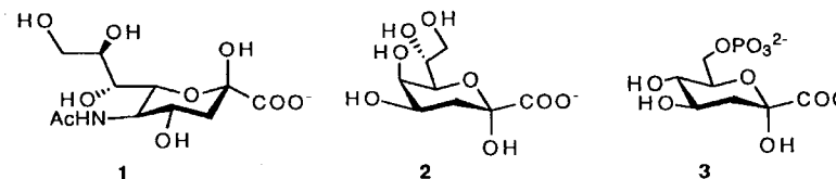
Scheme 2 The most important 3-deoxy-2-keto-ulosonic acids.
