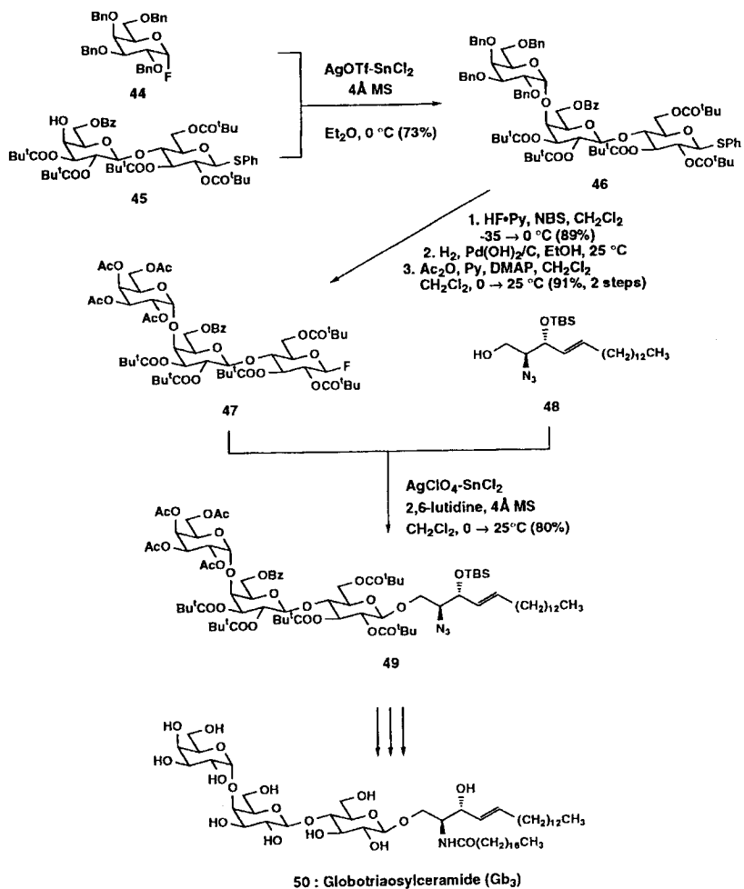
Scheme 17 Synthesis of globotriaosylceramide (Gb 3 ) 50 [50].
