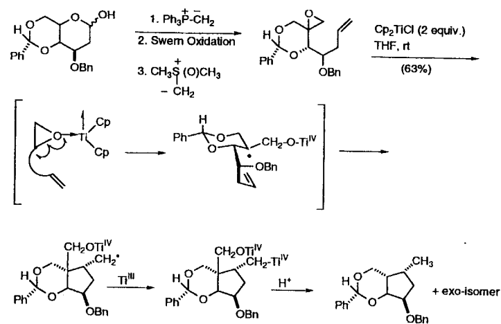
Scheme 9 Uses of a transition-metal centered radical for the cyclization of an epoxyolefin. 32
