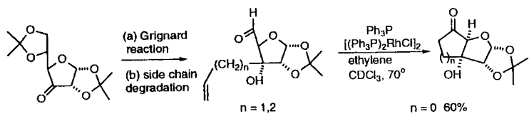
Scheme 13 Rh-catalyzed intramolecular hydroacylation route to carbocycles. 49
