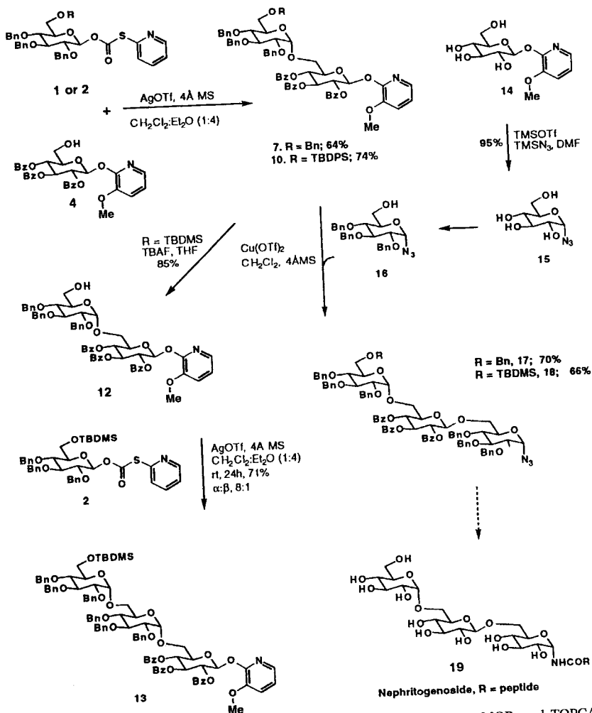
Scheme 4 Rapid and efficient iterative oligosaccharide assembly using MOP- and TOPCAT-leaving groups.
