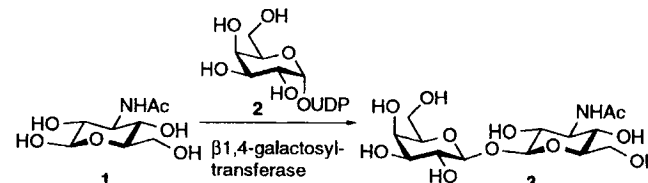
Figure 3 Synthesis of a \beta , \beta -1,1-linked disaccharide with galactosyltransferase. (From Ref. 17.)
