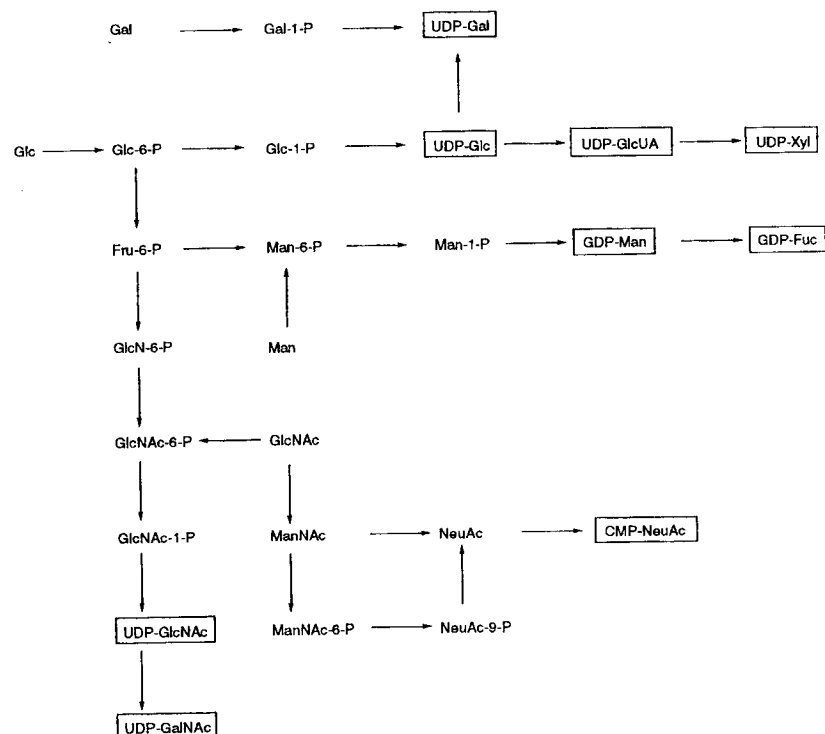
Figure 1 Biosynthesis of sugar nucleotides. (From Ref. 12.)
