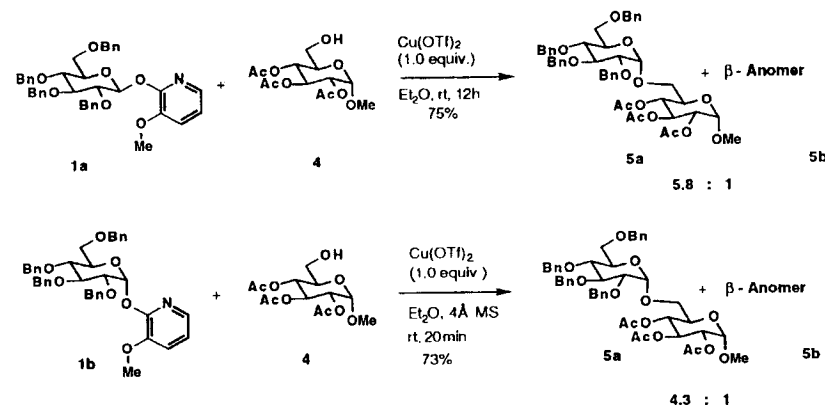
Scheme 4 Disaccharide synthesis with O -benzyl MOP glycosyl donors using Cu(OTf) 2 as promoter.
