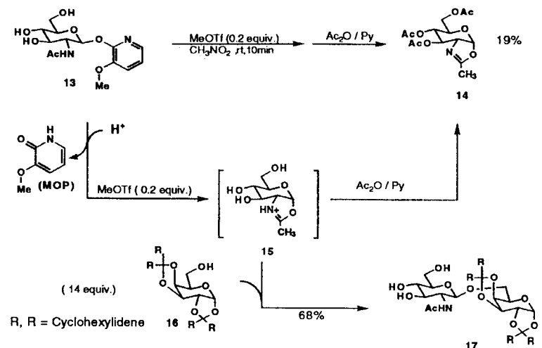
Scheme 3 1,2- trans -Glycoside synthesis using an unprotected MOP glycosyl donor containing a 2-acetamido group.
