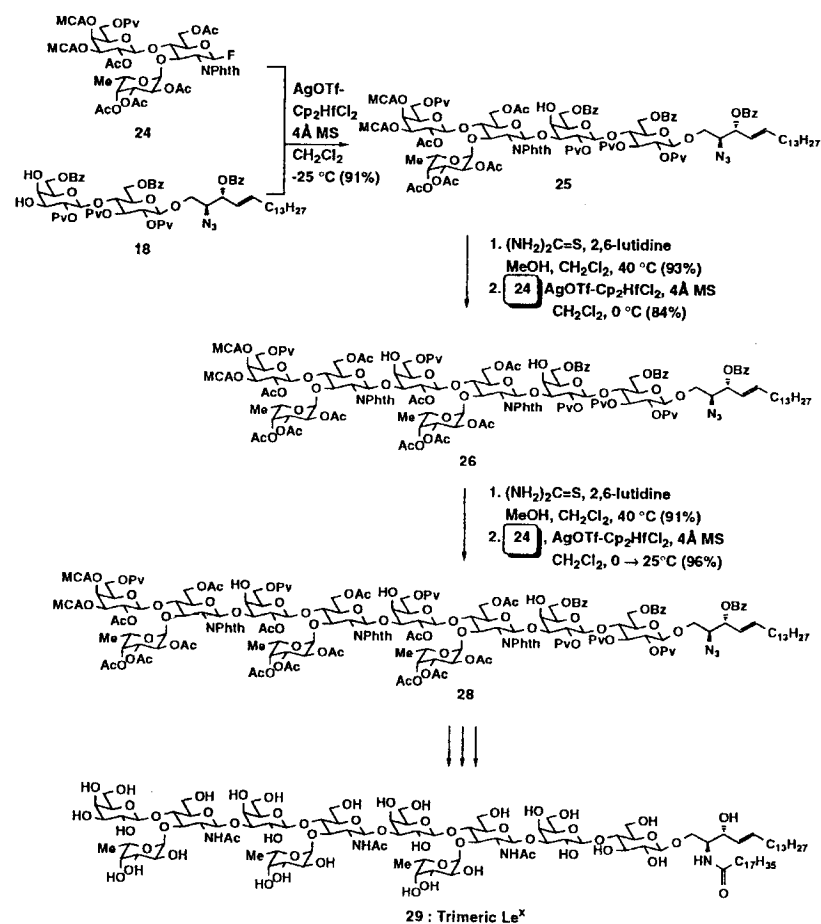
Scheme 14 Synthesis of trimeric Le x 29 [48].
