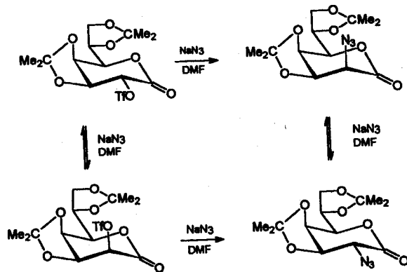
Scheme 5 Epimerization by azide ion.
