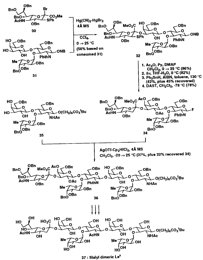
Scheme 15 Synthesis of sialyl dimeric Le^x 37 [48].
