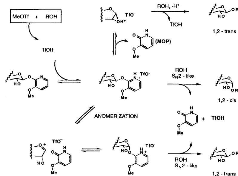
Scheme 4 Possible mechanistic pathways.
