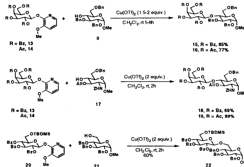
Scheme 7 1,2- trans -Disaccharide synthesis using MOP-leaving group.
