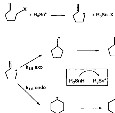
Scheme 1 Hex-5-enyl Radical Cyclization at 60°C, k_{1,5} = 10^5\text{--}10^6 \text{ s}^{-1} ; k_{1,5}/k_{1,6} = 50 .
