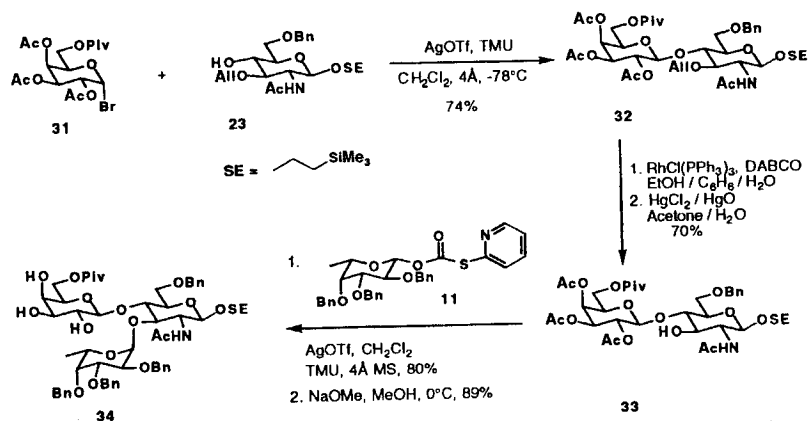
Scheme 7 Synthesis of Le x trisaccharide derivative via TOPCAT-mediated glycosylation.
