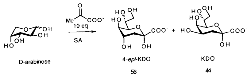
Scheme 4 Lack of stereoselectivity observed in the sialic acid aldolase-catalyzed addition of pyruvate with D-arabinose.
