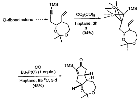
Scheme 11 An application of the Pauson–Khand reaction. 44a
