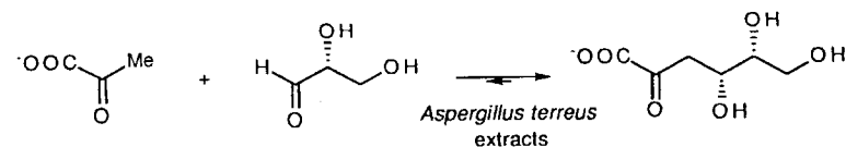
Scheme 8 Reversible aldol addition reaction catalyzed by Aspergillus terreus KDGal aldolase.
