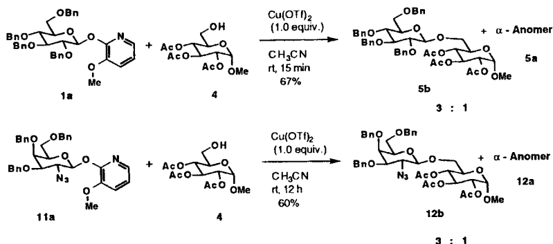
Scheme 6 1,2- trans -Disaccharide synthesis using CH 3 CN as solvent.
