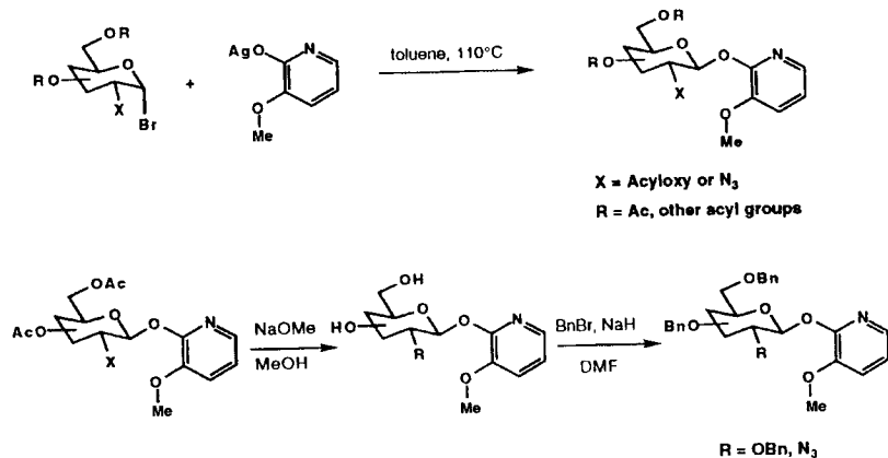
Scheme 2 Preparation of O -protected MOP glycosyl donors.
