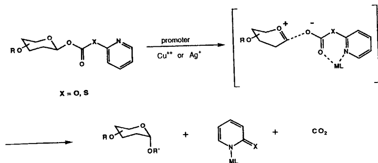
Scheme 1 The design of glycosyl 2-pyridylcarbonate or glycosyl 2-thiopyridylcarbonate (TOP-CAT) donors based on the remote activation concept.
