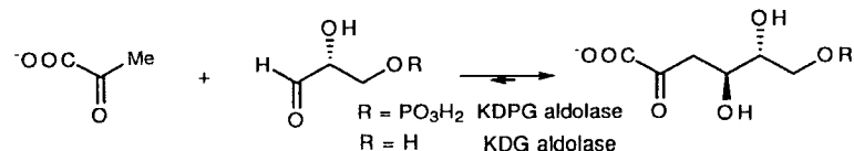
Scheme 7 Reversible aldol addition reaction catalyzed by KDPG and KDG aldolases.
