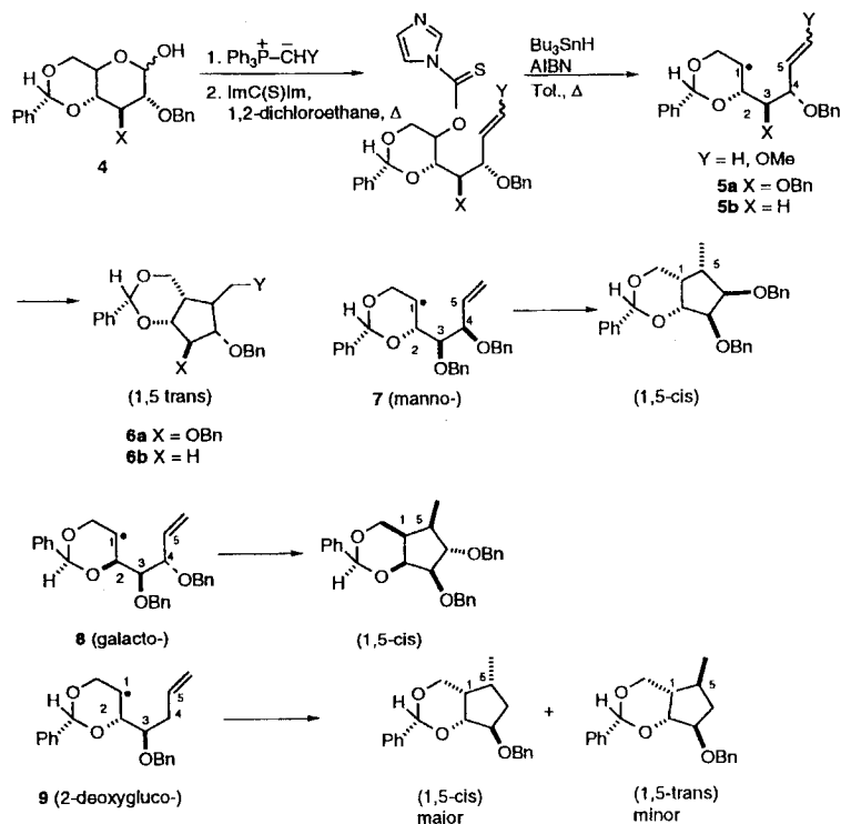
Scheme 3 1,2-Dialkylcyclopentanes from hexopyranose sugars. 12
