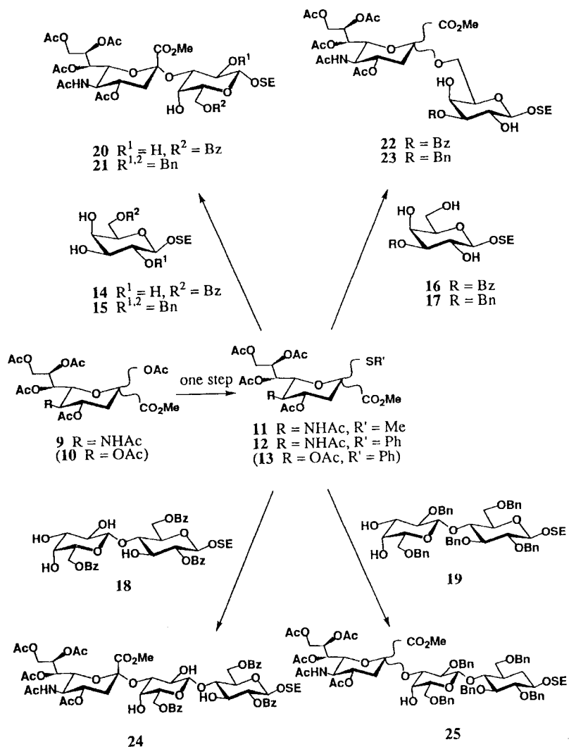
Figure 2 An efficient regio- and \alpha -stereoselective synthesis of mono-sialyl glycosides. (SE = -\text{CH}_2\text{CH}_2\text{SiMe}_3 .)
