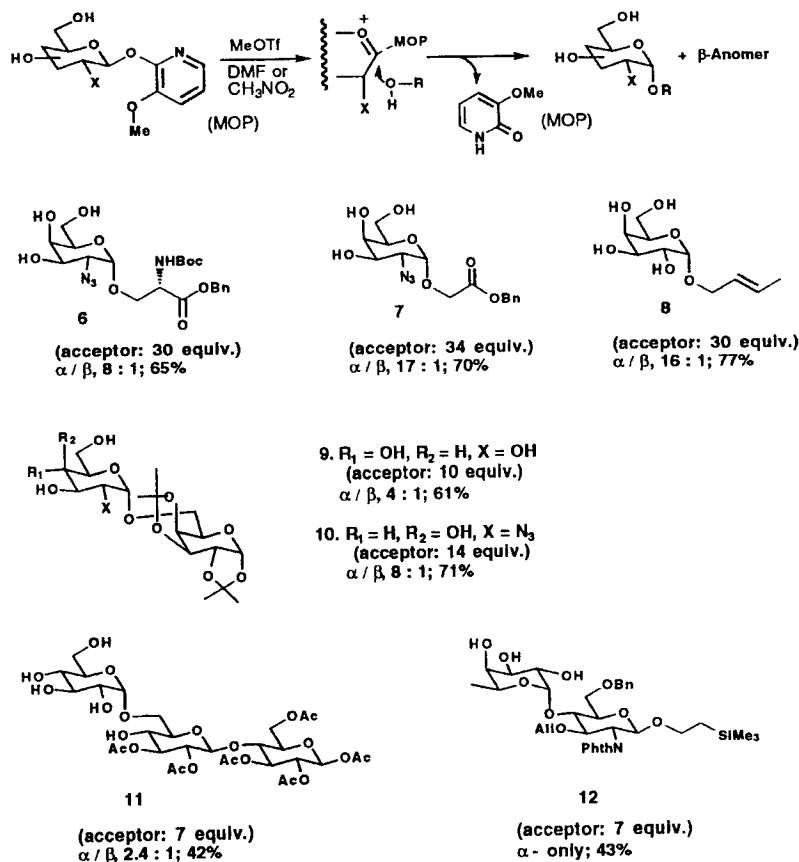
Scheme 2 Synthesis of 1,2- cis glycosides with unprotected MOP-glycosyl donors.
