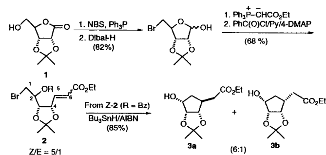
Scheme 2 Carbocyclic compounds from furanose sugars.
