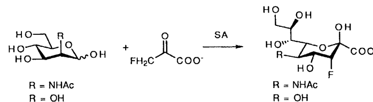
Scheme 5 Aldol addition of fluoropyruvate with N-acetylmannosamine or mannose catalyzed by sialic acid aldolase.
