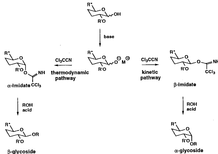
Scheme 3 The preparation of trichloroacetimidates and their glycosidation reaction [10].
