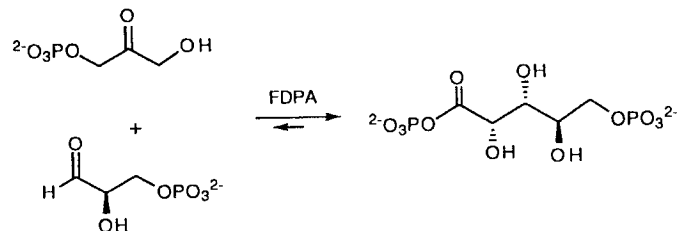
Scheme 1 Reversible aldol addition reaction catalyzed by fructose diphosphate aldolase.
