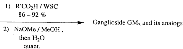
Figure 6 A synthetic route to ganglioside GM_3 .
