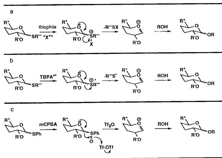
Scheme 8 Thioglycoside-based glycosidation reactions. (a) thiophile = N -bromosuccinimide (NBS) [35], methyl triflate [38], dimethyl(methylthio)sulfonium triflate (DMTST) [39], or N -iodosuccinimide (NIS)-triflic acid [40]. (b) \text{TBPA}^+ = tris(4-bromophenyl)ammonium hexachloroantimonate [42]. (c) mCPBA = m -chloroperbenzoic acid [43].
