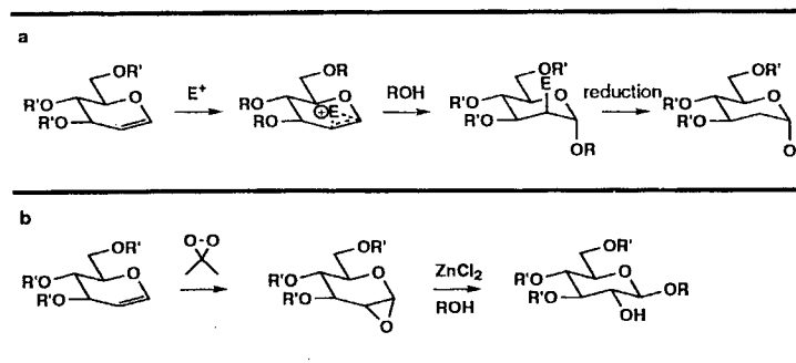
Scheme 4 Glycal-based glycosidation reactions. (a) E^+ = I(\text{collidine})_2\text{ClO}_4 [11], N -iodosuccinimide [12], \text{PhSeCl} [13], \text{PhSCl} [14]. (b) Danishefsky method [15].
