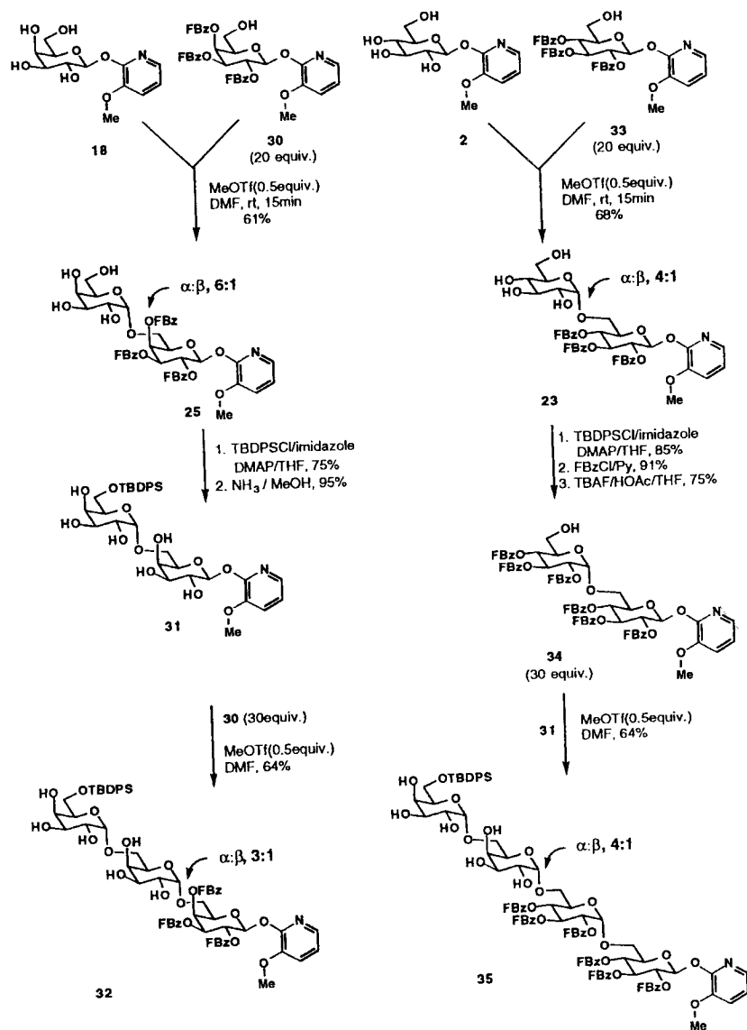
Scheme 7 Iterative oligosaccharide synthesis.
