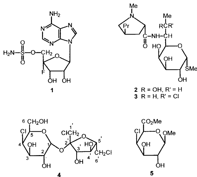
Figure 1 Structure of some biologically important derivatives of deoxyhalogeno sugars.
