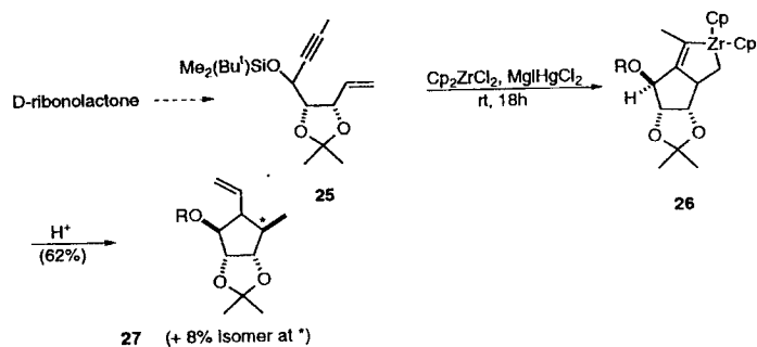
Scheme 12 Low-valent zirconium-mediated cyclization of eneynes. 45
