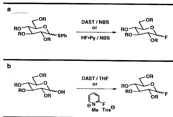
Scheme 7 Methods for glycosyl fluorides using (a) thioglycosides [23] and (b) lactols [29,30].
