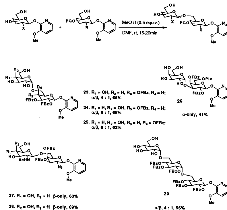
Scheme 6 Selective activation; unprotected MOP donors versus protected MOP glycosides.
