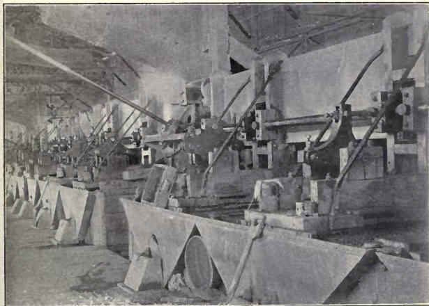
DIAMOND PULSATOR, DE BEERS DIAMOND MINE AT KIMBERLEY, SOUTH AFRICA
