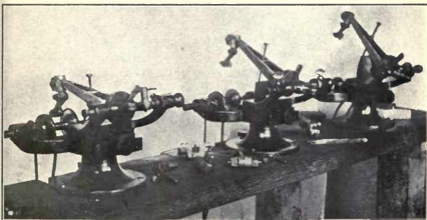
DIAMOND SAWING MACHINES
