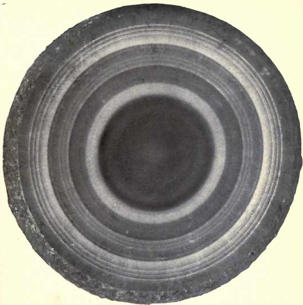
AGATE WITH CONCENTRIC RINGS
