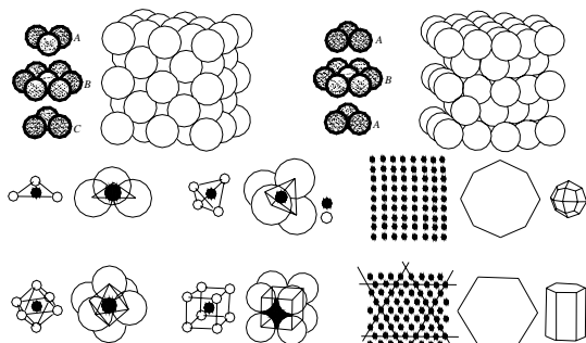
coordination of crystal structures
