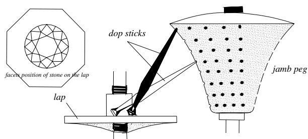
diamond polishing device or jamb peg
