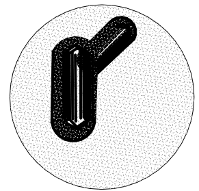
olivine crystals in diamond. ca. 2000x
