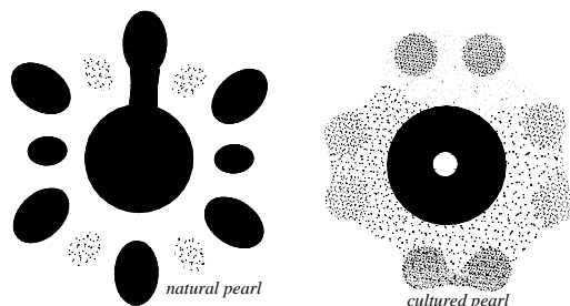
X-ray Laue-gram of natural and cultured pearl
