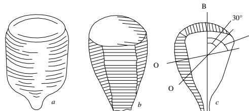
a: synthetic ruby boule, b: cut a part of boule and c: cross section of synthetic ruby boule with axes and angles
