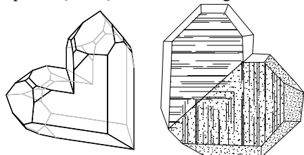
Japanese law twins of quartz
