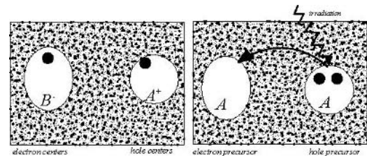
electron and hole centers in crystal. After Nassau 1963
