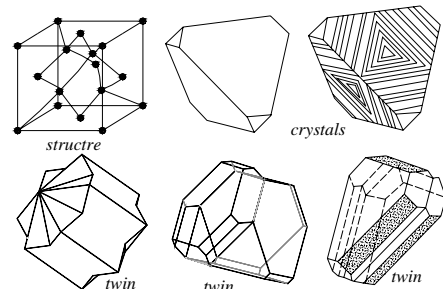
sphalerite structure, crystals and twins
