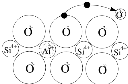
smoky quartz and irradiation. After Nassau 1983
