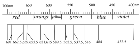
zircon absorption spectrum
