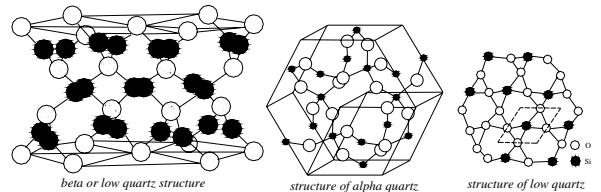
quartz crystal structures
