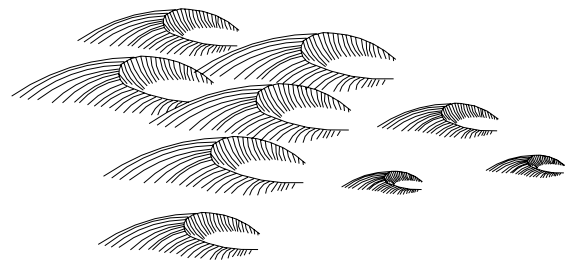
barchan of sand dune
