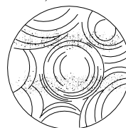
perlite of obsidian
