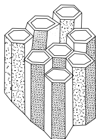
columnar structure of basalt
