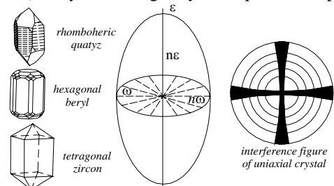
an ellipsoidal sketch of an uniaxial crystal with two different refractive indices, n_o and n_e
