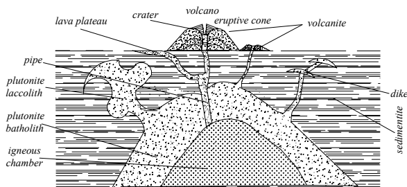
forms of igneous activity
