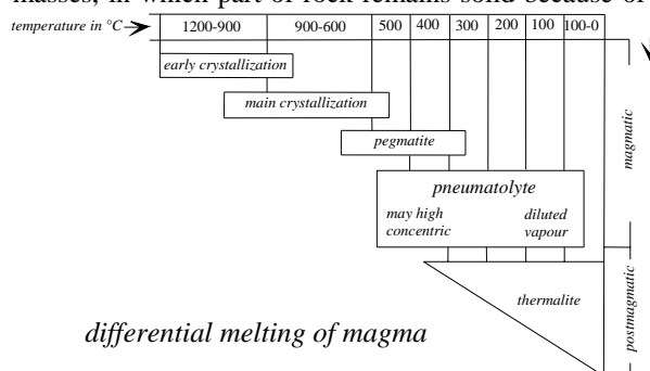
differential melting of magma
