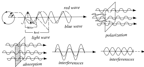
light wave, polarization, absorption and interferences
