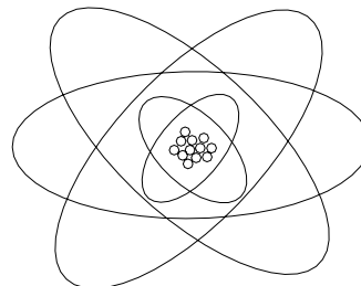
carbon-12 structure and surrounding negative electrons orbitals the nucleous
