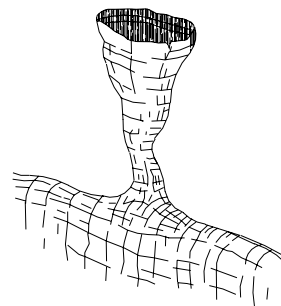
Kimberlite volcano pipe. After Cloos, H. 1936
