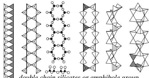
double chain silicates or amphibole group of inosilicate (\text{Si}_4\text{O}_{11})^{6-}
