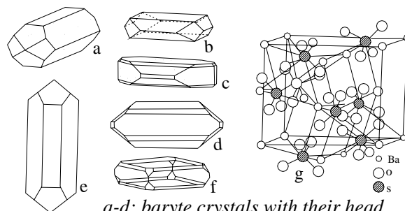
a-d: baryte crystals with their head forms and f: crystal structure
