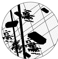
zircon needles in labradorite from Labrador
