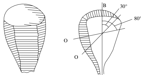
left: a synthetic ruby boule. Right: cross section through a ruby boule. O: optical axis. B: boule axis
