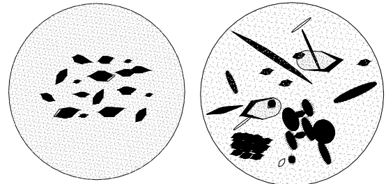
biotite scales in peridot and emerald
