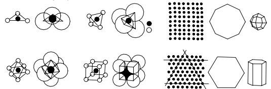
coordination of crystal structures
