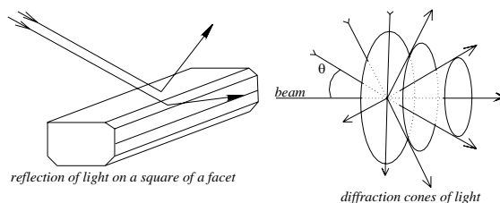
reflection of light on facets and conical effect
