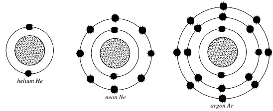
electronic configuration of inert atoms
