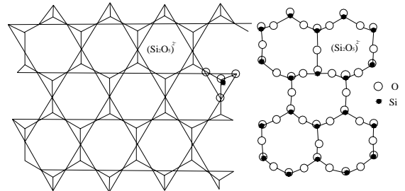
phyllosilicate structure, hexagonals are tetrahedron of (\text{SiO}_3)^{2-}
