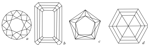
crown of different cuts, a: round-brilliant crown, b: emerald-cut crown, c: five rayed star-cut crown and d: hexagon-cut crown
