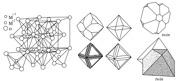
spinel structure, crystals and twins
