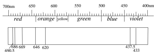
spodumene absorption spectrum
