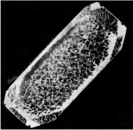
Figure 15.10 A synthetic hydrothermally grown quartz crystal showing the characteristic pebbly surface which is never seen in natural quartz
