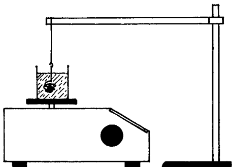
Figure 7.6 An alternative single-pan method of hydrostatic weighing uses an independent suspension of the specimen to measure the downthrust produced by its displacement of water
