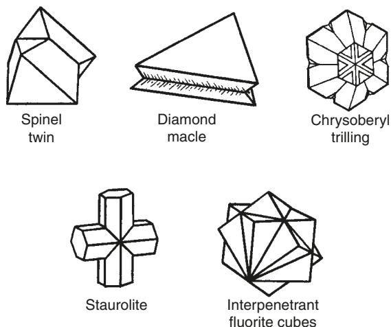
Figure 4.15 Top: three examples of contact twins. Bottom: two examples of interpenetrant twins
