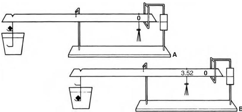
Figure 7.8 A direct-reading SG balance. Two gemstone holders are provided at the left end of the beam for the in-air and in-water weighings (the lower one is immersed in the beaker of water during both weighings). The counterweight is set to the '0' mark for the in-air weighing and is loaded (by means of hook-on weights) for balance equilibrium (A). For the in-water weighing, the counterweight is moved to the left to restore equilibrium (B), its new position on the scale indicating the gemstone's SG. (Hanneman)
