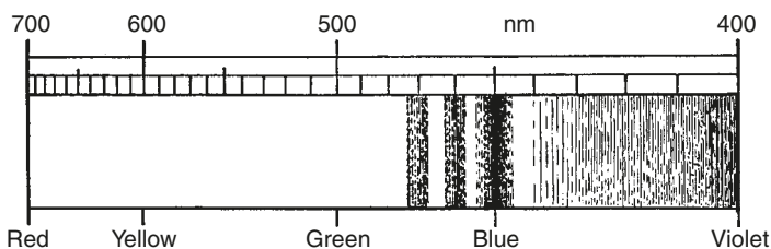
Figure 8.4 An absorption spectrum showing three bands (caused by iron) which are diagnostic for blue sapphire
