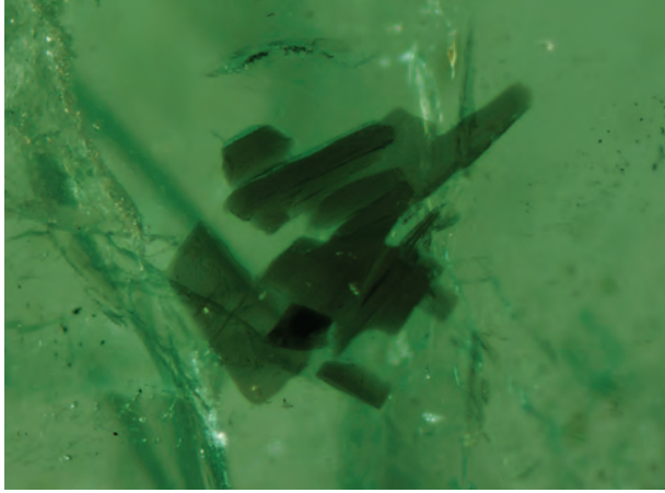
Figure 27. Platelets of phlogopite, as seen here in one of the Chantete emeralds, are quite common inclusions in Zambian emeralds. Photomicrograph by H. Zwaan; magnified 80 \times .
