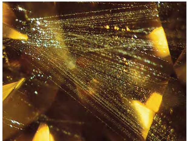
Figure 12. Stringers of numerous tiny inclusions, some in reflective orientation, create an interesting cloud formation in this brownish yellow diamond. The presence of this cloud further supports the diamond’s natural-color determination. Photomicrograph by John I. Koivula; magnified 30x.
