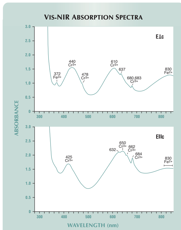
Figure 39. These polarized absorption spectra of an emerald from the Chantete mine show bands that are representative of all the Kafubu samples, and indicate the presence of not only \text{Cr}^{3+} and \text{Fe}^{2+} , but also \text{Fe}^{3+} . The intensities of the bands varied somewhat between samples, but no straightforward relationship could be established between band intensities and Cr and Fe concentrations (or \text{FeO}/\text{Cr}_2\text{O}_3 ratios) measured by electron microprobe. The spectra shown here were collected on a 4.27 ct emerald cut that contained an average of 0.17 wt. % \text{Cr}_2\text{O}_3 and 0.36 wt. % \text{FeO}^{\text{tot}} .
