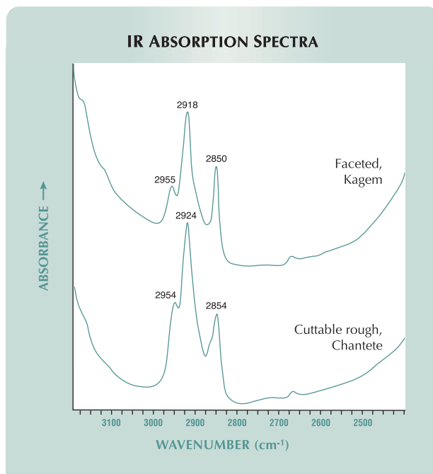
Figure 41. Peaks in the 3100–2800 \text{cm}^{-1} range were seen in the FTIR spectra of both faceted and cuttable rough specimens of Kafubu emerald, indicating the presence of oil. No artificial resin was found in the stones that were tested. Spectra have been offset vertically for clarity.
