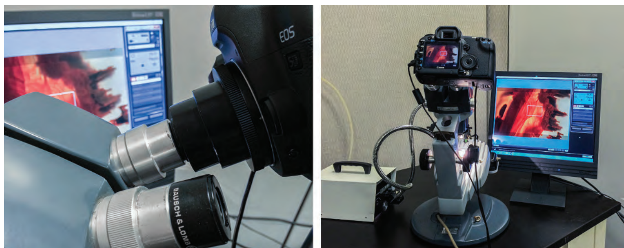
Figure 5. Left: A camera adapter that slips over the microscope's ocular can turn a binocular microscope into a photomicroscope, as seen on the author's GIA Gemolite Mark V. Right: A live view shown on a computer monitor is used for focusing and composition because the oculars are blocked by the camera. The camera is remotely controlled by the software, which helps prevent vibration-induced blurring that would occur by manually pressing the shutter button. Photos by Nathan Renfro.
