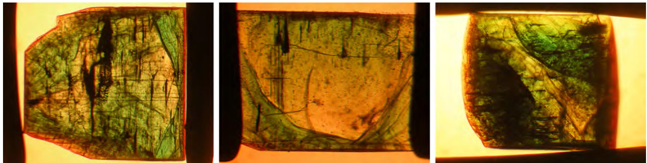
Figure 8. The type 2 synthetic emeralds grown from molybdenum- and vanadium-bearing fluxes are less heavily included. They also show colorless seeds with fluid inclusions (flat cavities) oriented parallel to the basal face. Immersion, field of view 4.6 × 3.4 mm (left), 3.5 × 2.6 mm (center), and 3.8 × 2.8 mm (right). Photomicrographs by K. Schmetzer.
