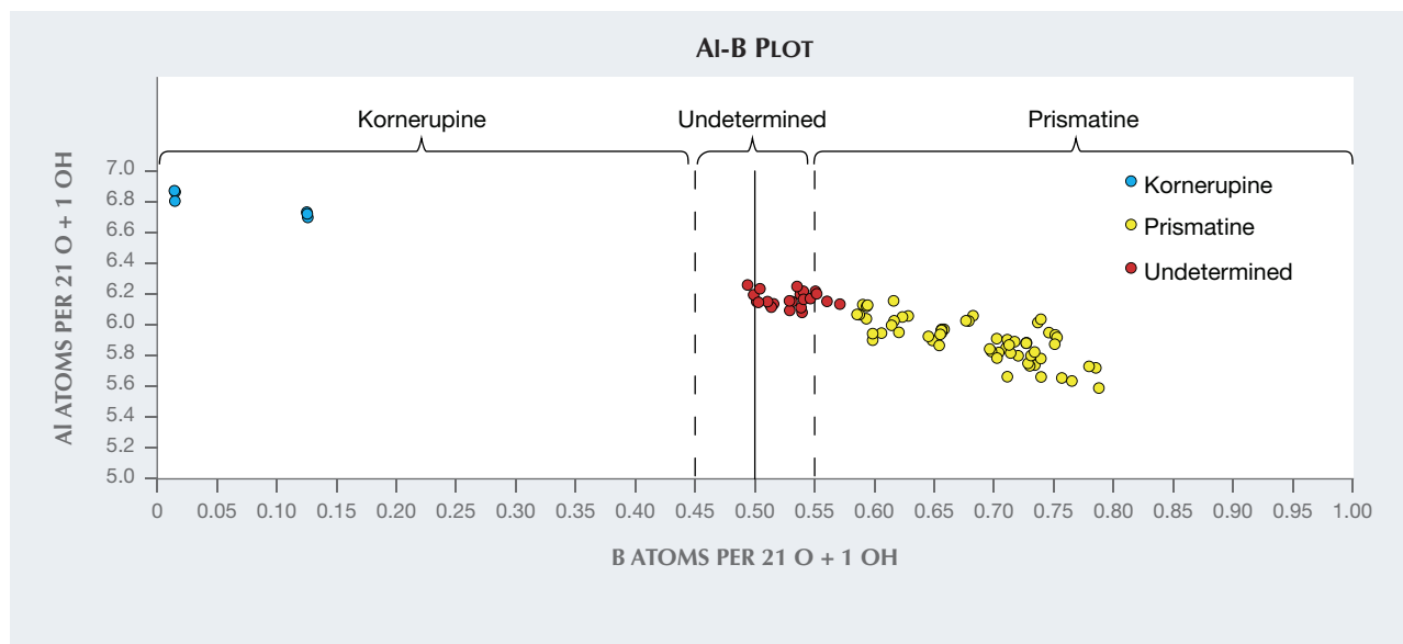
Figure 8. The AI-B plot shows three sections. When the B (apfu) is between 0 and 0.45, stones are classified as kornerupine (blue spots). When the B (apfu) is between 0.45 and 0.55, the species for the stones (red spots) cannot be determined. When the B (apfu) is between 0.55 and 1.00, stones (yellow spots) are classified as prismaticine. For three spot analyses, if one spot has a B (apfu) between 0.45 and 0.55, the species is considered undetermined.
