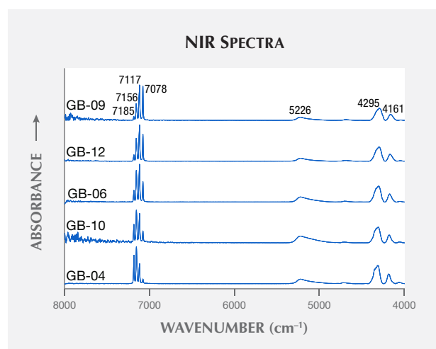
Figure 9. Near-infrared spectra of five typical thin-section samples (0.73–0.97 mm thick) from Guangxi showing bands related to the first overtone of M_3\text{-OH} asymmetry stretching modes as well as the combination modes of water, M_3\text{-OH} , and Si-O groups of actinolite or ferro-actinolite in the 8000–4000 \text{cm}^{-1} range. Spectra are offset vertically for clarity.
