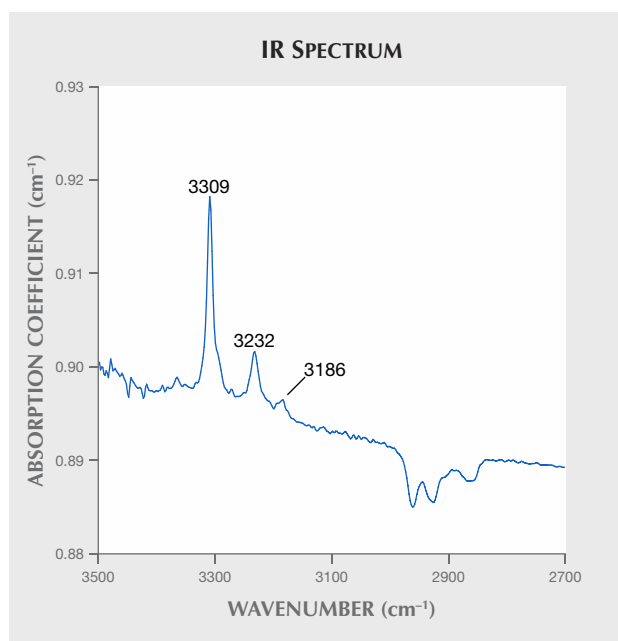
Figure 15. After heating to 1300°C, sample 2 developed a strong 3309 \text{cm}^{-1} series with peaks at 3309, 3232, and 3186 \text{cm}^{-1} . In sapphires (and rubies) that have formed in metamorphic environments, the presence of the 3309 peak is not diagnostic; it is the appearance of the 3232 peak that provides strong evidence of artificial heat treatment.
