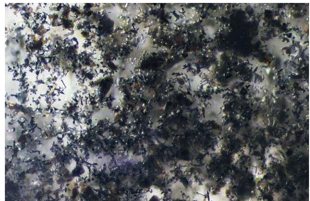
Figure 14. The black appearance of a topaz was due to these small dark mineral inclusions. Photomicrograph by Jonathan Muyal; field of view 1.44 mm.
