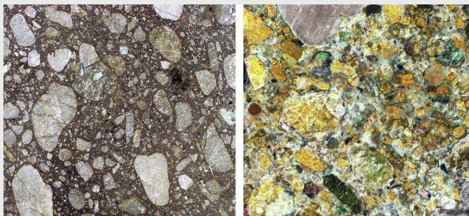
Figure A-1. Images of kimberlite textures. Left: Hypabyssal kimberlite from the Grizzly 3 kimberlite, Canada (field of view 7.62 cm). Right: Volcaniclastic kimberlite from the Victor North kimberlite, Canada (field of view 7.62 cm). Photos by Steve Shirey.
