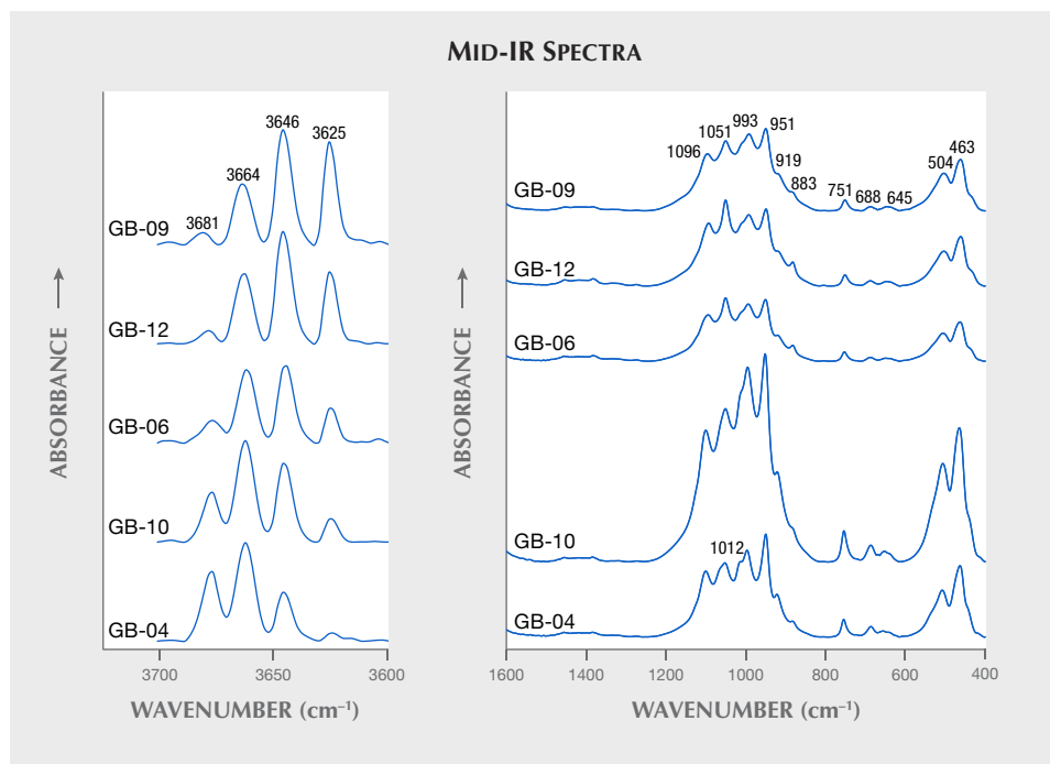
Figure 8. Mid-infrared spectra of five typical plate samples from Guangxi in the 3700–3600 \text{cm}^{-1} (left) and 1600–400 \text{cm}^{-1} (right) ranges. The spectra show bands related to M_3\text{-OH} asymmetric stretching modes; Si-O-Si, O-Si-O, and M-O stretching modes; Si-O bending modes; and O-H translational modes of actinolite or ferro-actinolite. (M is an abbreviation for a metal ion.) Spectra are offset vertically for clarity.
