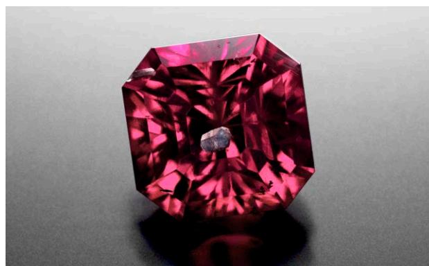
Figure 1. This 5.33 ct red pyrope-spessartine garnet was faceted by the author to display the unusual blue apatite crystal within. Photo by Diego Sanchez.
