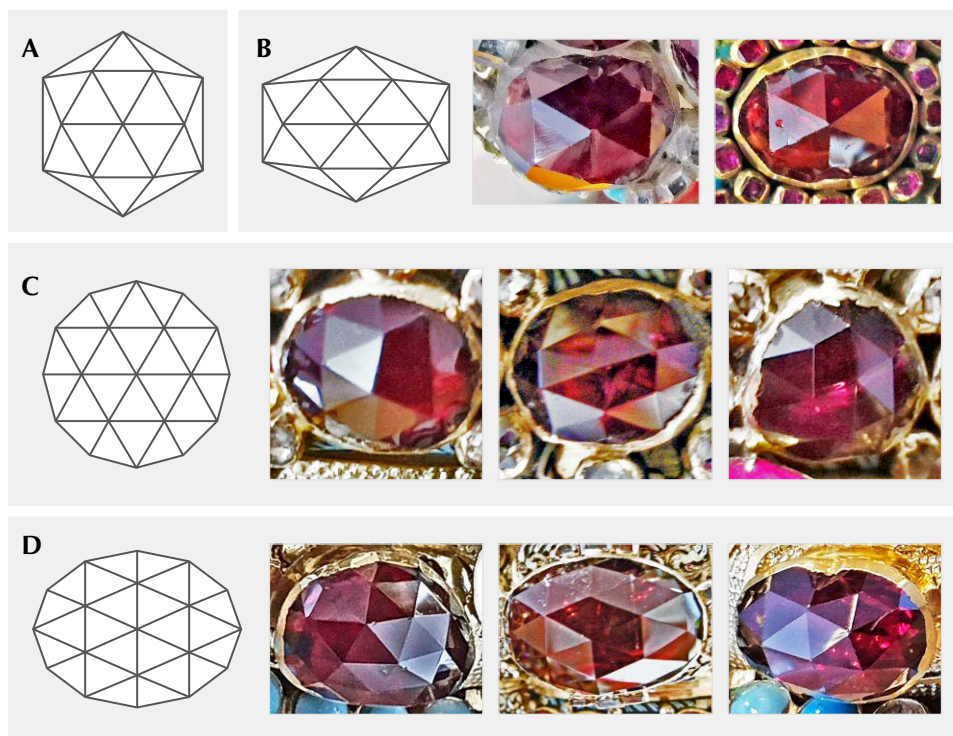
Figure 17. Group 2 garnets with half-Dutch (A, B) and full-Dutch rose cuts (C, D) from the Limburg and Cologne insignia displayed outlines approximating round, almost round to slightly oval (A, C) or oval (B, D). B: Both 15 \times 11 mm. C (left to right): 8 \times 7 mm, 8 \times 7 mm, and 7 \times 7 mm. D (left to right): 20 \times 16.5 mm, 30 \times 21 mm, and 9 \times 7 mm. Drawings and photos by K. Schmetzer.
