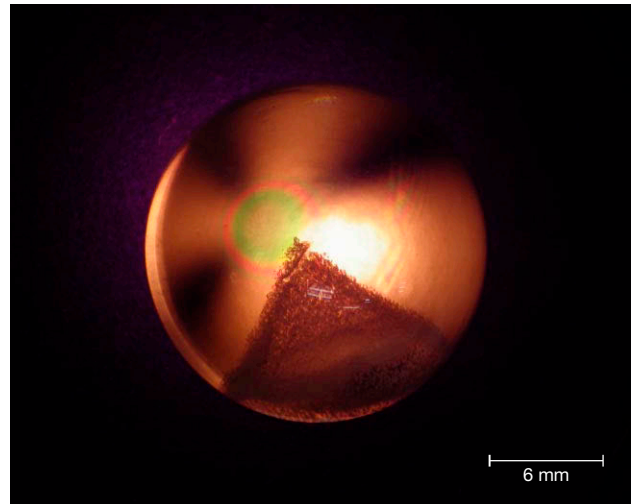
Figure 15. Crossed polarizers revealed that the bull's eye, indicating the optic axis, was nearly perpendicular to the axis of the engraved “phantom.” Photo by Shu-Hong Lin.
