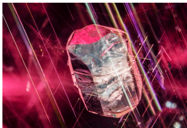
Figure 2. A blue apatite crystal associated with intersecting iridescent needles was showcased. Photomicrograph by Jessa Rizzo; field of view 2.90 mm.
