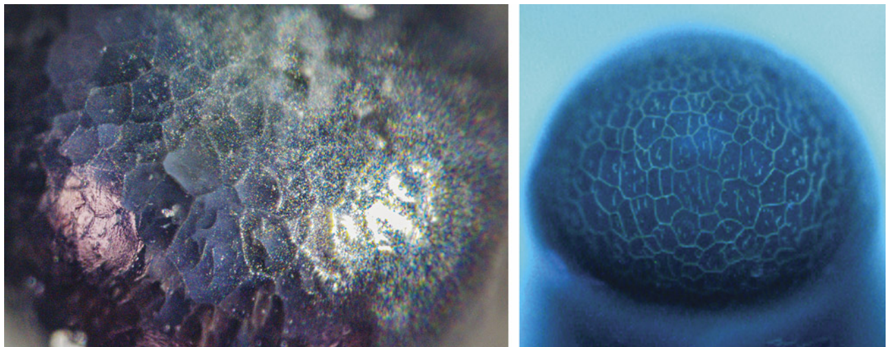
Figure 20. Left: Non-nacreous surface of the black pearl; field of view 3.4 mm. Right: DiamondView image showing a bluish reaction of the outline of the cellular structure. Photos by Anukul Belanke.
