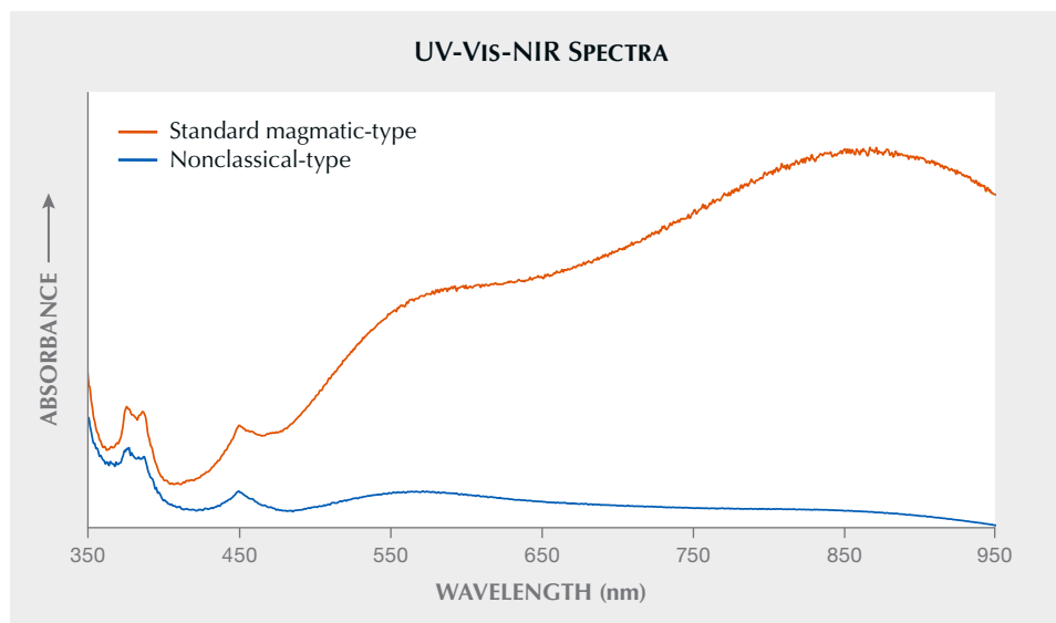
Figure 30. Representative UV-Vis-NIR spectra of Matepwende sapphire. Half of the samples showed a standard magmatic-type UV-Vis-NIR spectrum with a prominent 880 nm band and Fe 3+ -related features, while the other half showed a nonclassical spectrum without a prominent 880 nm band but with prominent Fe 3+ -related features.
