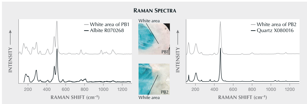
Figure 18. Raman spectra of the white matrix in the two “Paraíba matrix” samples, with standard RRUFF reference spectra included for comparison. Spectra are offset vertically for clarity.
