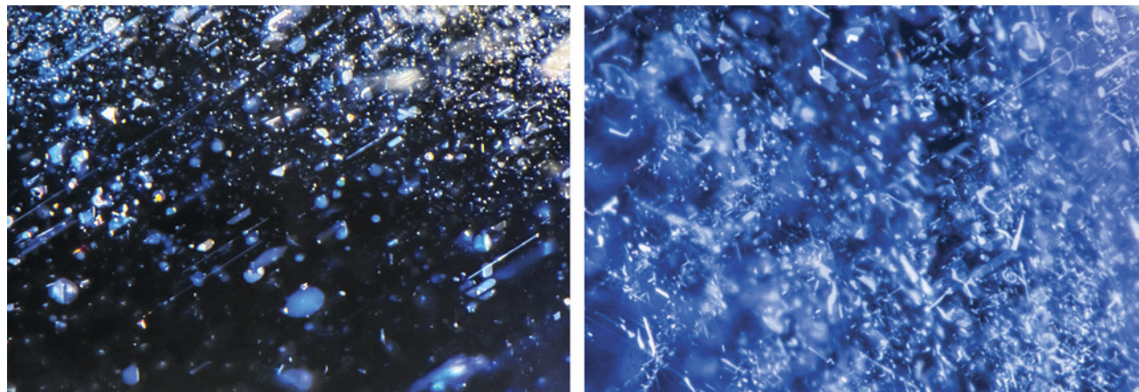
Figure 31. Platelet-type inclusions (left) and reflective silk (right) in the Matepwende sapphires with a magmatic-type UV-Vis-NIR spectrum. Photomicrographs by Aaron Palke; fields of view 1.58 mm (left) and 1.26 mm (right).
