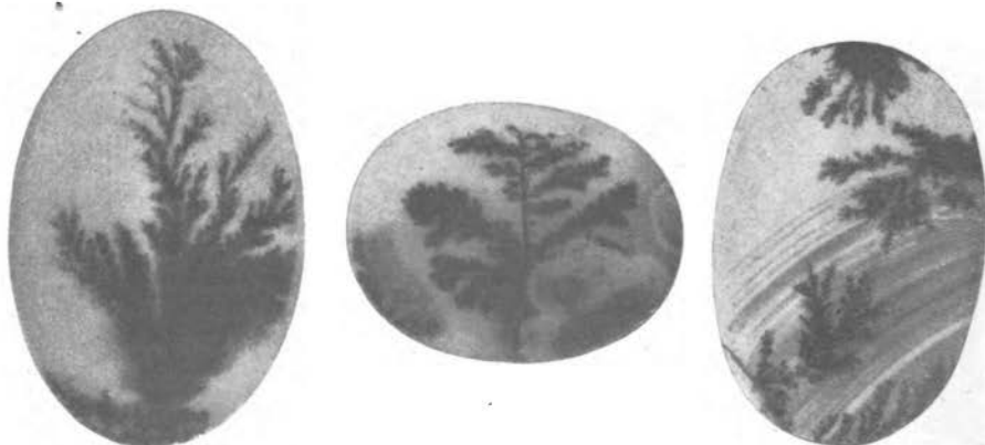
FIG. 3.—MOSS AGATES.
