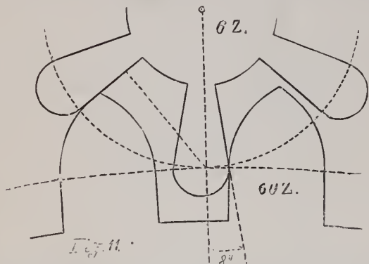
Figs. 11 to 14.—The teeth have the altered curve, the fullness of the tooth is larger than the space.
