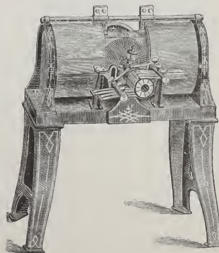
FIG. 2.—The Mather Dynamo-Electric Machine.
