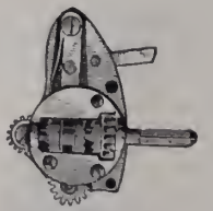
For HOWARD 16 & 18 Size Watches.
